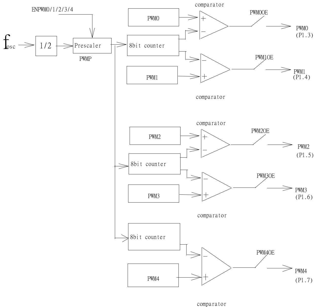
Figure 1 PWM diagram
