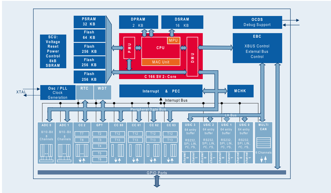
Block Diagram XC2267M
