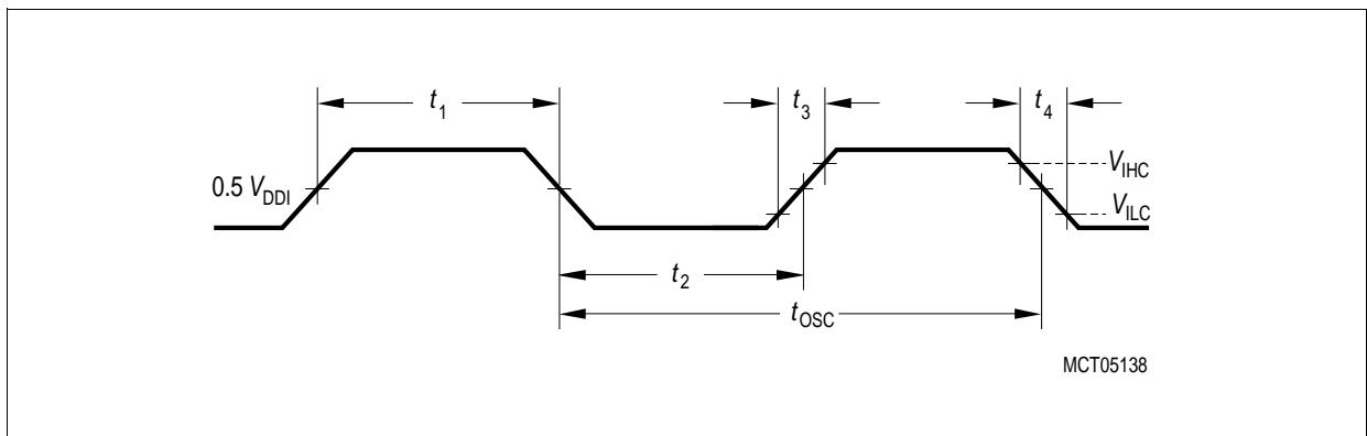
Figure 16 External Clock Drive XTAL1
