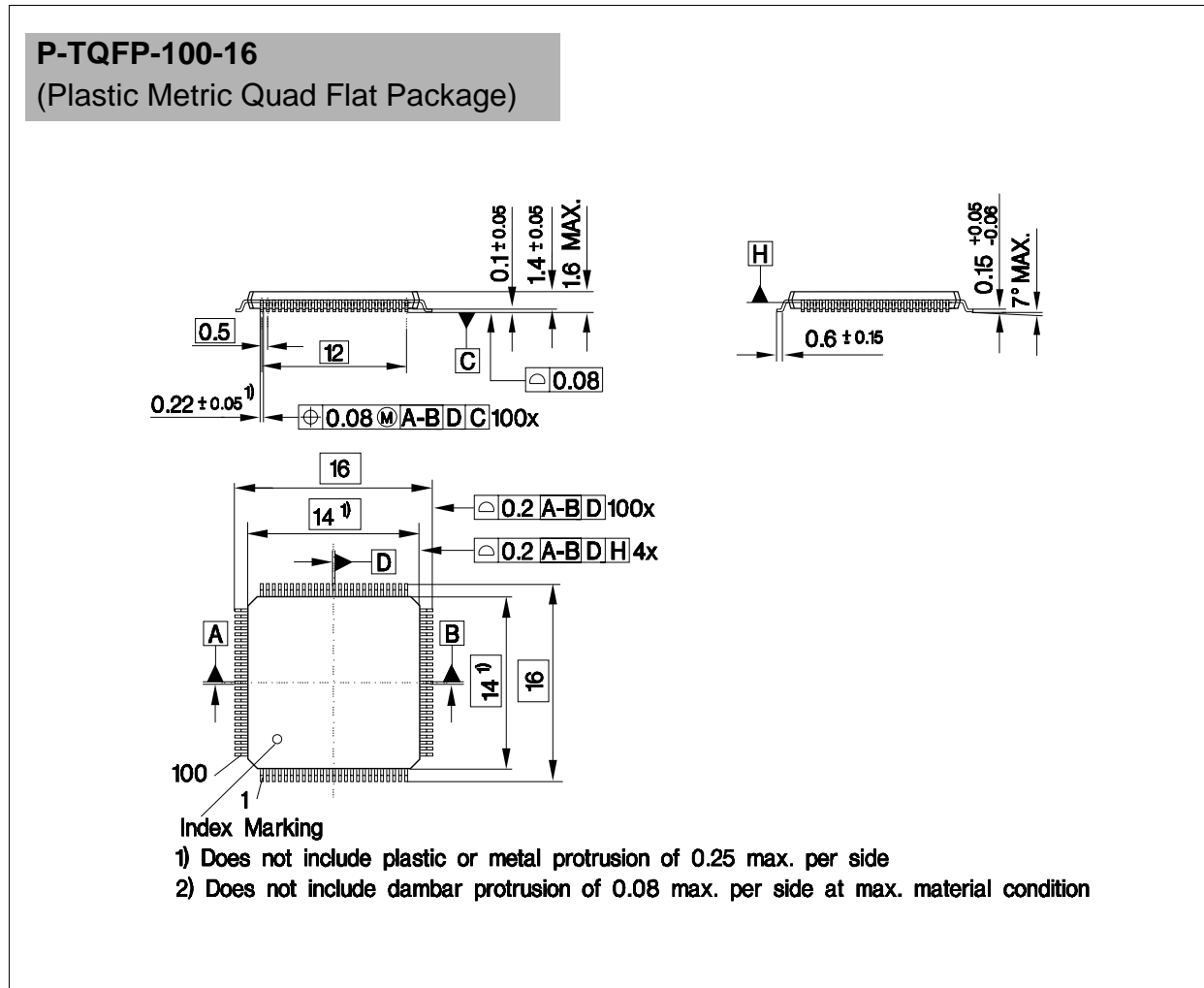
Figure 22 Package Outlines P-TQFP-100-16
