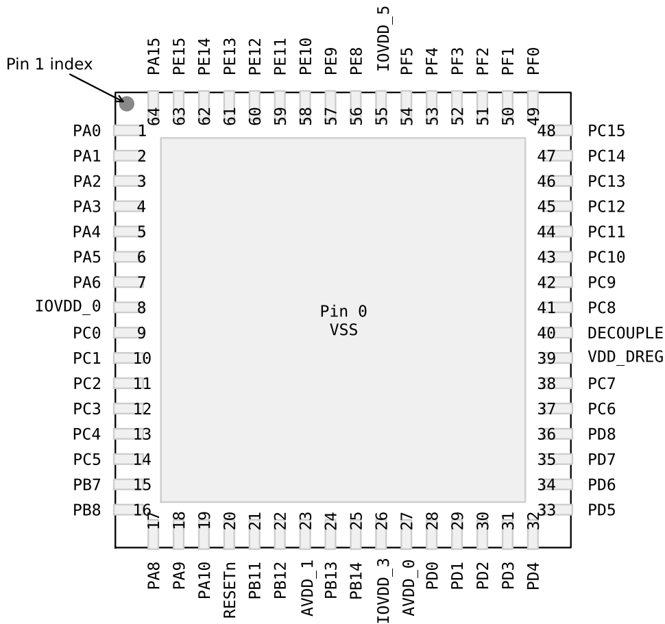
Figure 4.1. EFM32TG230 Pinout (top view, not to scale)
