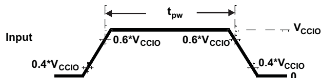
Figure 5-13. FlexRay Inputs
