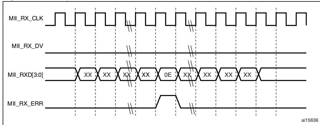
Figure 331. Reception with false carrier indication
