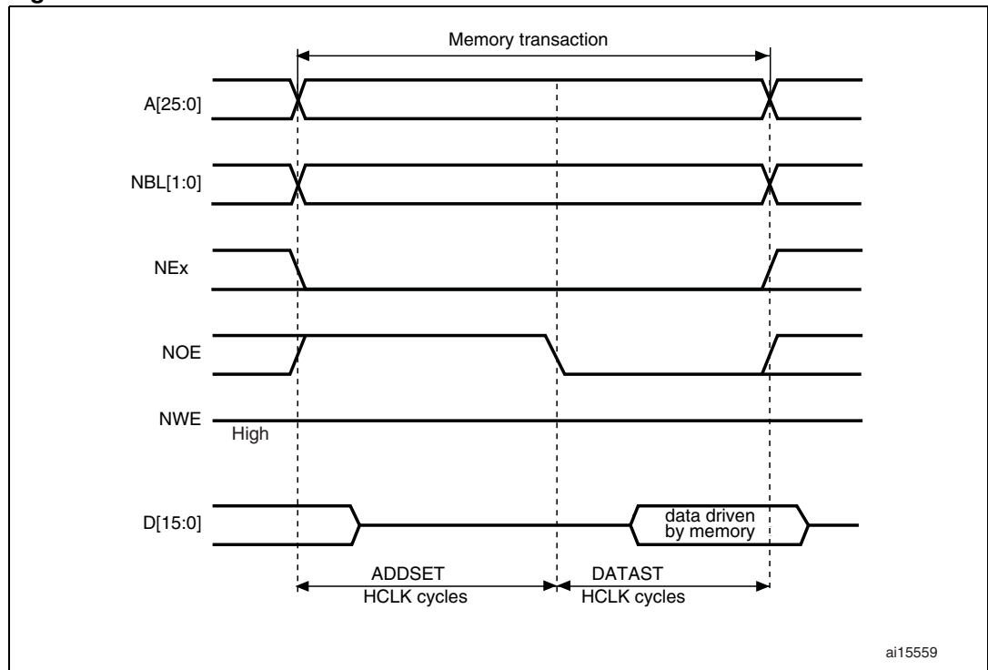
Figure 398. ModeA read accesses
