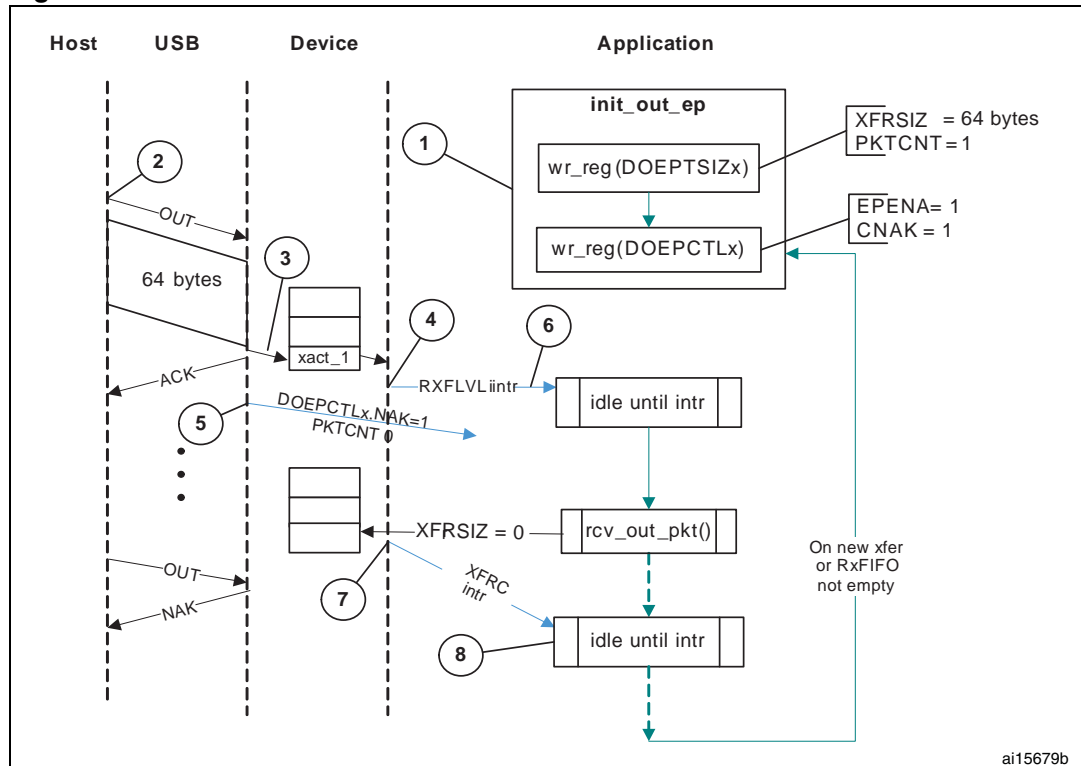
Figure 366. Bulk OUT transaction
