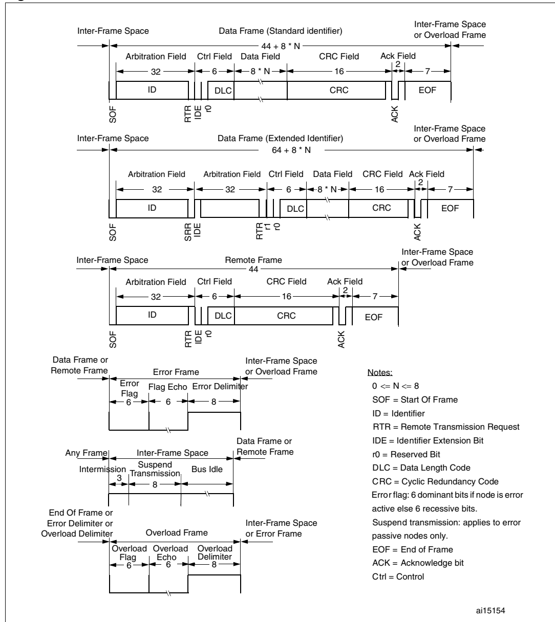
Figure 310. CAN frames
