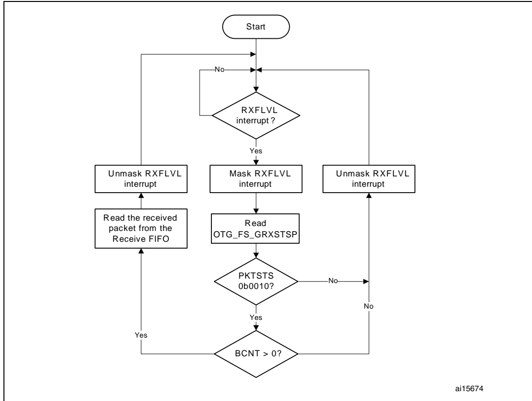
Figure 359. Receive FIFO read task
