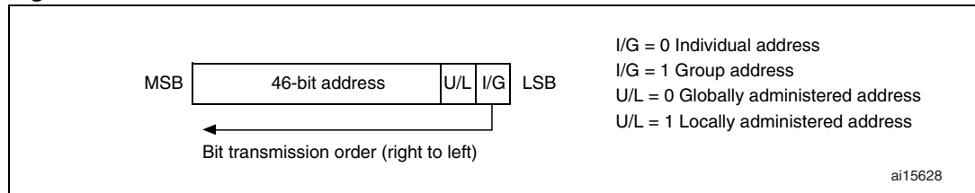
Figure 321. Address field format
