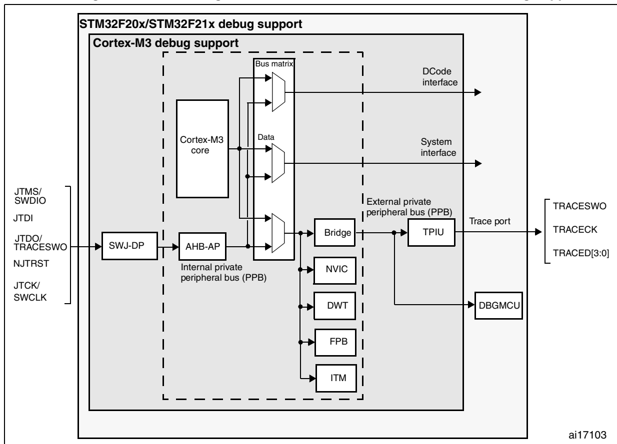
Figure 416. Block diagram of STM32 MCU and Cortex™-M3-level debug support
