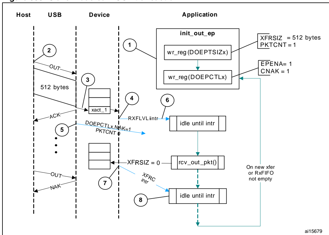
Figure 388. Slave mode bulk OUT transaction
