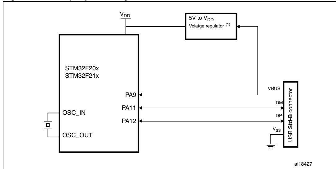
Figure 350. USB peripheral-only connection
