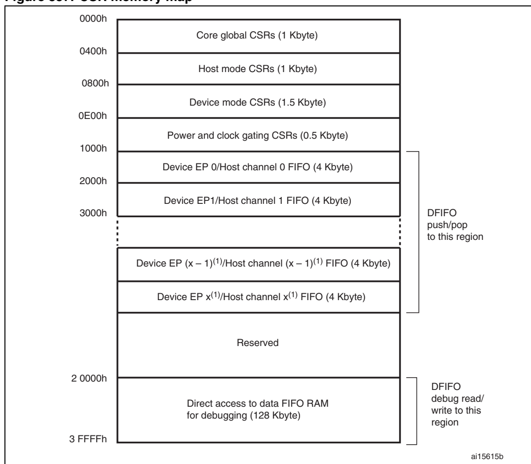
Figure 357. CSR memory map
