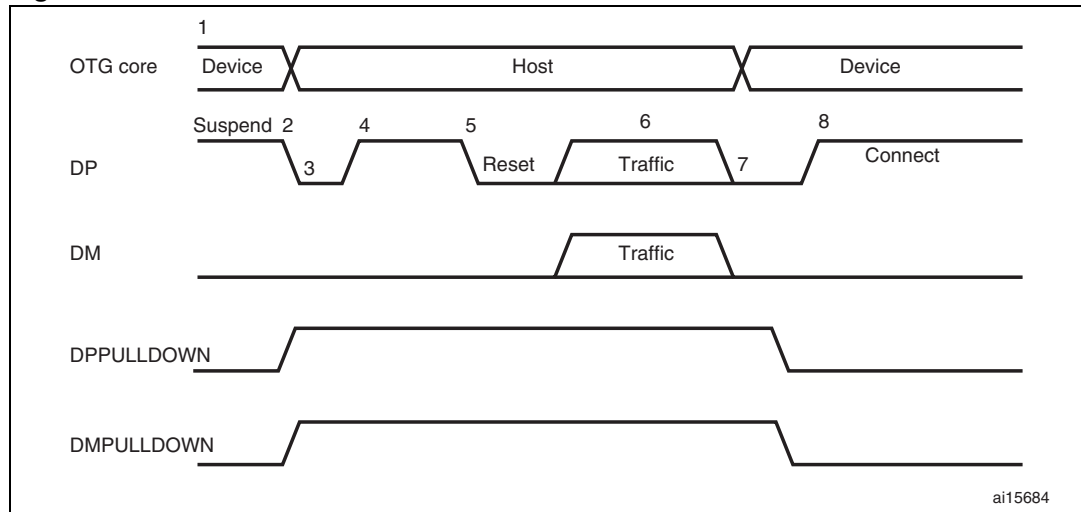
Figure 371. B-device HNP
