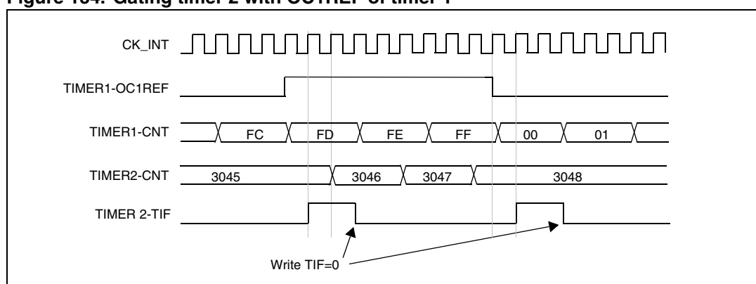
Figure 154. Gating timer 2 with OC1REF of timer 1
