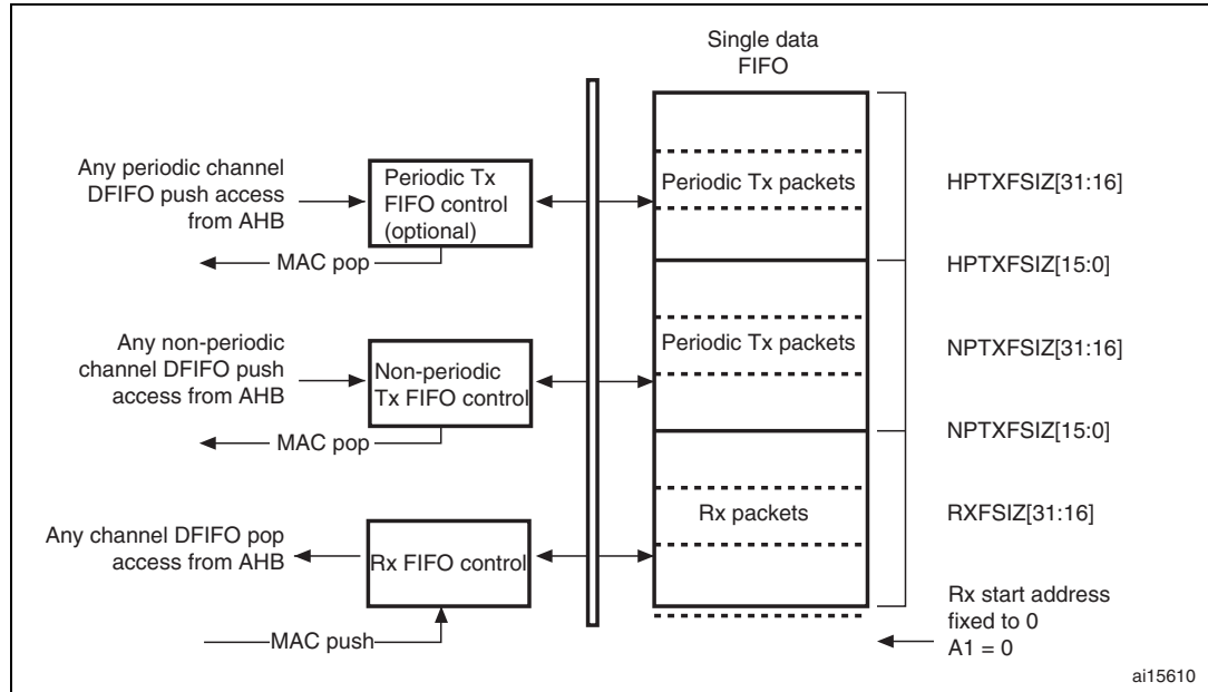
Figure 355. Host-mode FIFO address mapping and AHB FIFO access mapping
