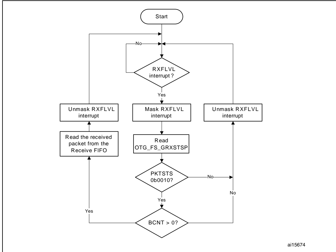
Figure 377. Receive FIFO read task
