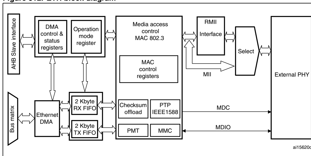
Figure 312. ETH block diagram
