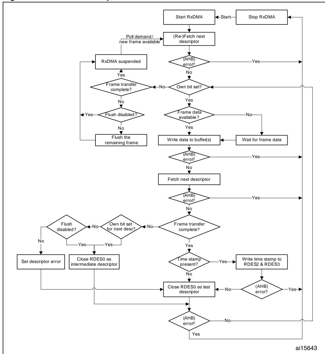
Figure 343. Receive DMA operation
