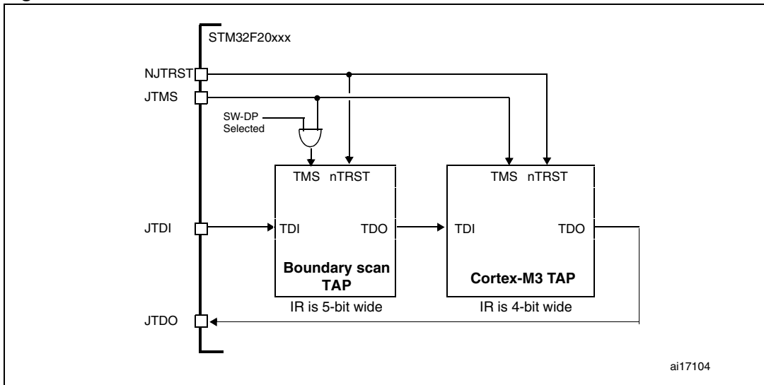
Figure 418. JTAG TAP connections
