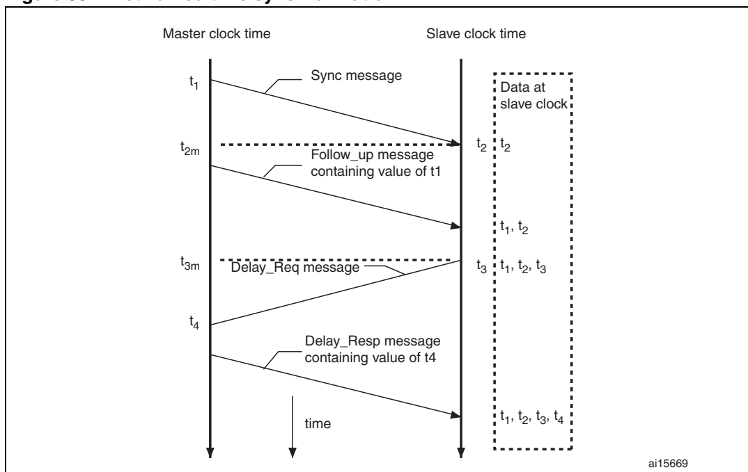
Figure 334. Networked time synchronization
