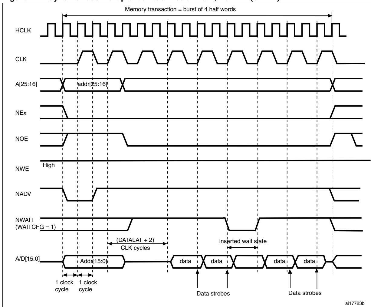
Figure 412. Synchronous multiplexed read mode - NOR, PSRAM (CRAM)
