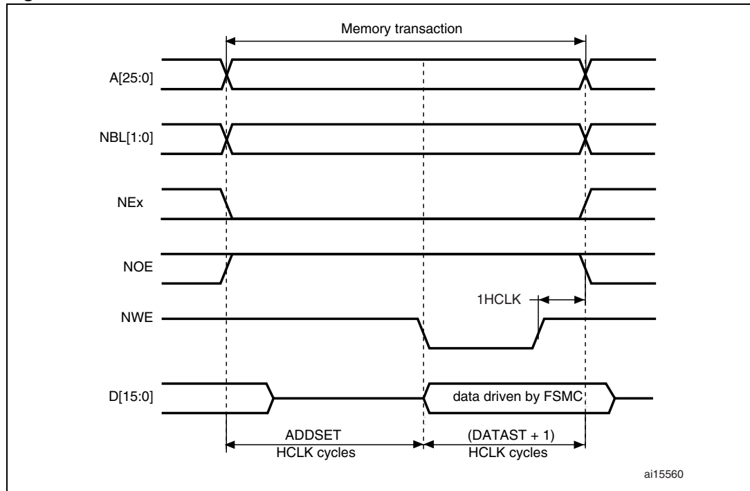
Figure 399. ModeA write accesses
