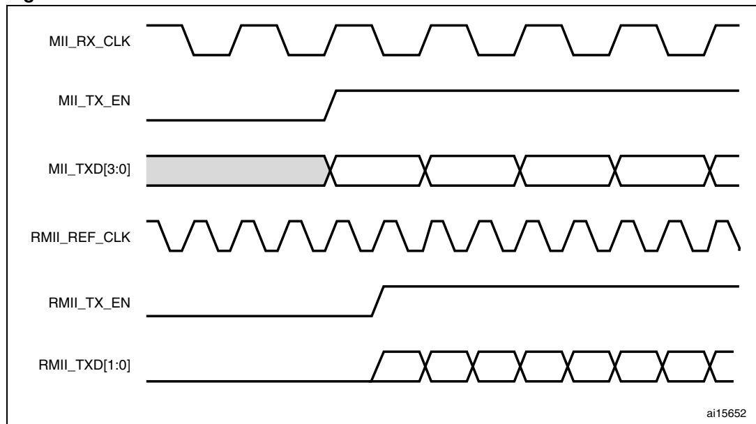
Figure 327. Frame transmission in MII and RMII modes
