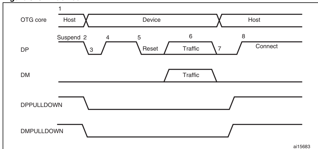
Figure 370. A-device HNP
