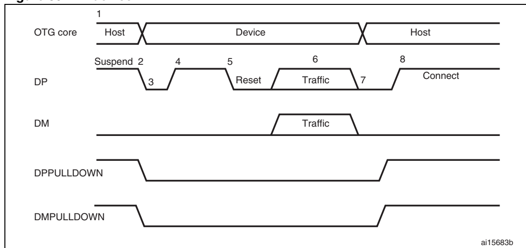
Figure 392. A-device HNP
