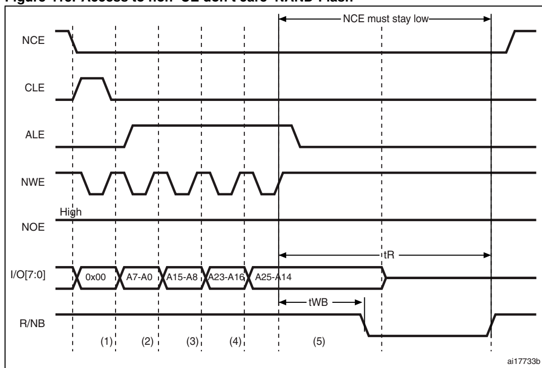
Figure 415. Access to non ‘CE don’t care’ NAND-Flash
