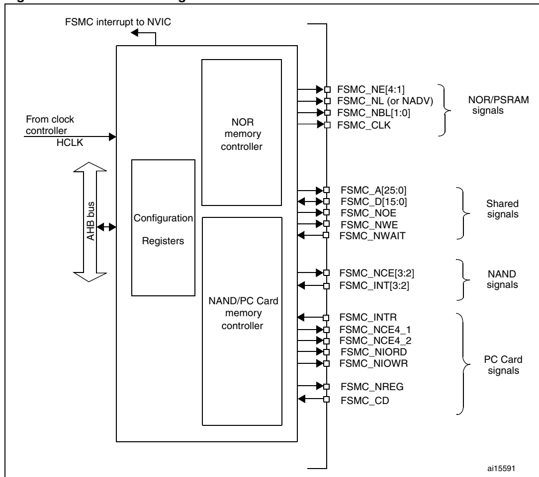
Figure 394. FSMC block diagram
