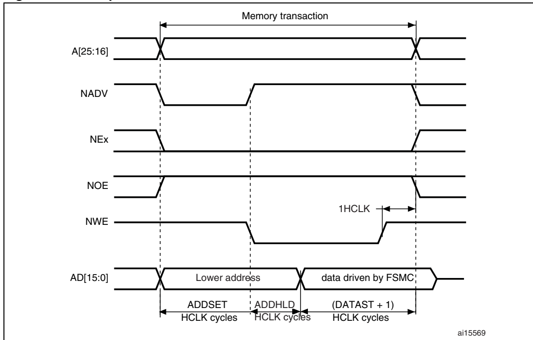
Figure 408. Multiplexed write accesses
