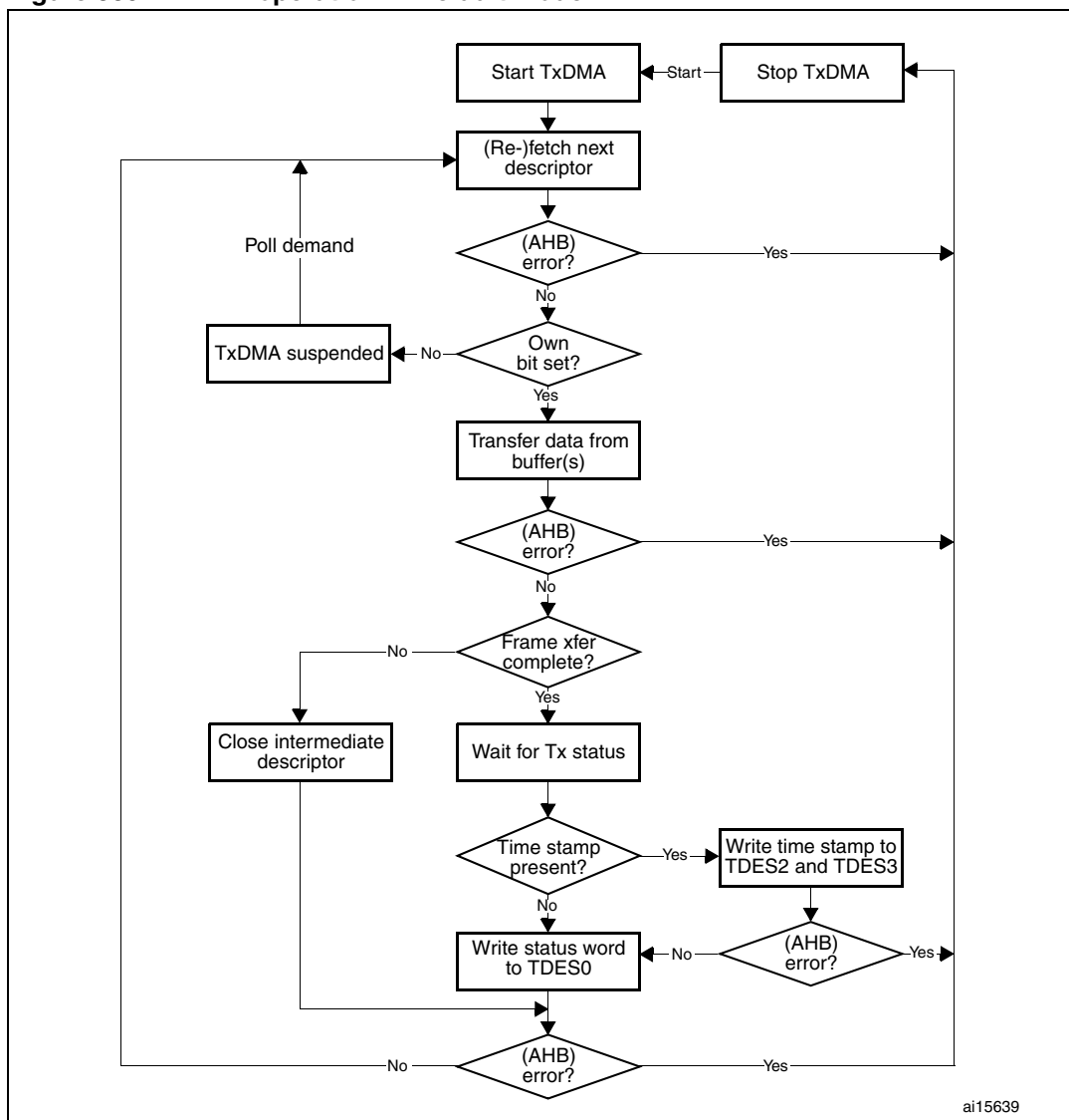
Figure 339. TxDMA operation in Default mode
