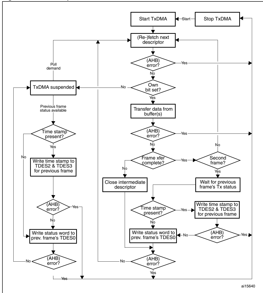
Figure 340. TxDMA operation in OSF mode
