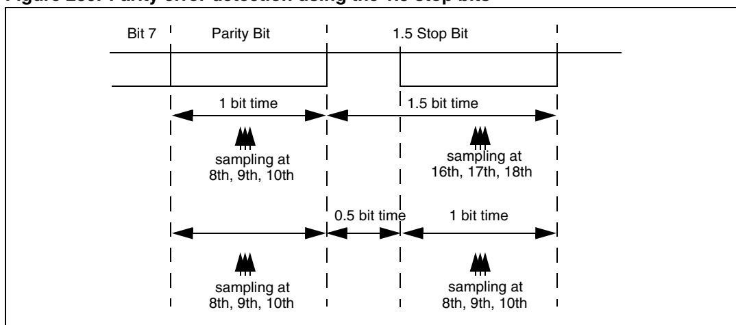
Figure 239. Parity error detection using the 1.5 stop bits
