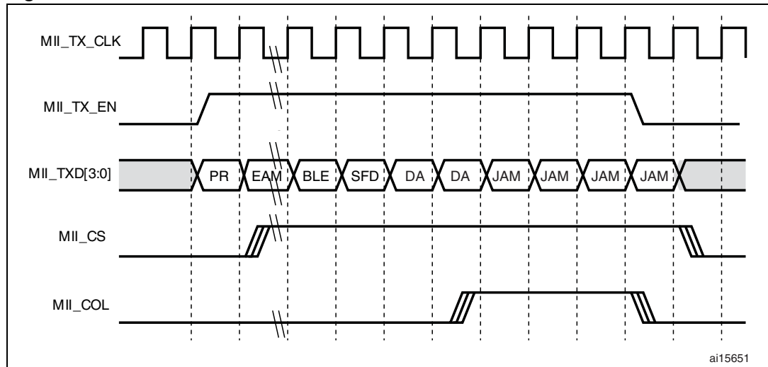
Figure 326. Transmission with collision
