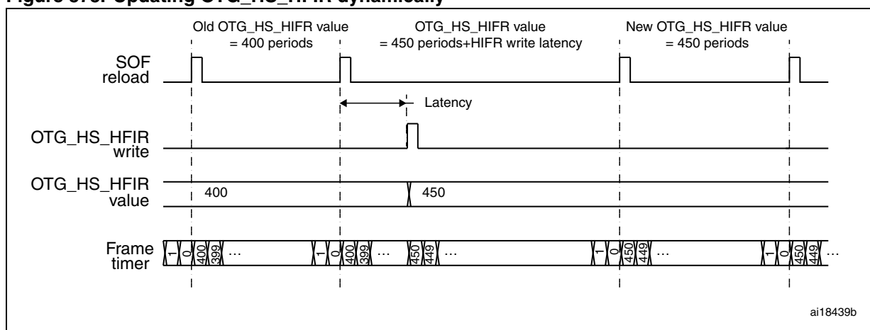
Figure 373. Updating OTG_HS_HFIR dynamically
