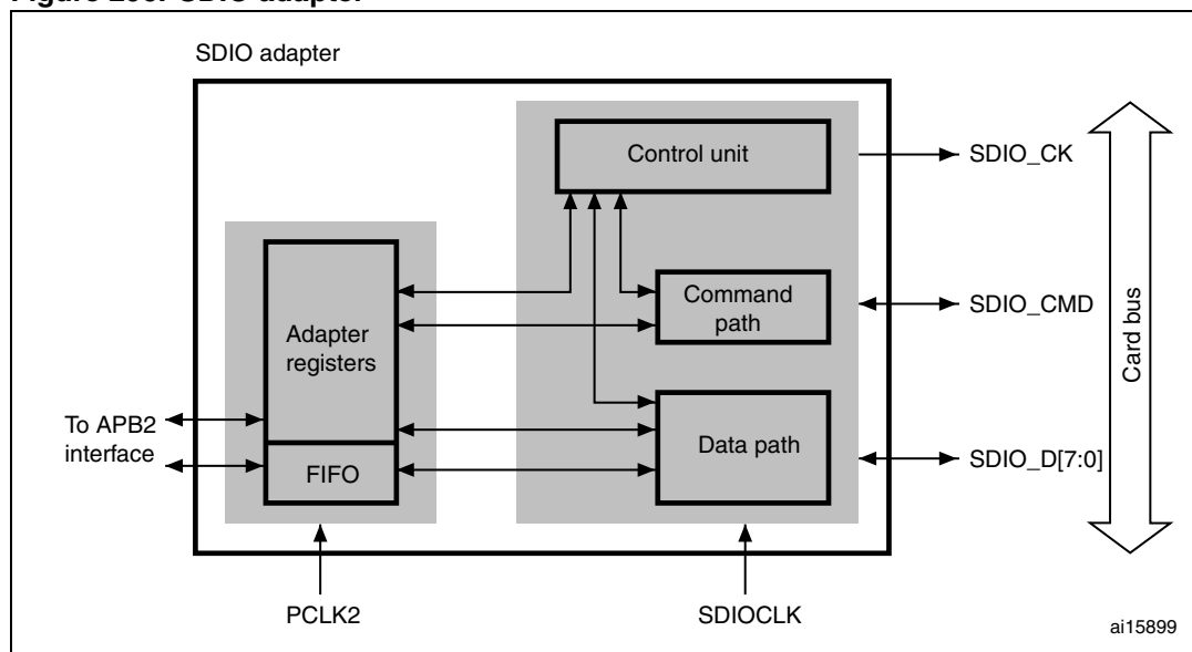
Figure 290. SDIO adapter
