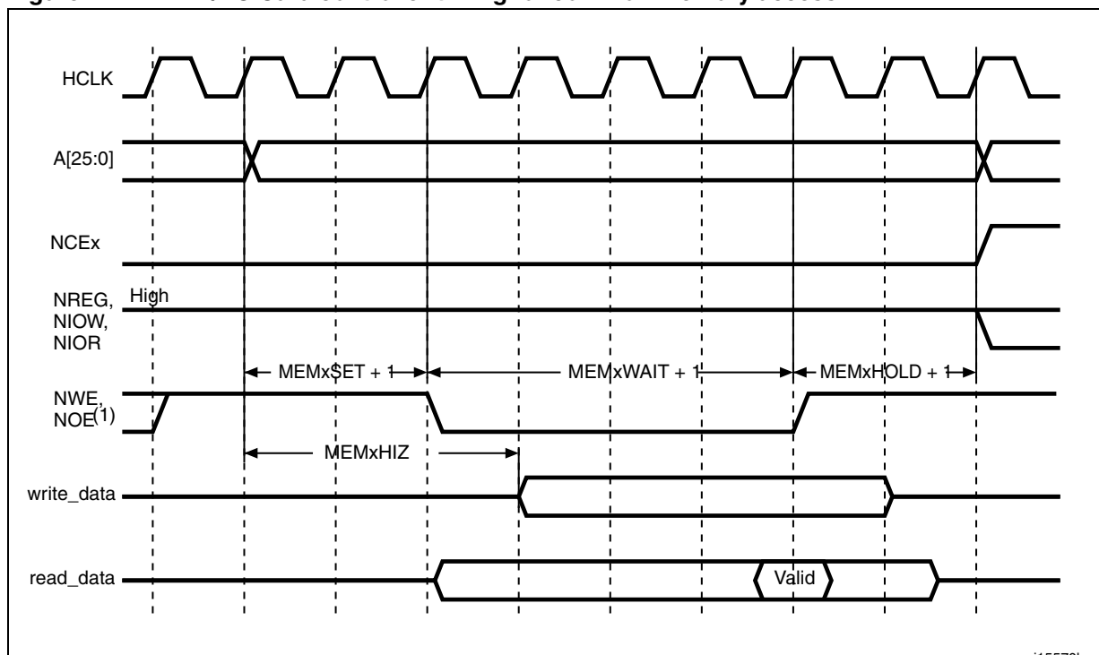
Figure 414. NAND/PC Card controller timing for common memory access
