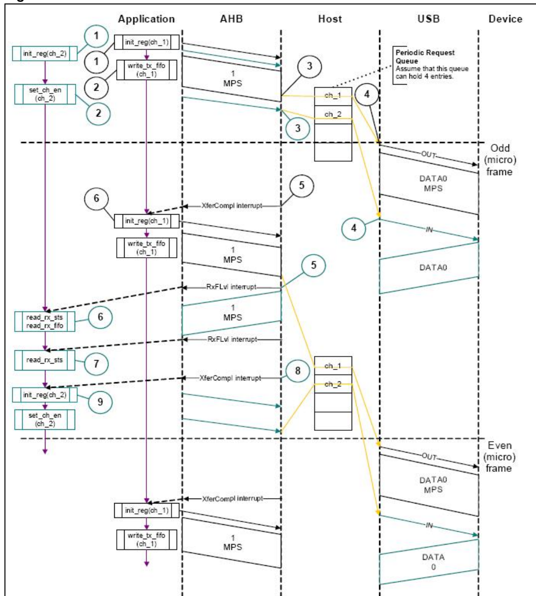
Figure 385. Normal isochronous OUT/IN transactions - Slave mode
