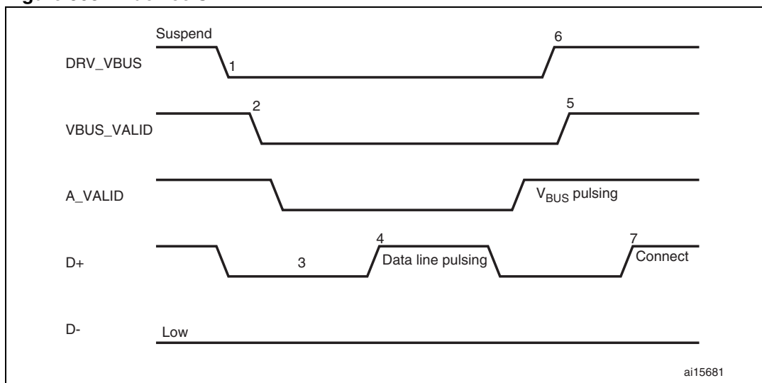
Figure 368. A-device SRP
