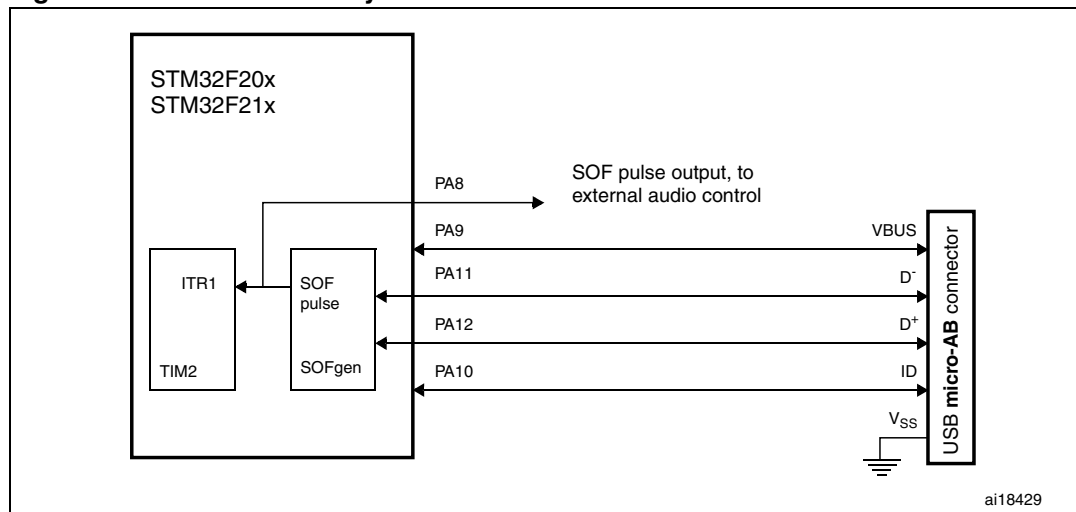
Figure 352. SOF connectivity
