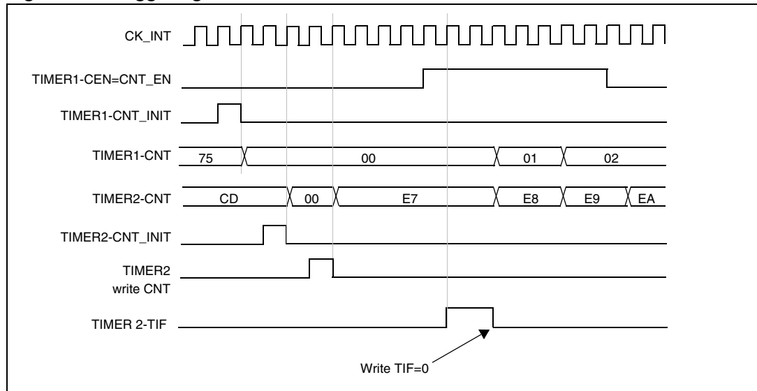
Figure 157. Triggering timer 2 with Enable of timer 1
