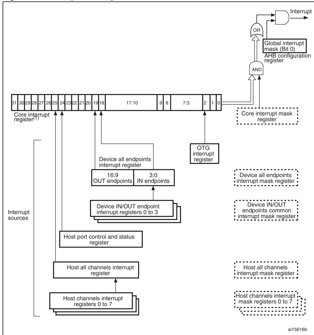
Figure 356. Interrupt hierarchy
