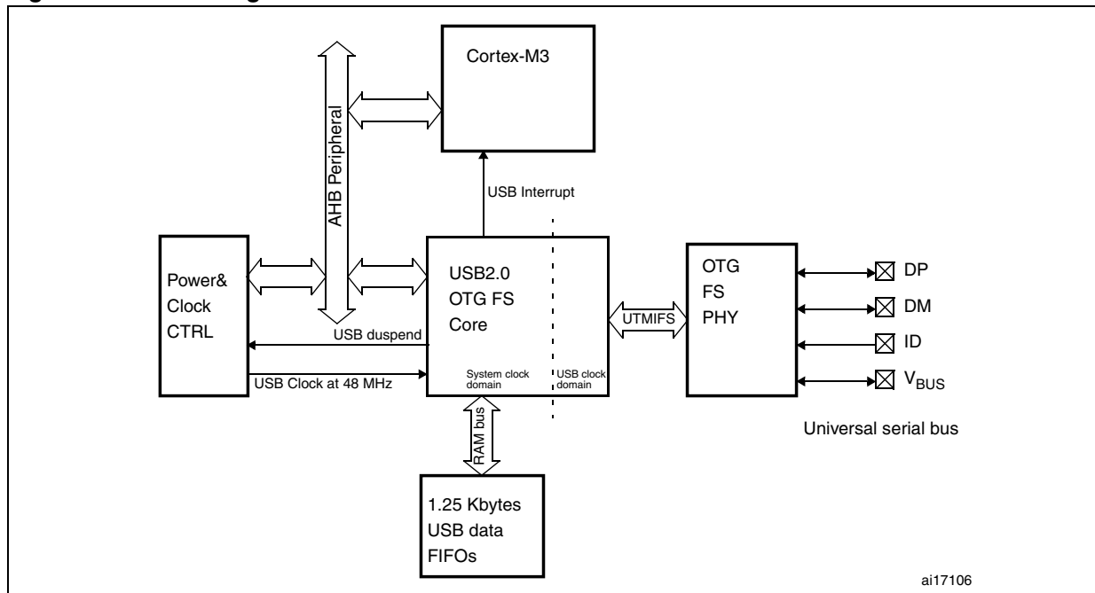
Figure 348. Block diagram
