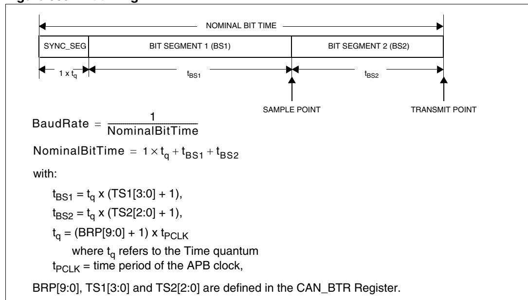
Figure 309. Bit timing
