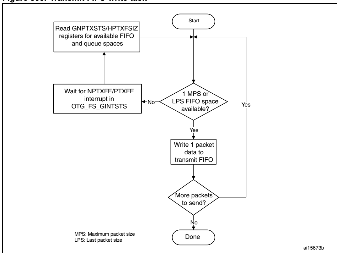
Figure 358. Transmit FIFO write task
