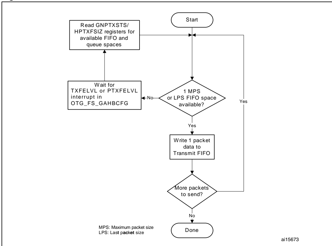
Figure 376. Transmit FIFO write task
