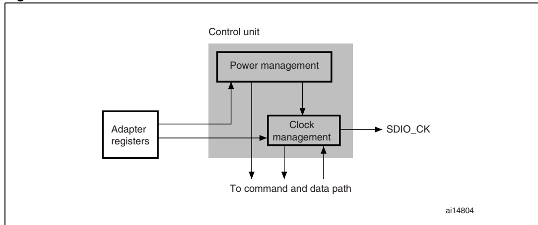
Figure 291. Control unit
