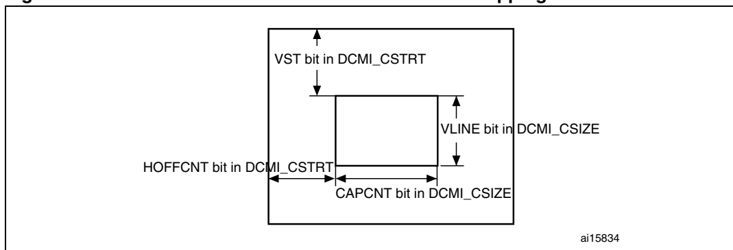
Figure 62. Coordinates and size of the window after cropping
