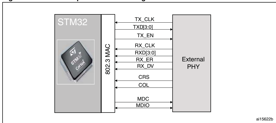
Figure 316. Media independent interface signals
