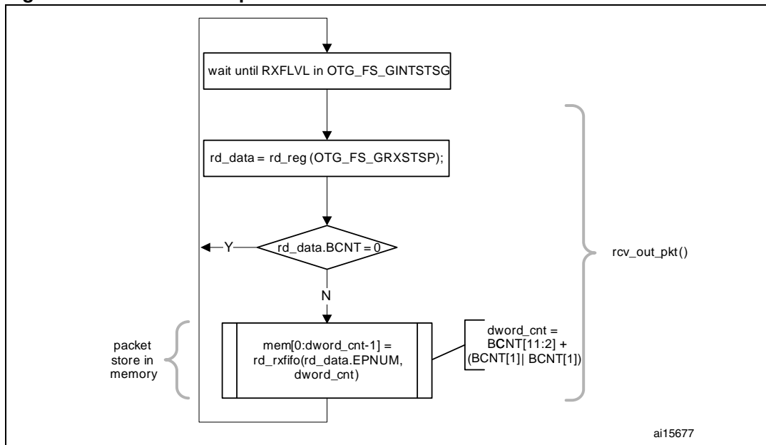
Figure 386. Receive FIFO packet read in slave mode
