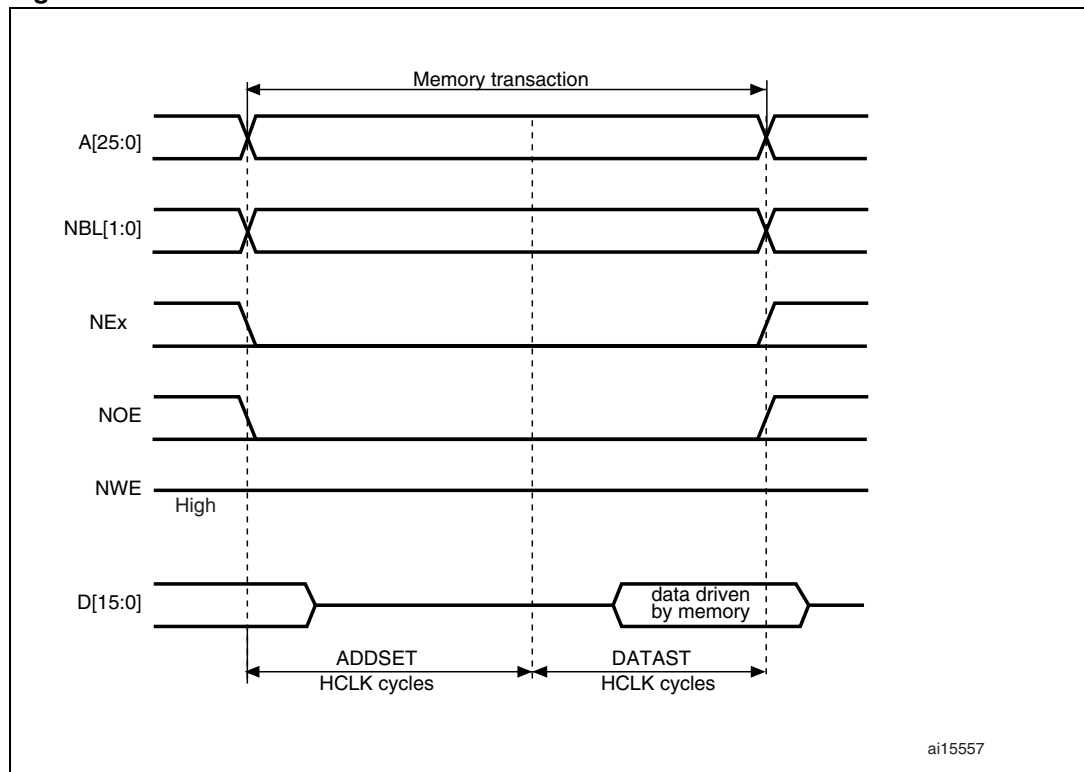
Figure 396. Mode1 read accesses
