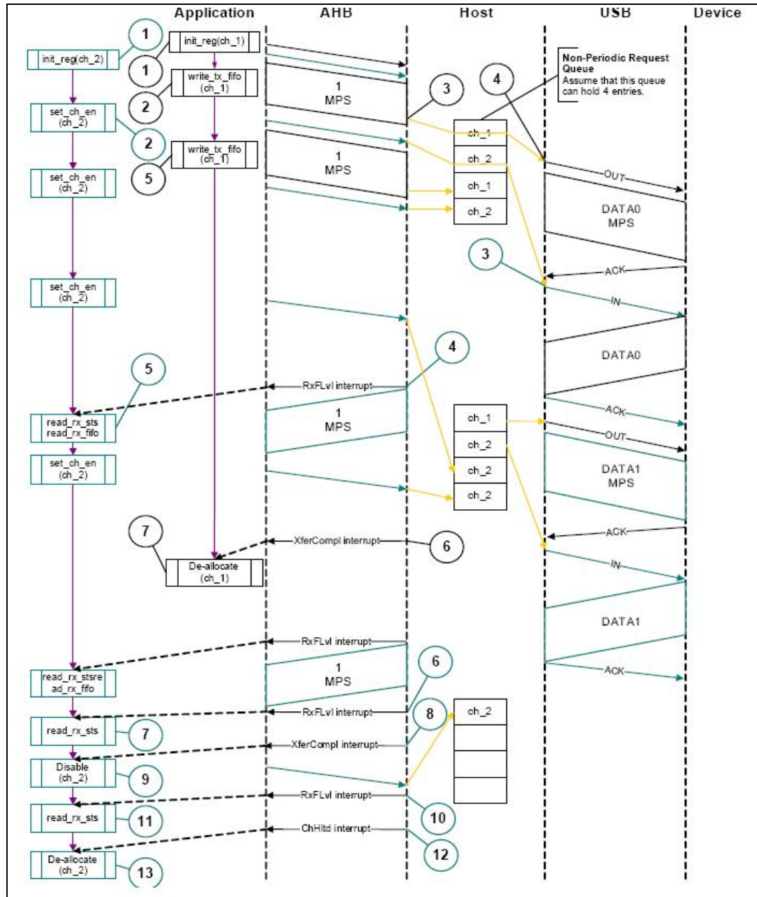
Figure 379. Normal bulk/control OUT/SETUP and bulk/control IN transactions - Slave mode
