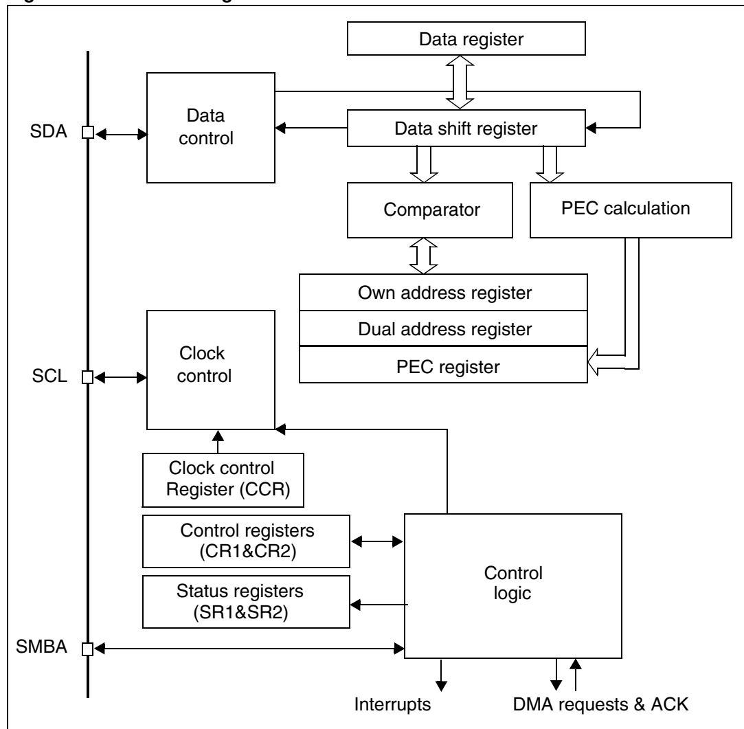
Figure 217. I 2 C block diagram
