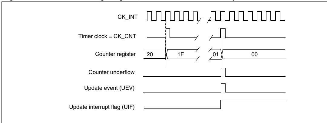
Figure 130. Counter timing diagram, internal clock divided by N
