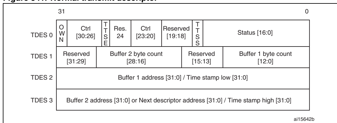
Figure 341. Normal transmit descriptor
