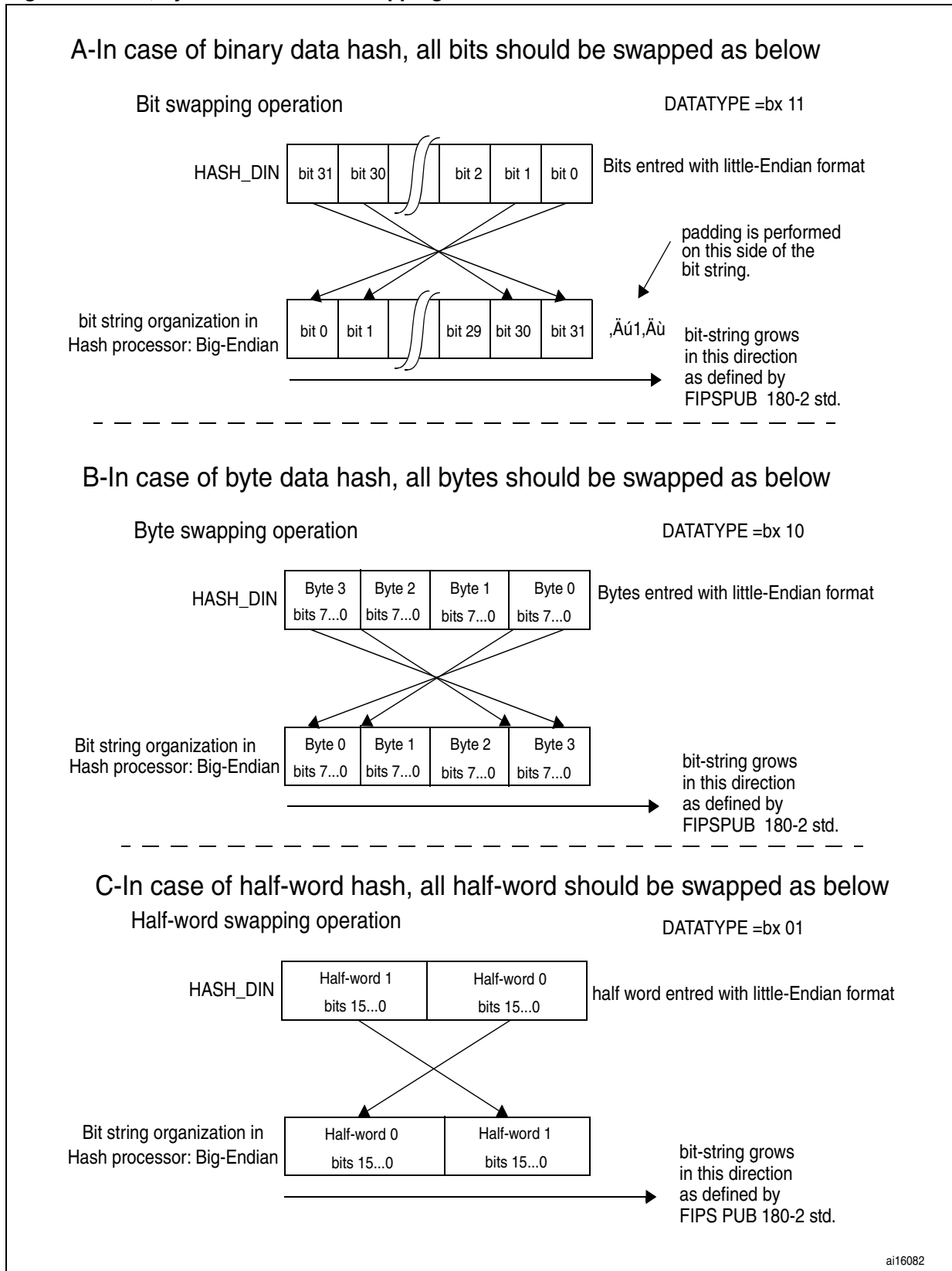
Figure 213. Bit, byte and half-word swapping
