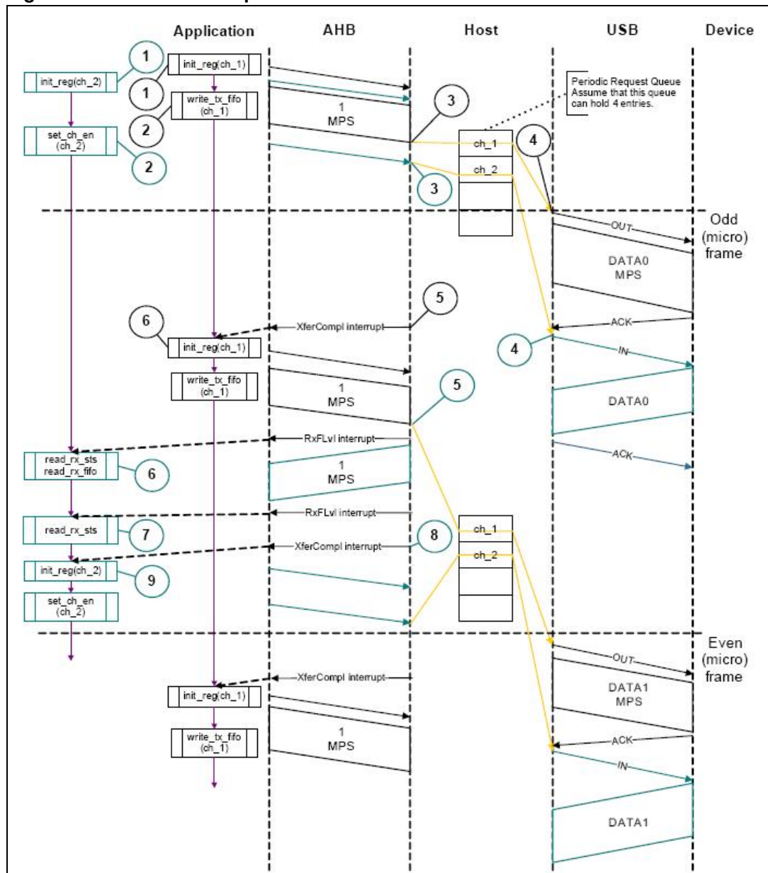
Figure 383. Normal interrupt OUT/IN transactions - Slave mode
