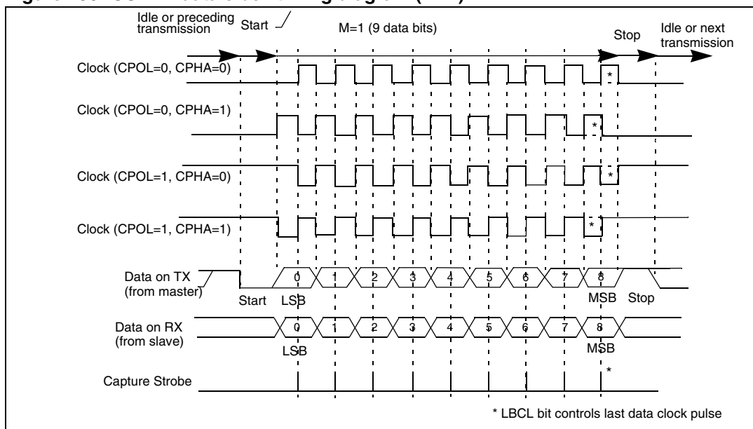
Figure 236. USART data clock timing diagram (M=1)
