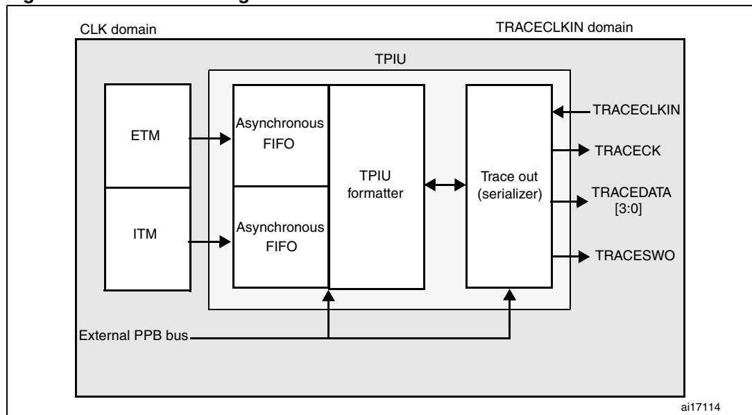
Figure 419. TPIU block diagram
