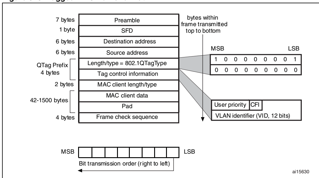
Figure 323. Tagged MAC frame format
