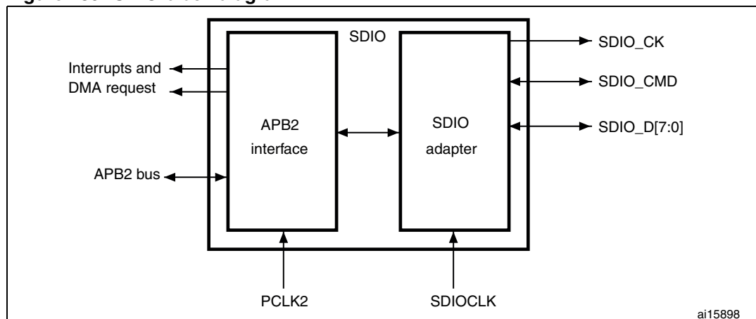
Figure 289. SDIO block diagram
