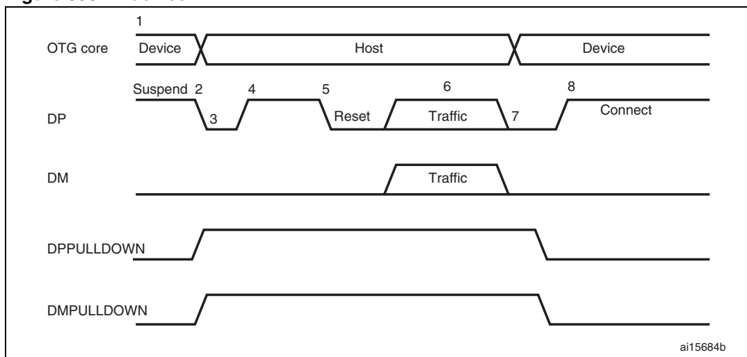
Figure 393. B-device HNP
