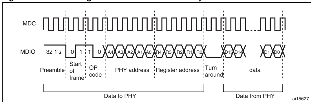
Figure 315. MDIO timing and frame structure - Read cycle
