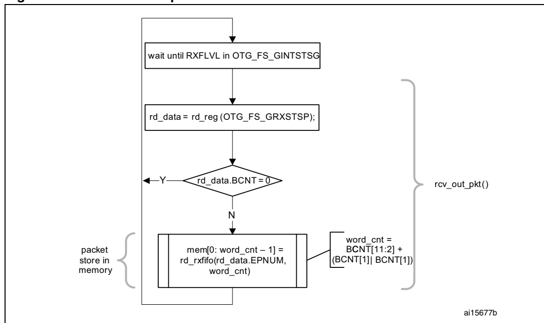
Figure 364. Receive FIFO packet read
