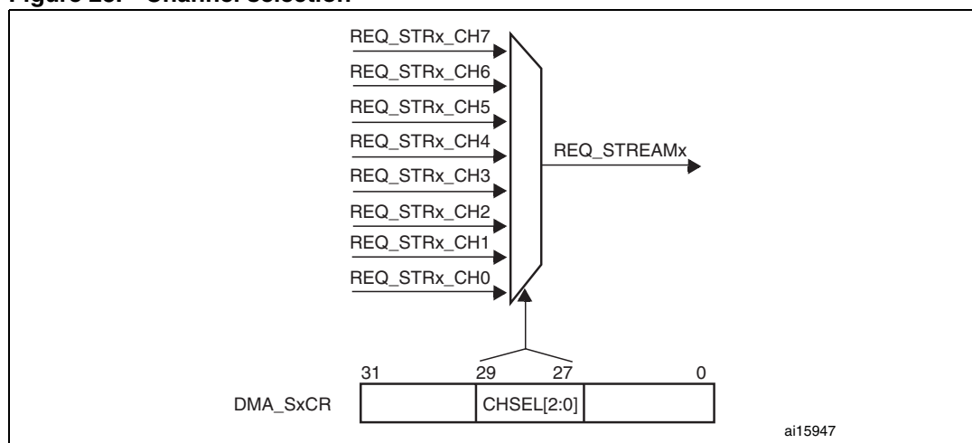
Figure 23. Channel selection
