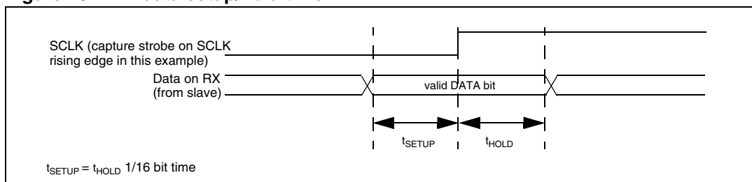
Figure 237. RX data setup/hold time
