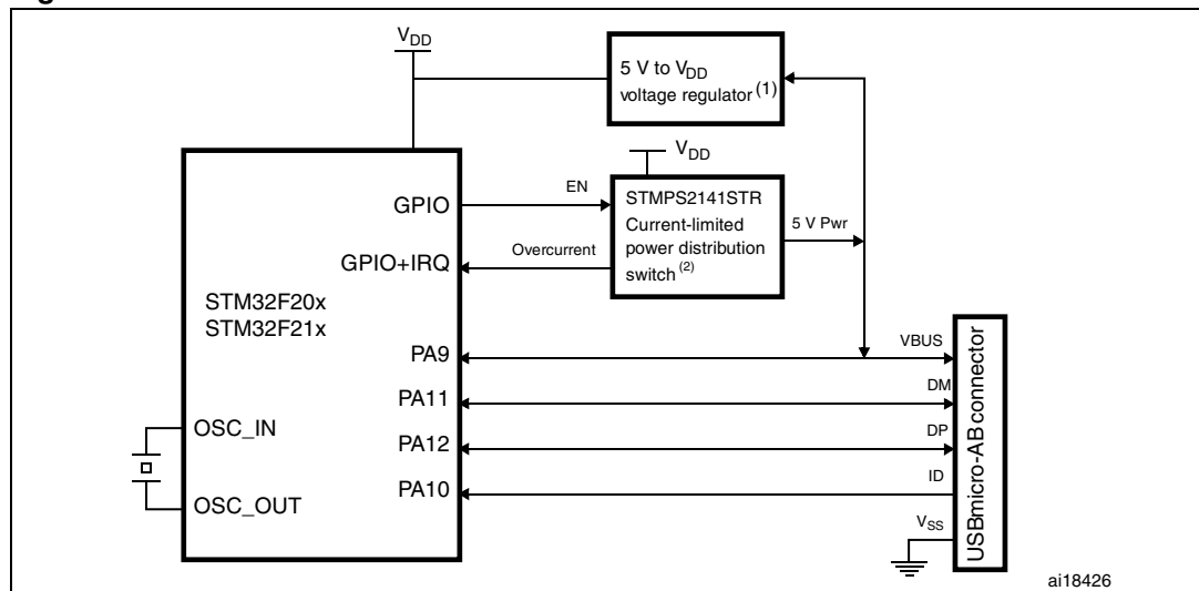
Figure 349. OTG A-B device connection
