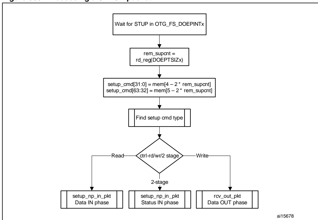
Figure 365. Processing a SETUP packet
