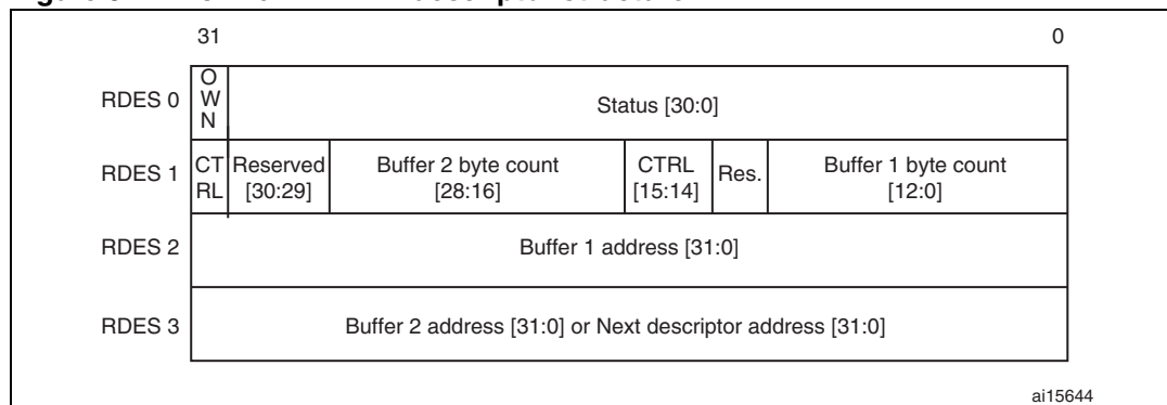
Figure 344. Normal Rx DMA descriptor structure
