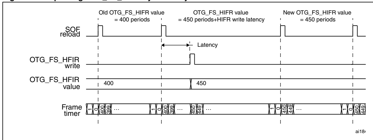
Figure 353. Updating OTG_FS_HFIR dynamically
