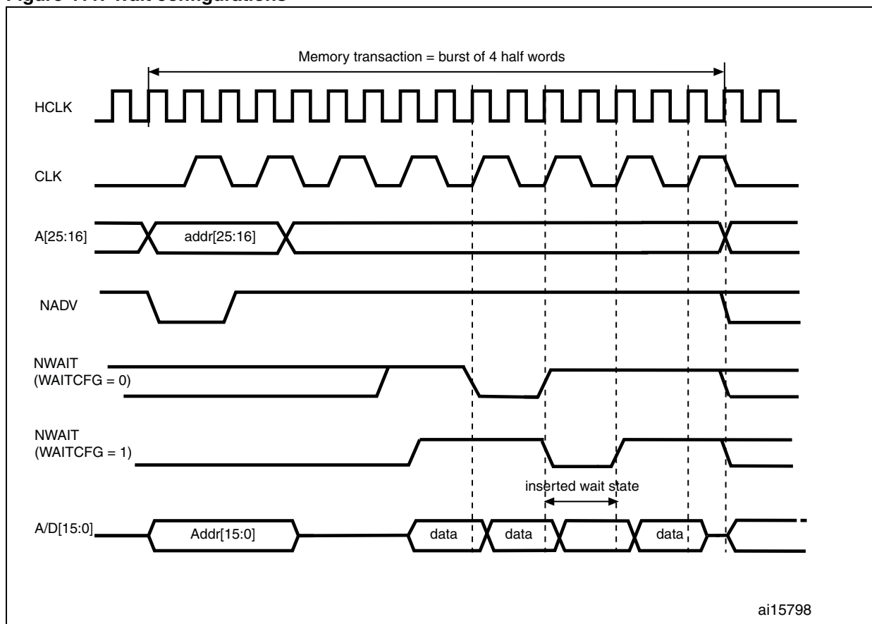
Figure 411. Wait configurations
