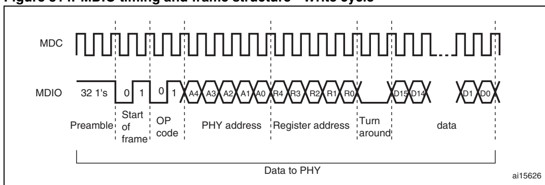
Figure 314. MDIO timing and frame structure - Write cycle
