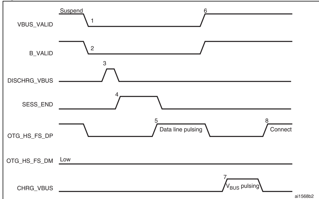
Figure 391. B-device SRP
