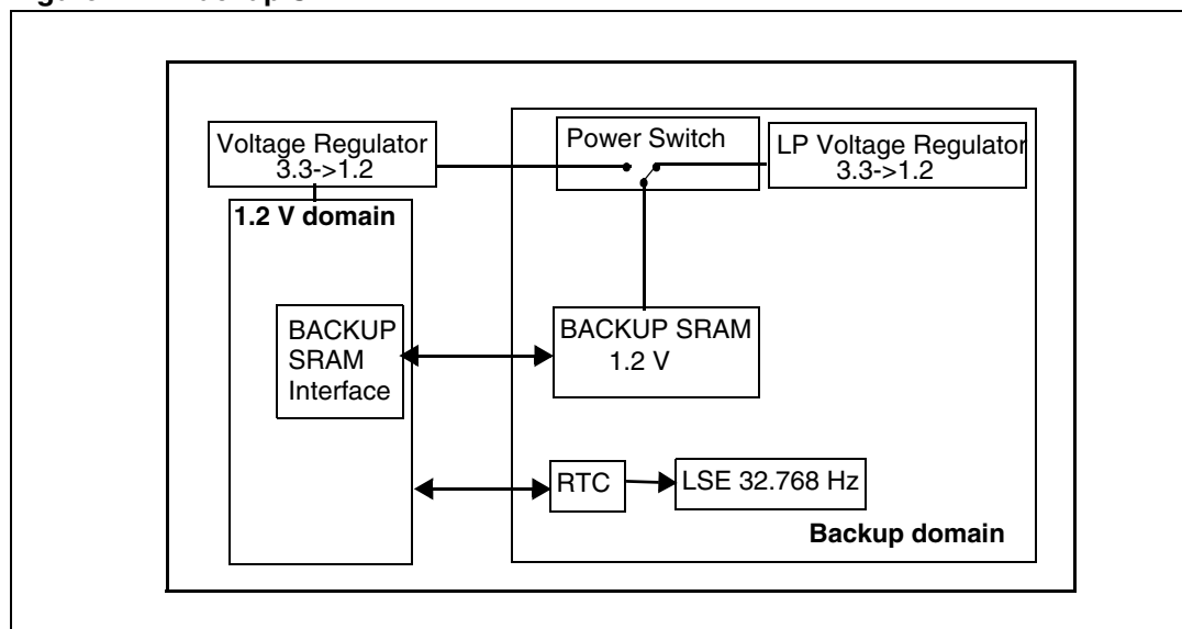
Figure 4. Backup SRAM
