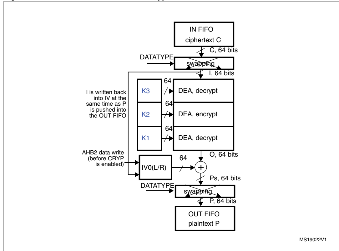
Figure 199. DES/TDES-CBC mode decryption
