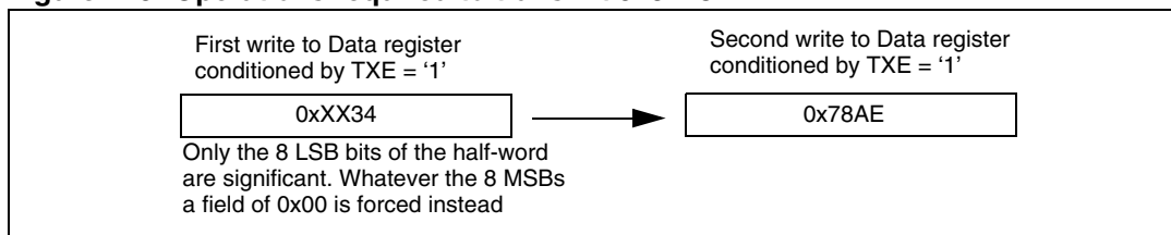
Figure 276. Operations required to transmit 0x3478AE
