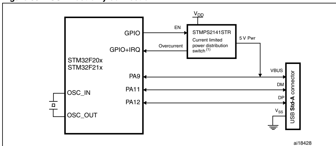
Figure 351. USB host-only connection
