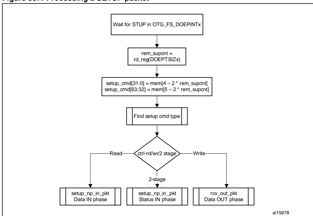
Figure 387. Processing a SETUP packet
