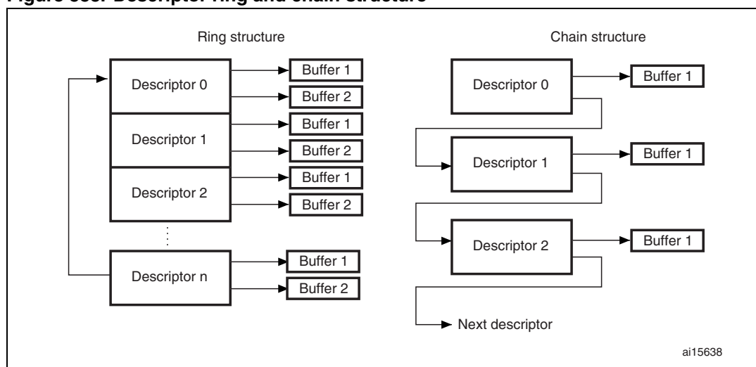
Figure 338. Descriptor ring and chain structure
