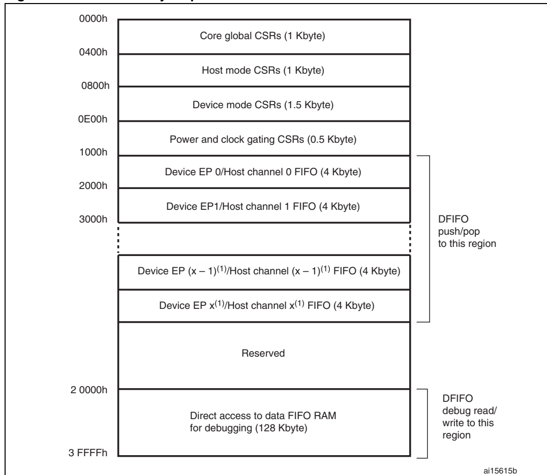
Figure 375. CSR memory map
