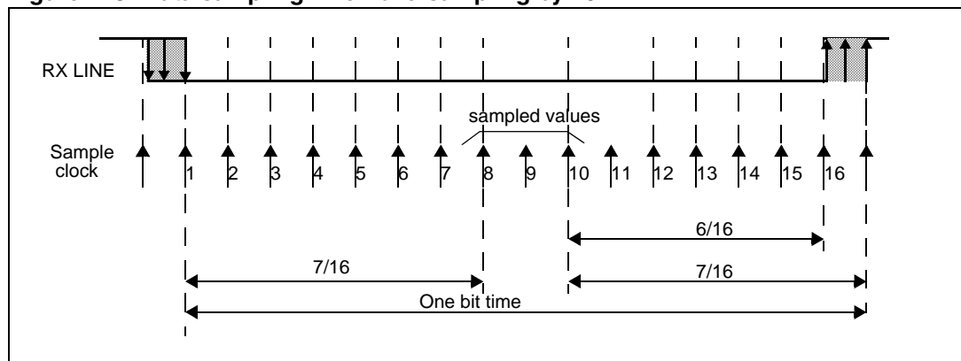
Figure 229. Data sampling when oversampling by 8
