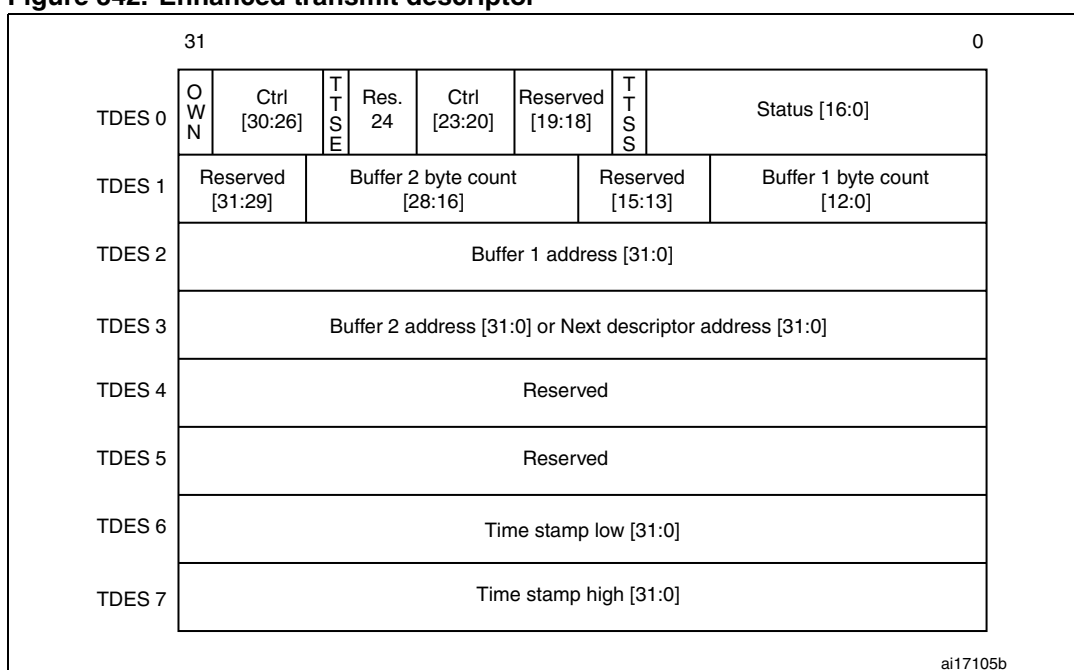
Figure 342. Enhanced transmit descriptor
