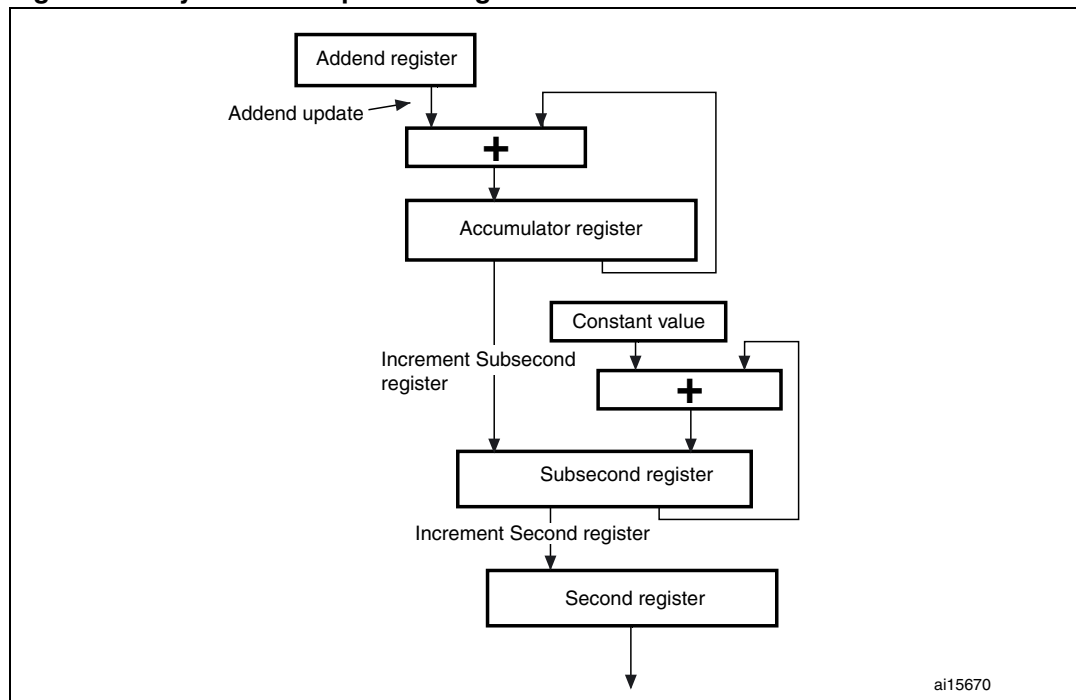
Figure 335. System time update using the Fine correction method
