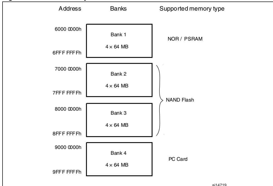
Figure 395. FSMC memory banks
