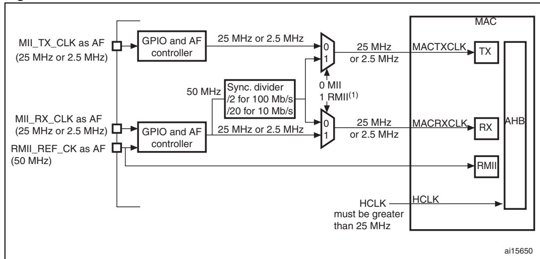
Figure 320. Clock scheme
