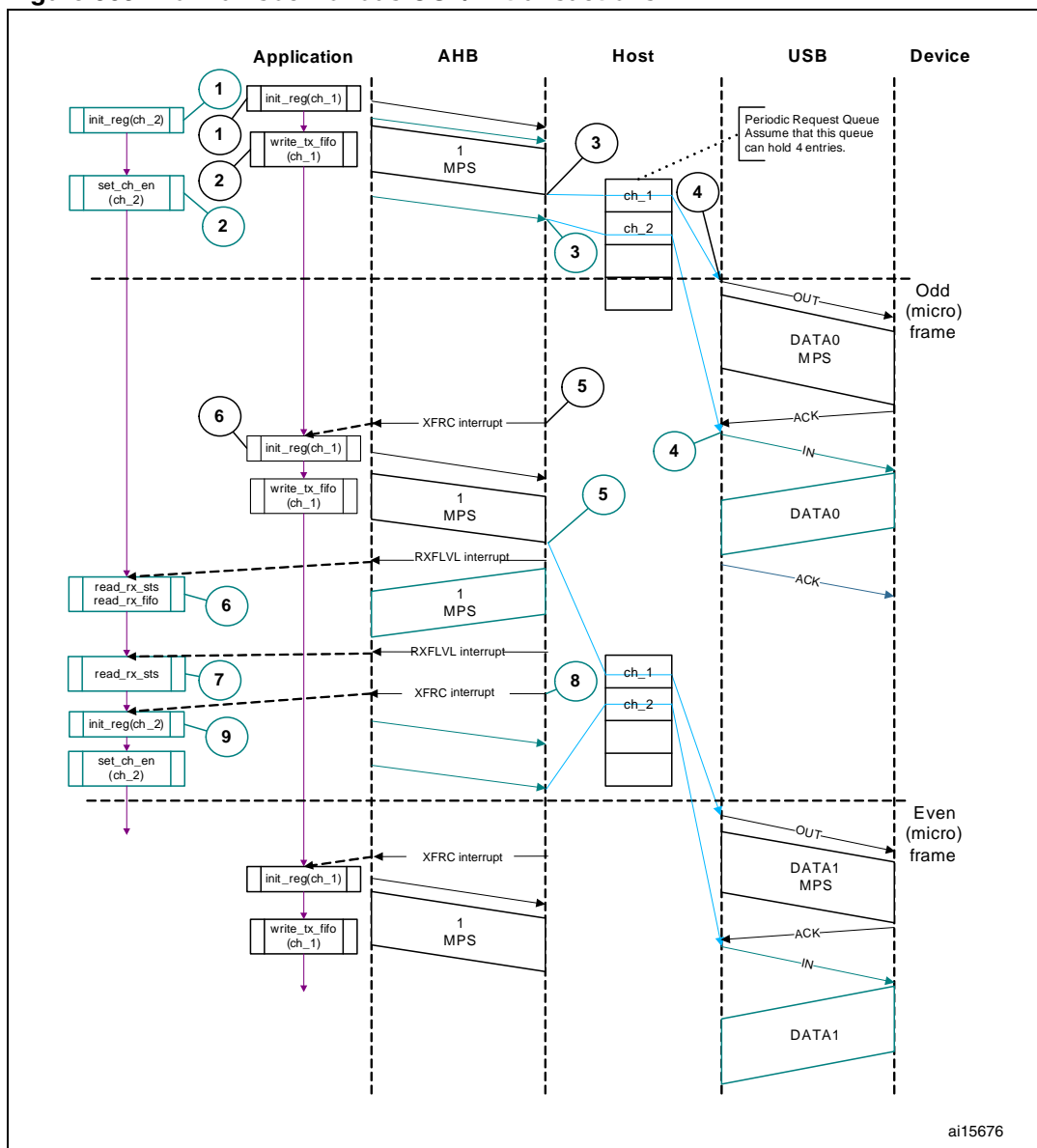
Figure 363. Normal isochronous OUT/IN transactions
