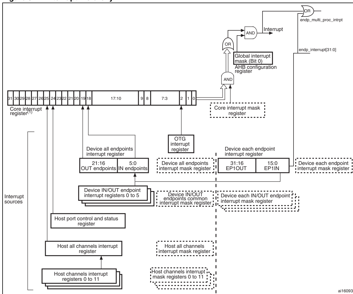
Figure 374. Interrupt hierarchy
