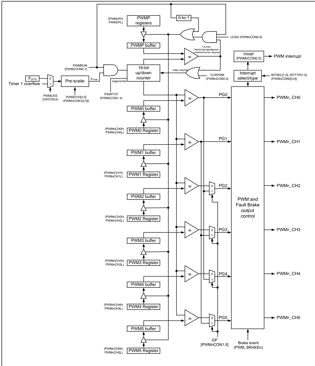
Figure 6.8-1 PWM Block Diagram
