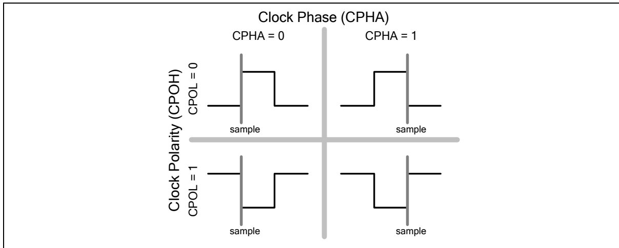
Figure 6.11-4 SPI Clock Formats
