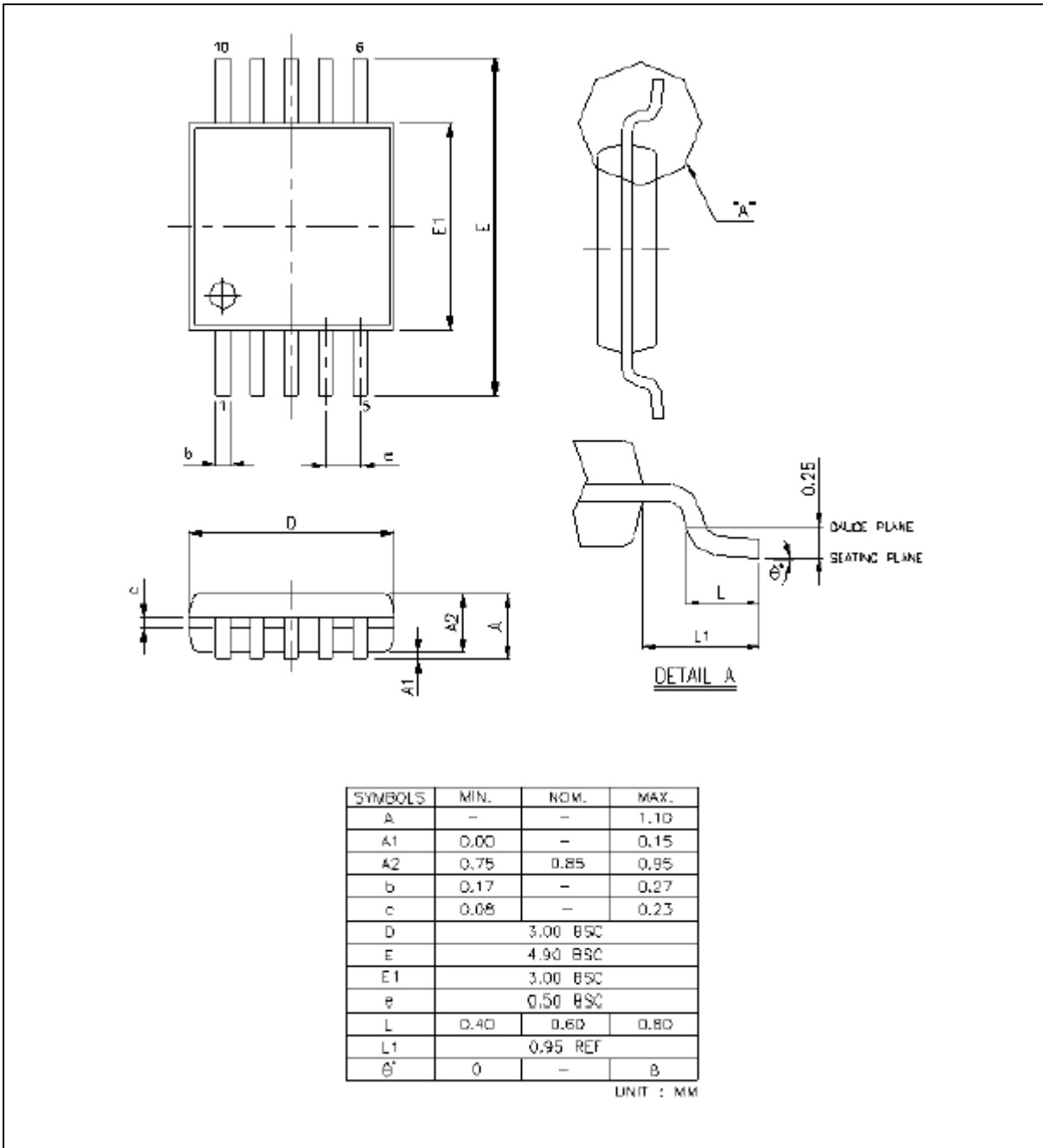
Figure 9.2-1 MSOP-10 Package Dimension
