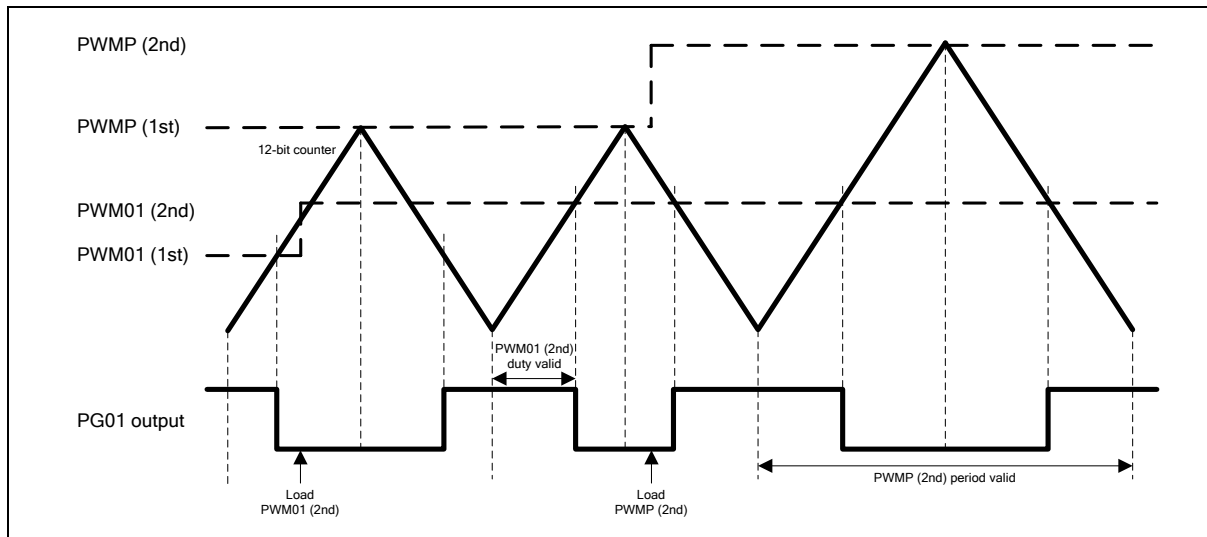
Figure 6.8-4 PWM Center-aligned Type Waveform
