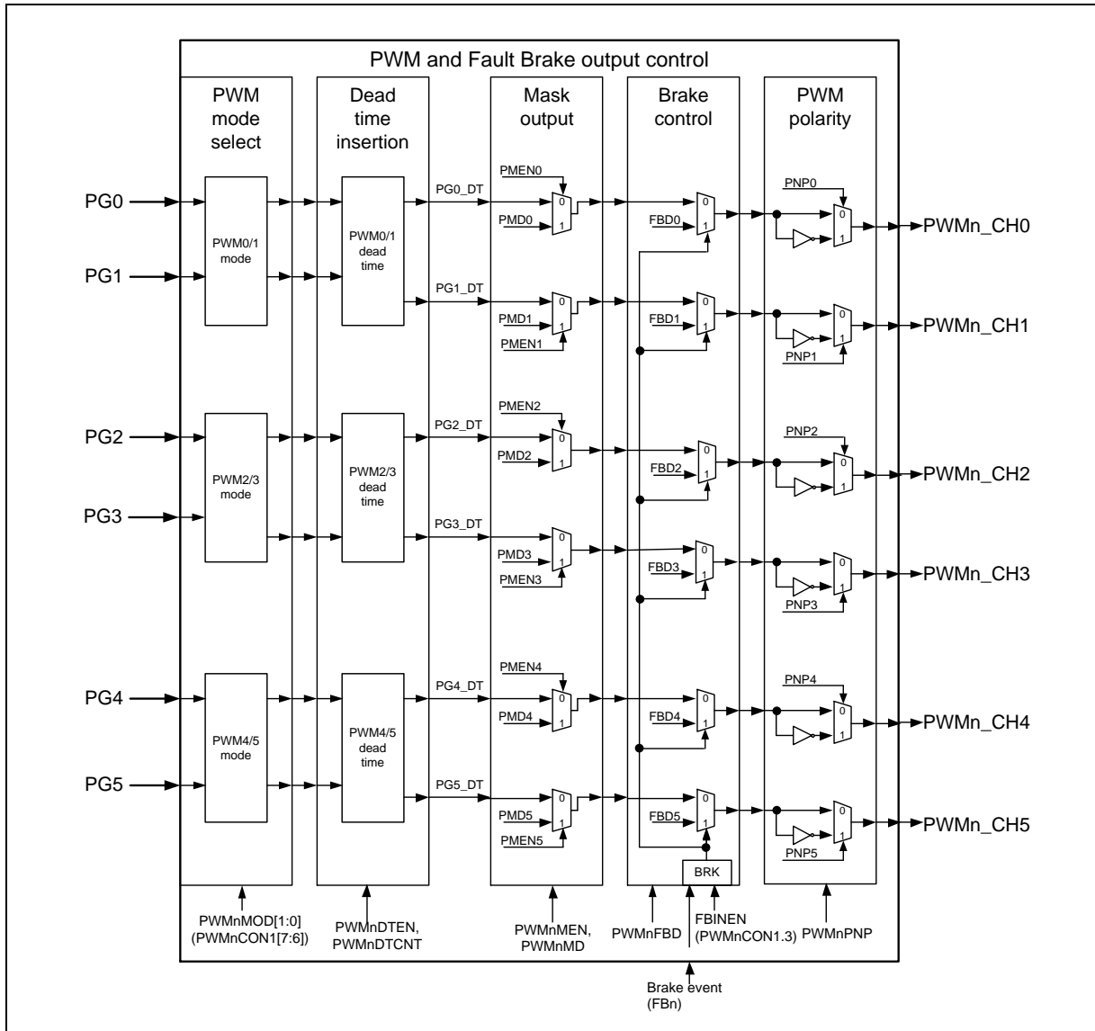
Figure 6.8-2 PWM and Fault Brake Output Control Block Diagram
