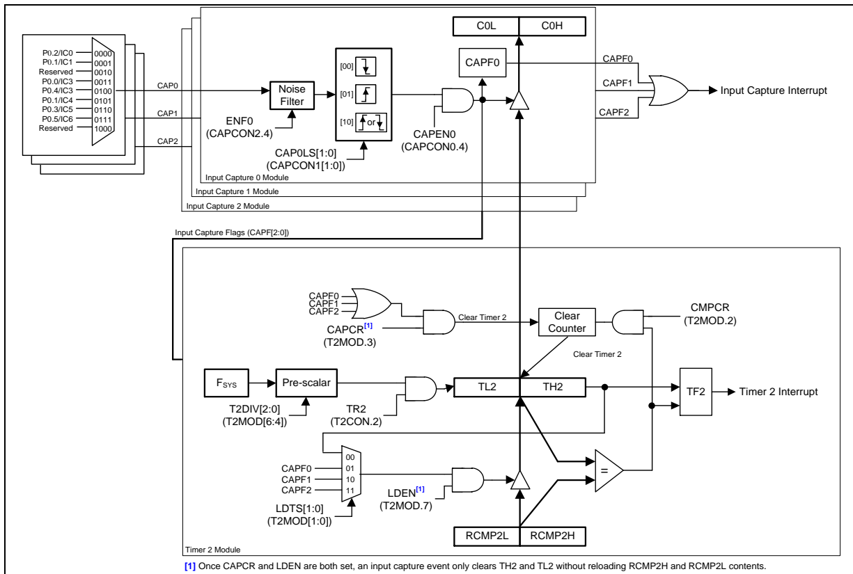
Figure 6.5-5 Timer 2 Full Function Block Diagram
