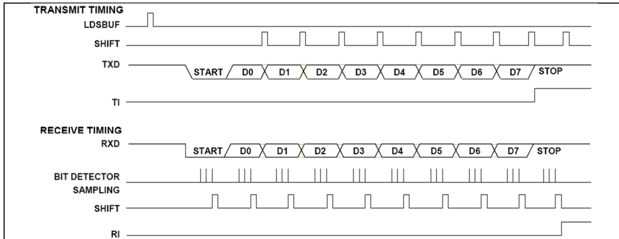
Figure 6.9-2 Serial Port Mode 1 Timing Diagram
