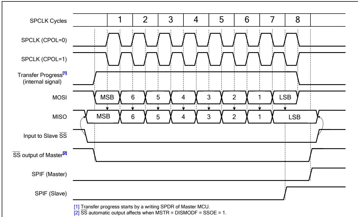
Figure 6.11-5 SPI Clock and Data Format with CPHA = 0
