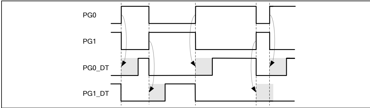
Figure 6.8-5 PWM Complementary Mode with Dead-time Insertion
