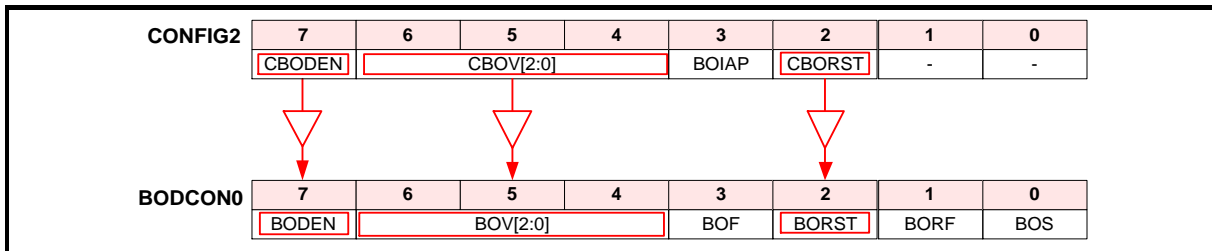
Figure 6.1-3 CONFIG2 Power-On Reset Reloading
