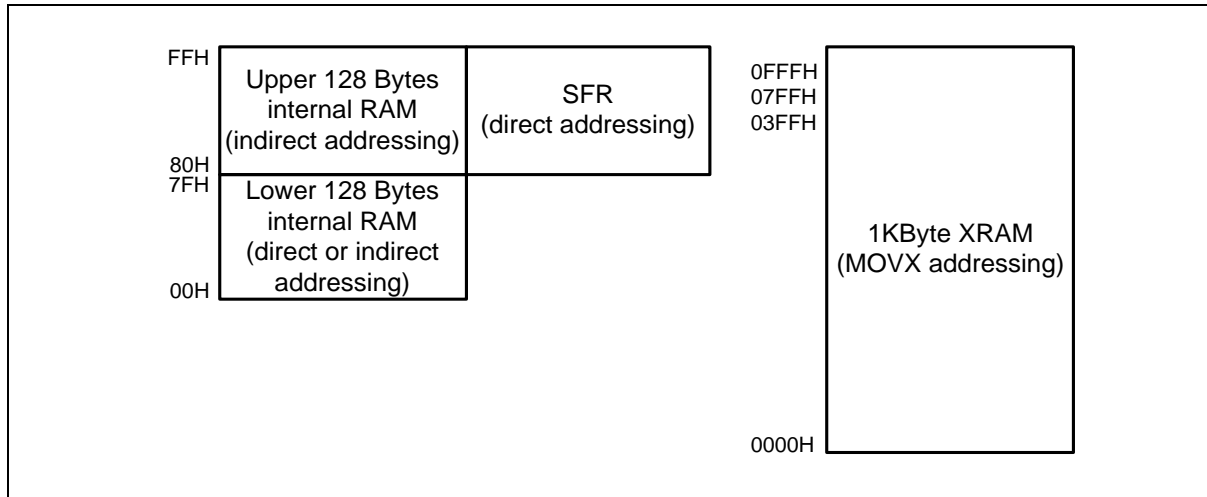
Figure 6.1-4 Data Memory Map
