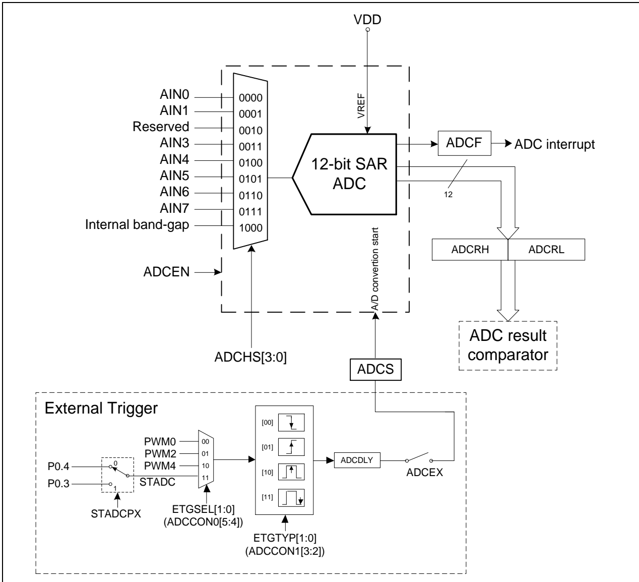
Figure 6.12-112-bit ADC Block Diagram
