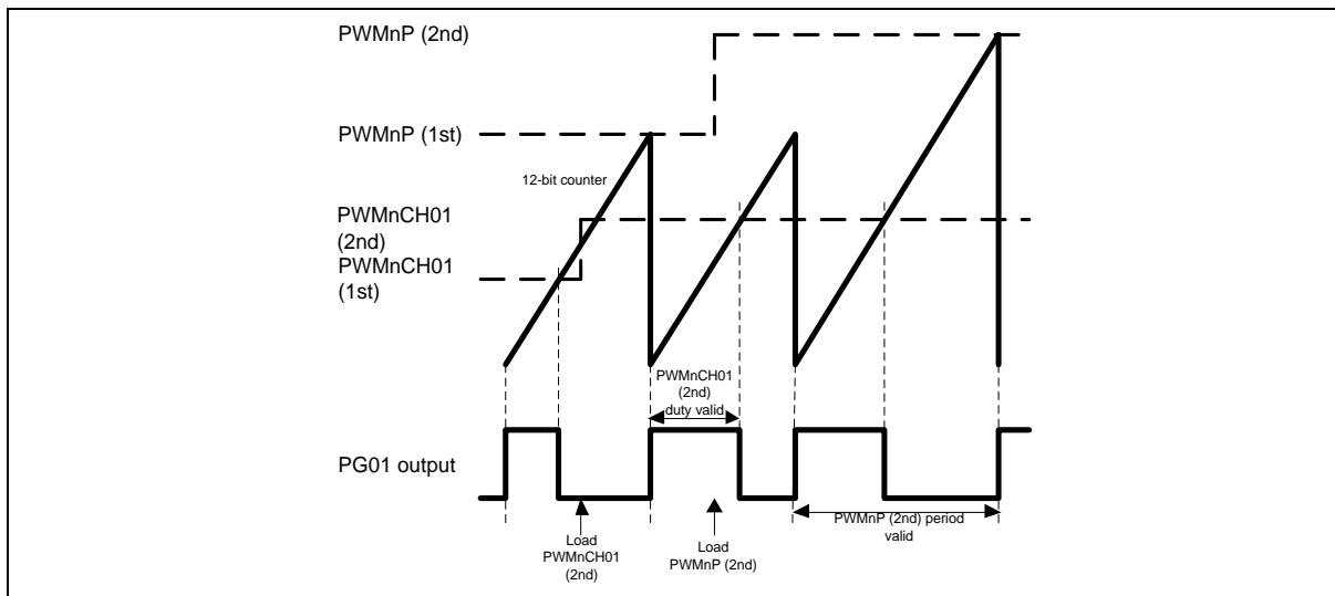
Figure 6.8-3 PWM Edge-aligned Type Waveform
