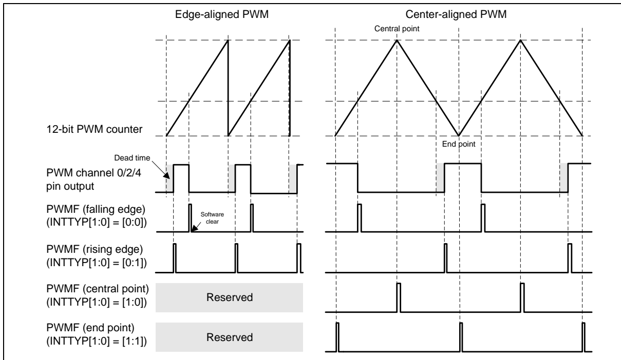
Figure 6.8-7 PWM Interrupt Type
