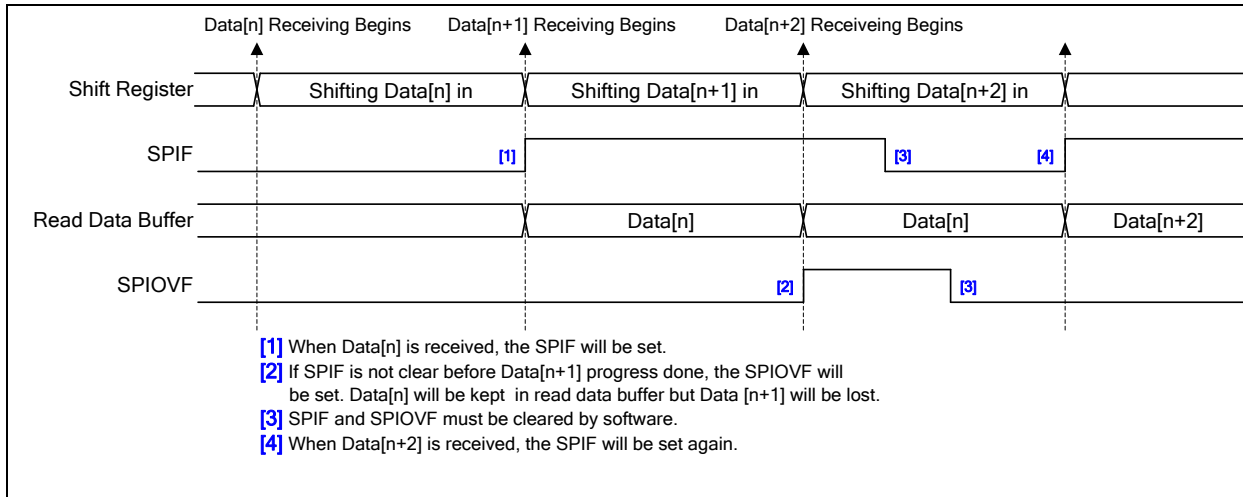
Figure 6.11-7 SPI Overrun Waveform
