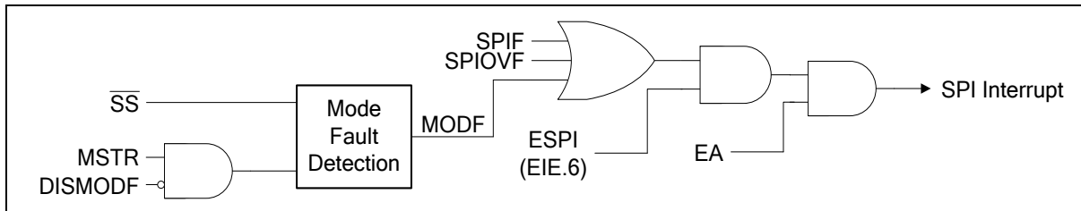
Figure 6.11-8 SPI Interrupt Request
