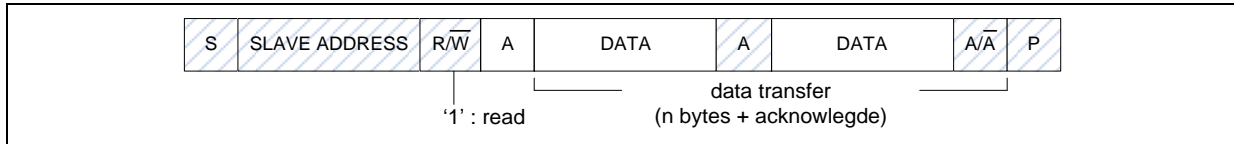
Figure 6.10-5 Master Reads Data from Slave by 7-bit
