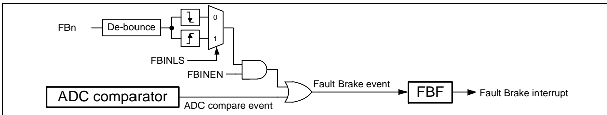
Figure 6.8-6 Fault Brake Function Block Diagram
