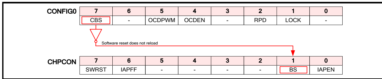
Figure 6.1-2 CONFIG0 Any Reset Reloading
