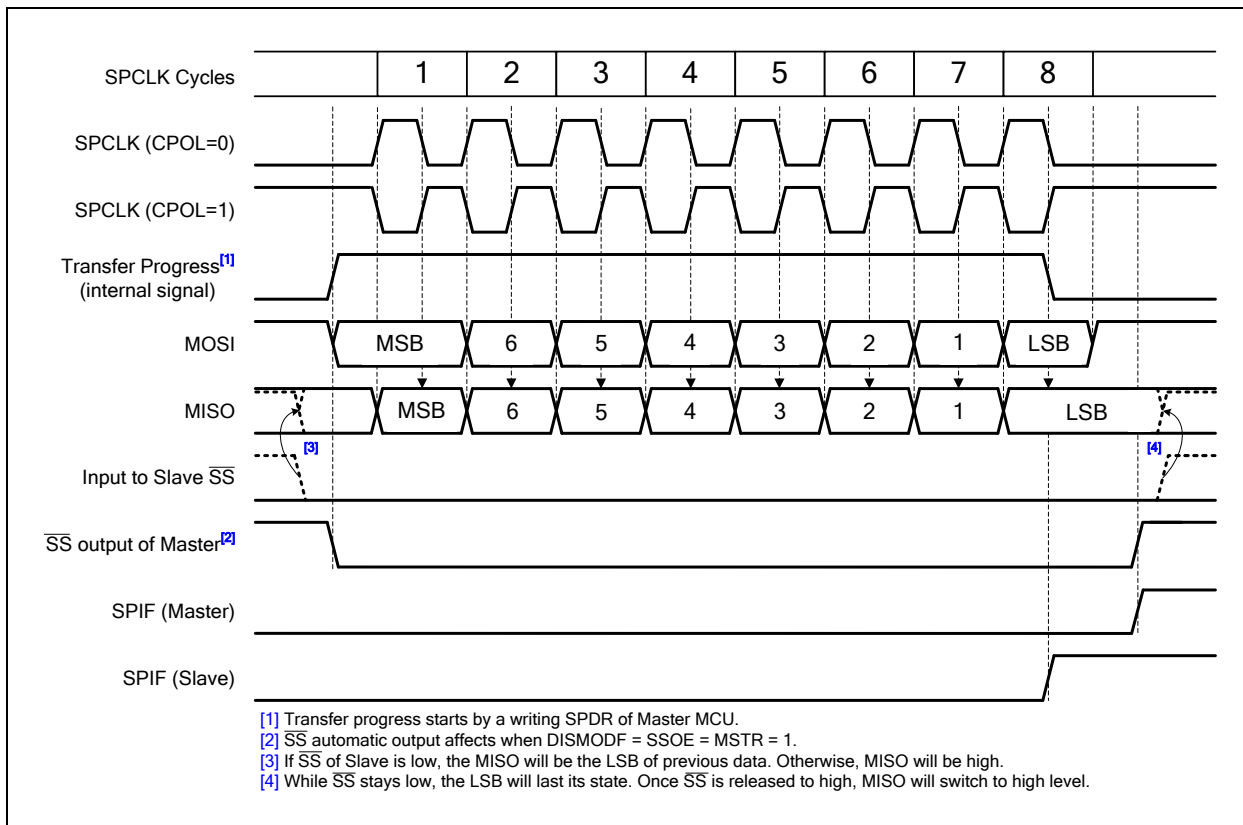
Figure 6.11-6 SPI Clock and Data Format with CPHA = 1
