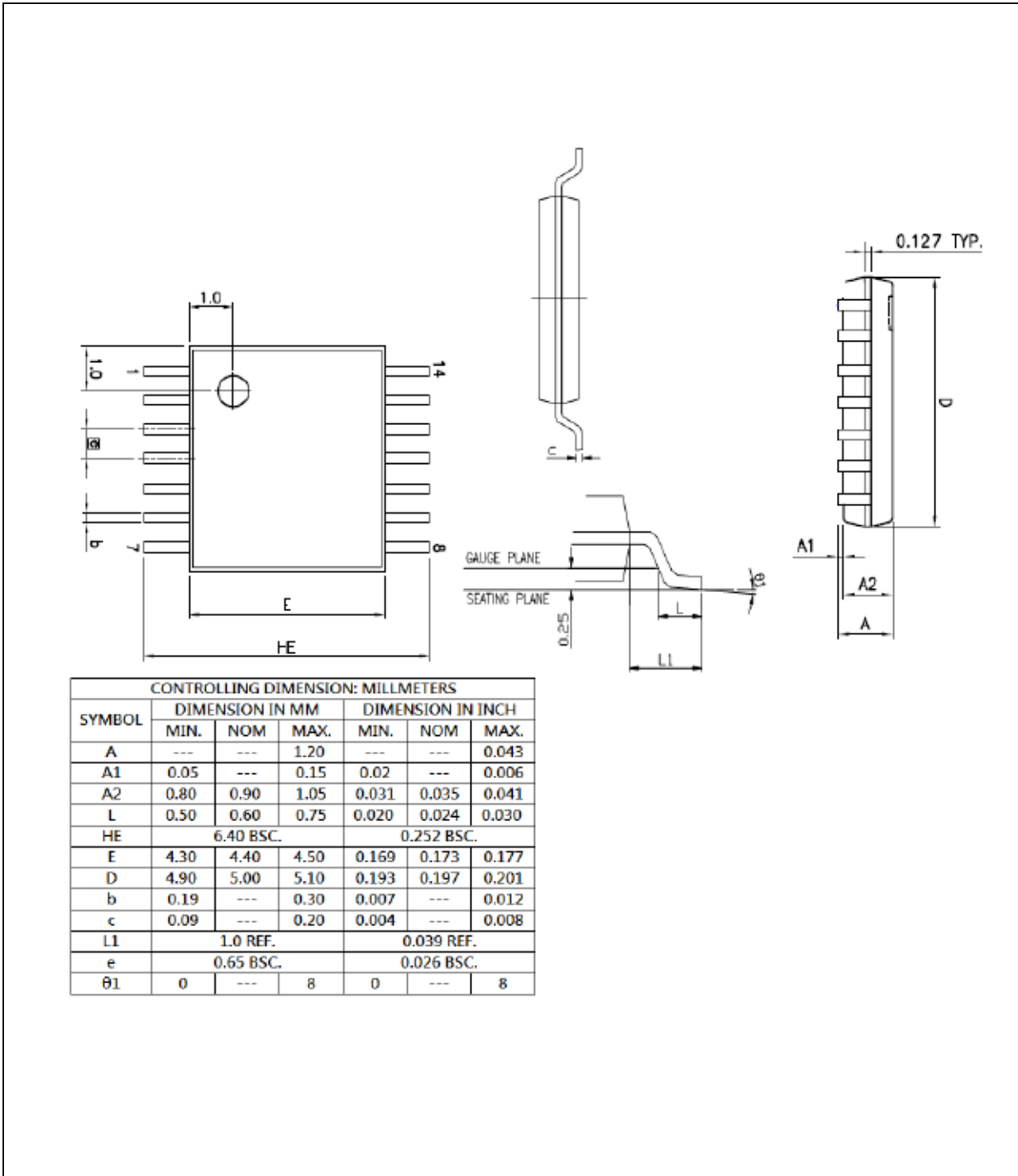
Figure 9.1-1 TSSOP-14 Package Dimension
