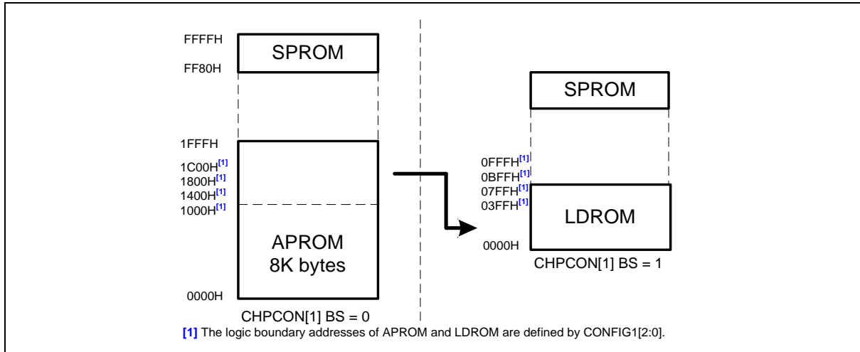
Figure 6.1-1 MS51 8KB Flash series Program Memory Map and Boot Select
