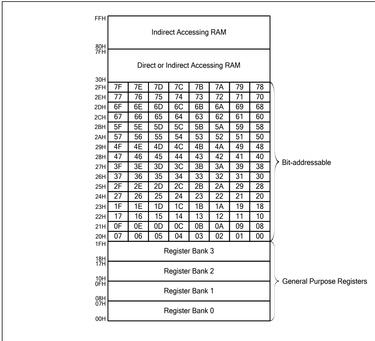
Figure 6.1-5 Internal 256 Bytes RAM Addressing
