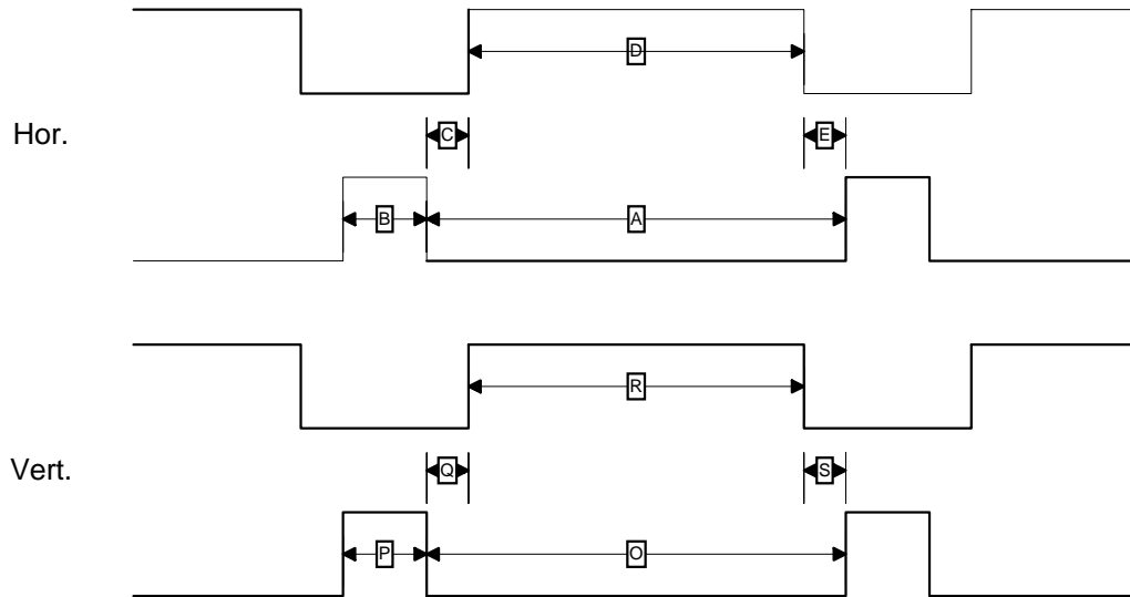
MTV112M Self-Test Pattern Timing (8MHz)
