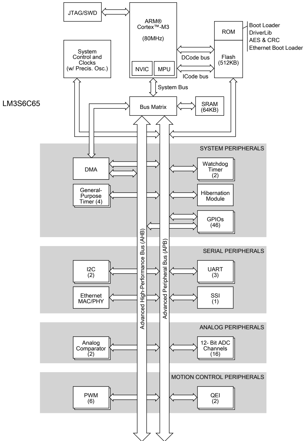
Figure 1-1. Stellaris LM3S6C65 Microcontroller High-Level Block Diagram
