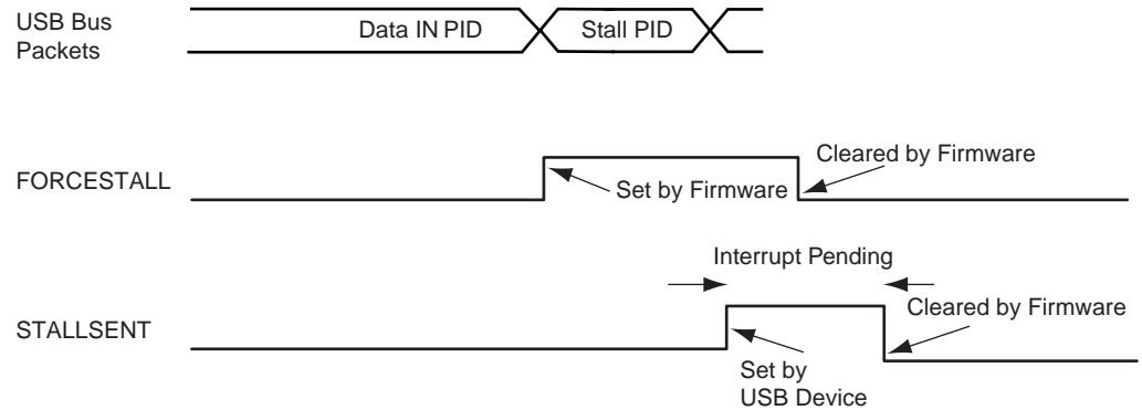
Figure 38-13. Stall Handshake (Data IN Transfer)
