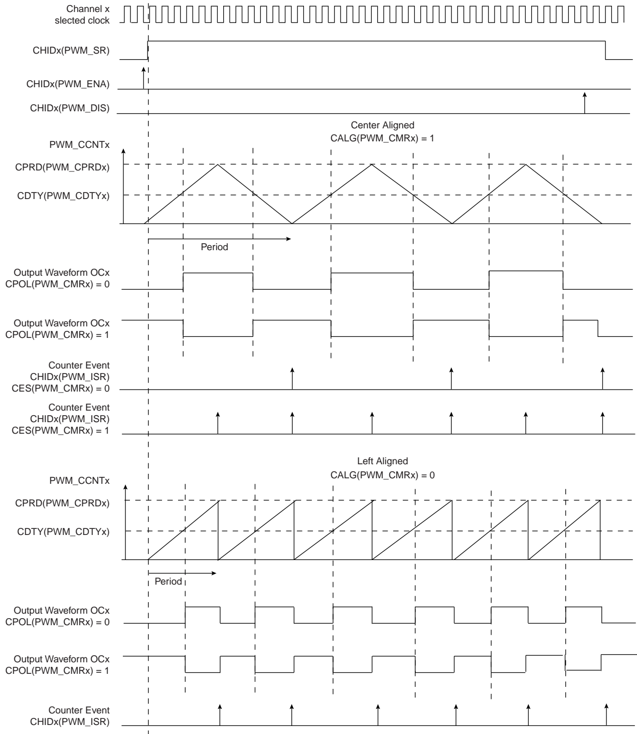
Figure 37-5. Waveform Properties
