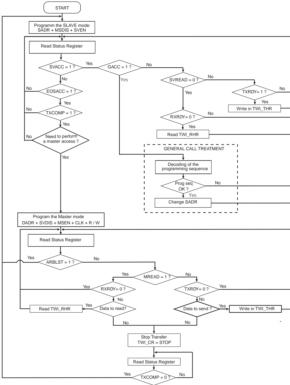
Figure 32-23. Multi-master Flowchart
