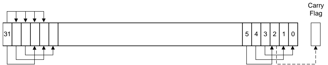
Figure 11-7. ASR #3
