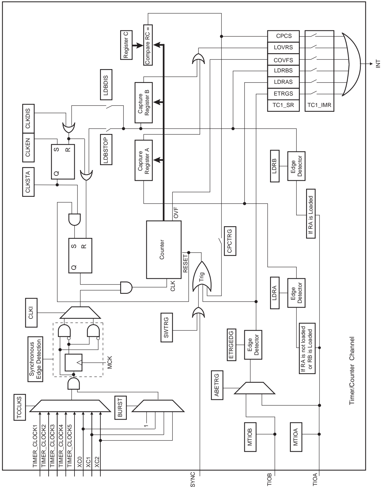
Figure 35-5. Capture Mode
