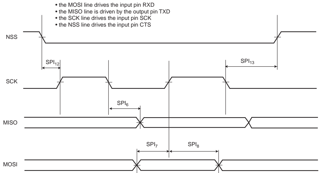
Figure 42-27. USART SPI Slave Mode: (Mode 1 or 2)
