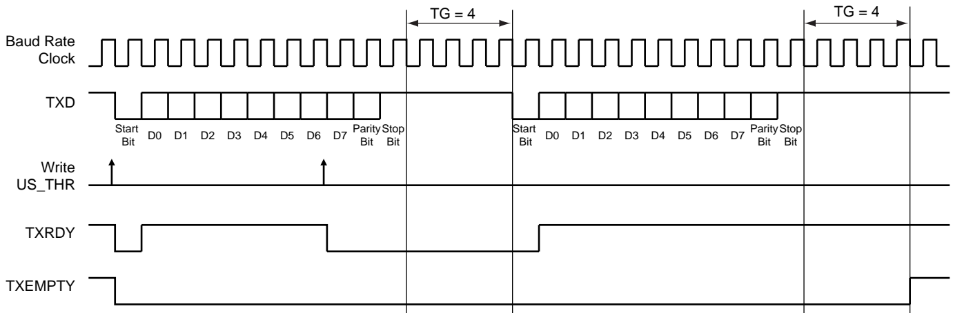
Figure 34-23. Timeguard Operations
