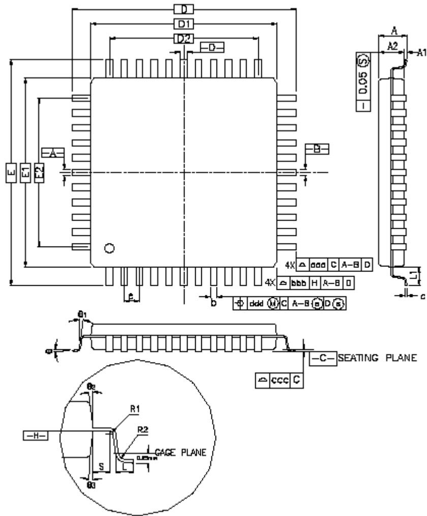
Figure 43-4. 64-lead LQFP Package Drawing
