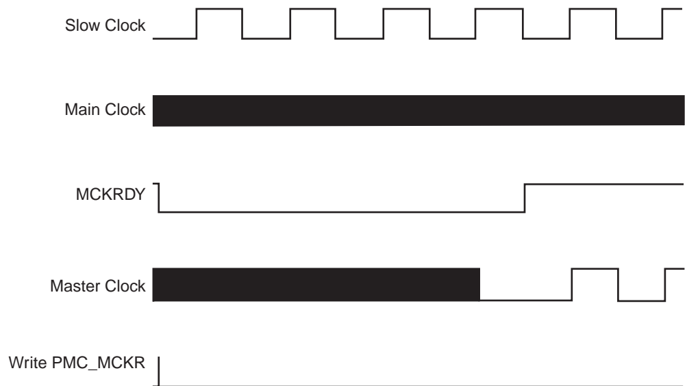
Figure 27-10. Switch Master Clock from Main Clock to Slow Clock
