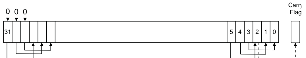
Figure 11-8. LSR #3
