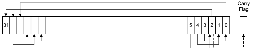
Figure 11-10. ROR #3
