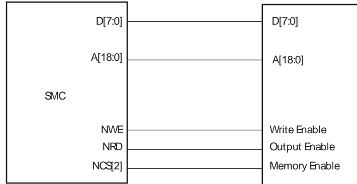
Figure 25-2. Memory Connection for an 8-bit Data Bus
