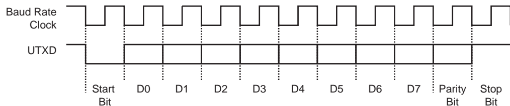
Figure 33-9. Character Transmission
