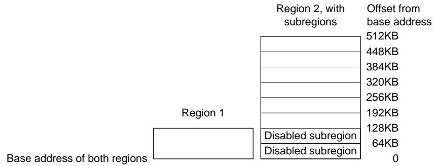
Figure 11-12. SRD Use
