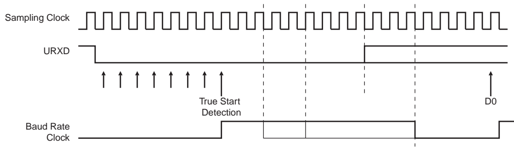
Figure 33-4. Character Reception
