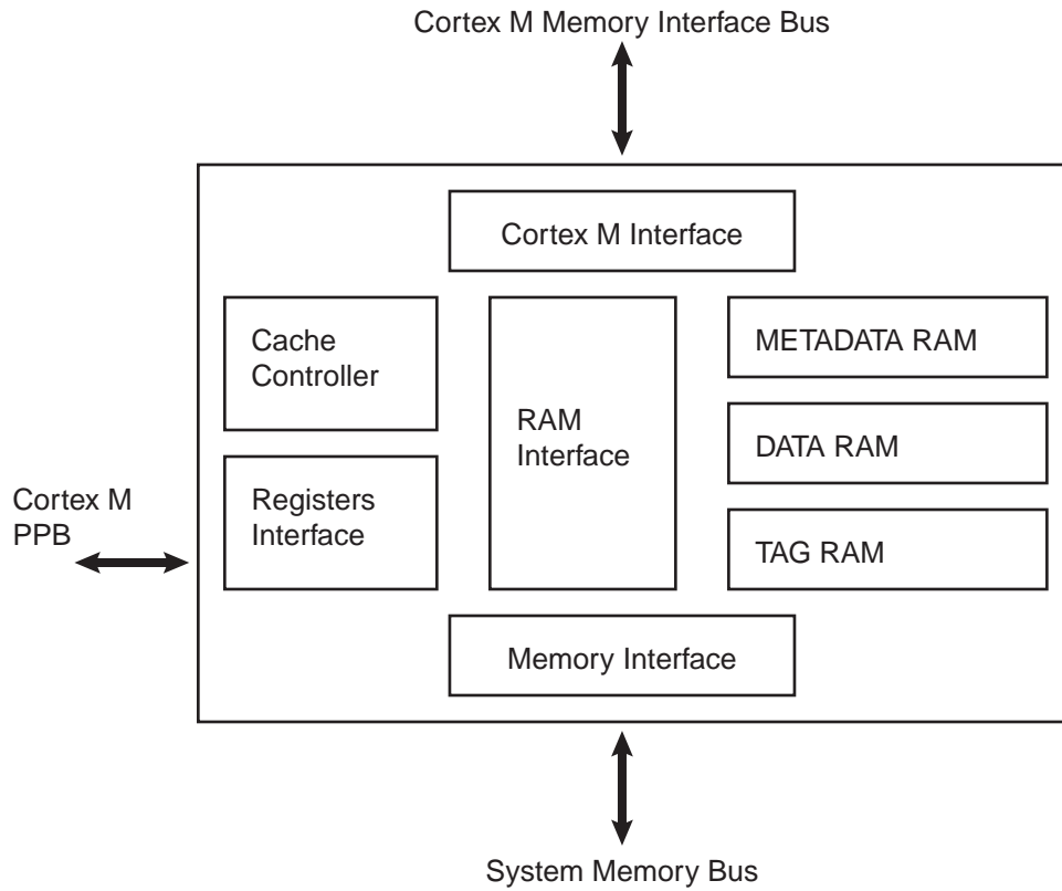
Figure 21-1. Block Diagram
