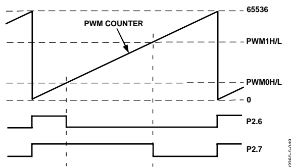
Figure 50. PWM Mode 3
