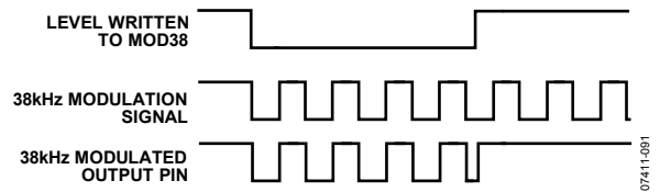
Figure 96. 38 kHz Modulation
