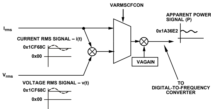
Figure 54. Apparent Power Signal Processing
