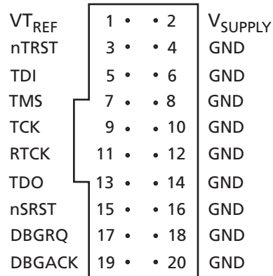
Figure 8-2 · JTAG 20-Pin Connector Pinout
