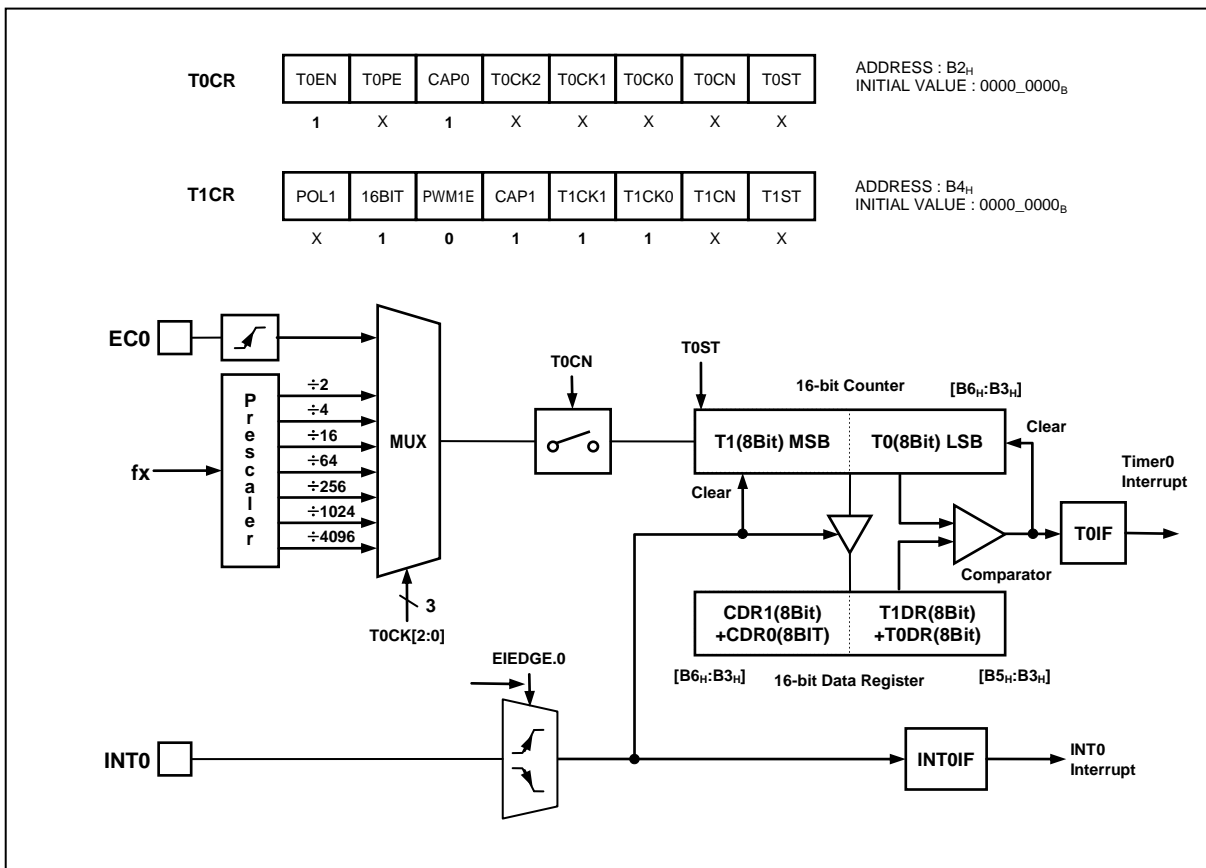
Figure 11-14 16-bit Capture Mode of Timer 0, 1
