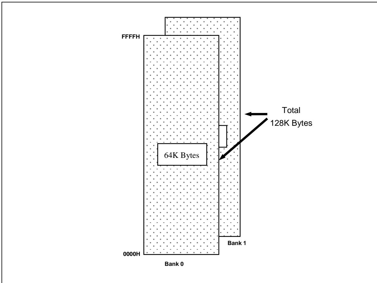
Figure 8-1 Program memory
