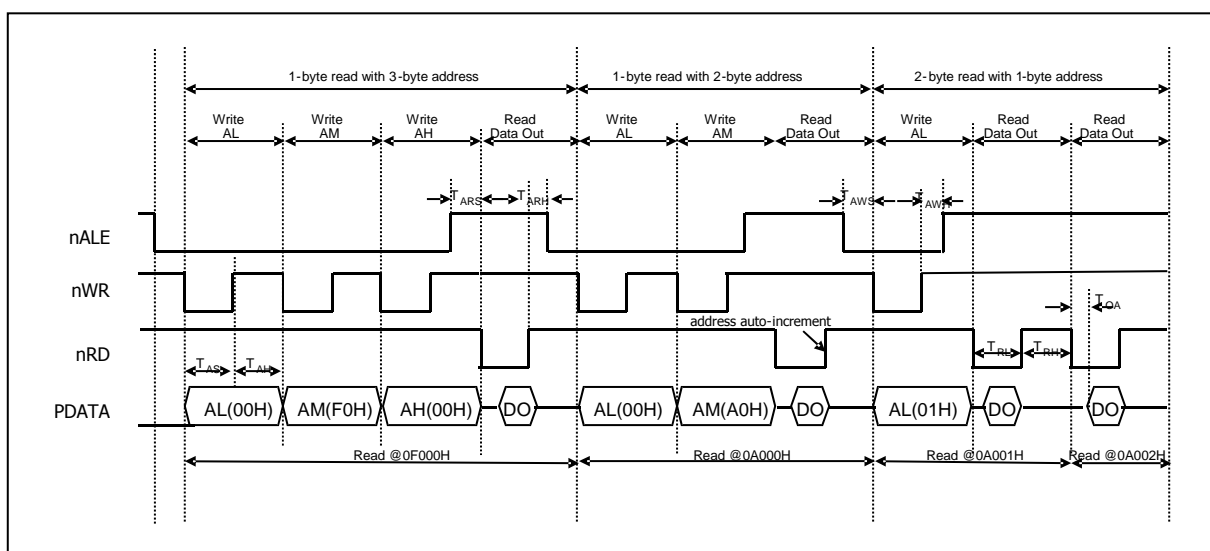
Figure 15-8 Parallel Byte Read Timing of Program Memory
