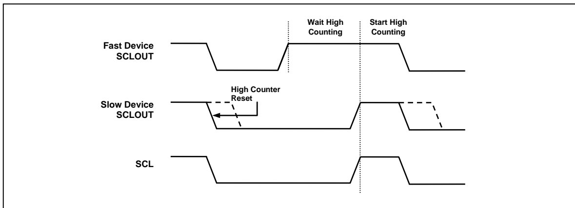
Figure 11-40 Clock Synchronization during Arbitration Procedure
