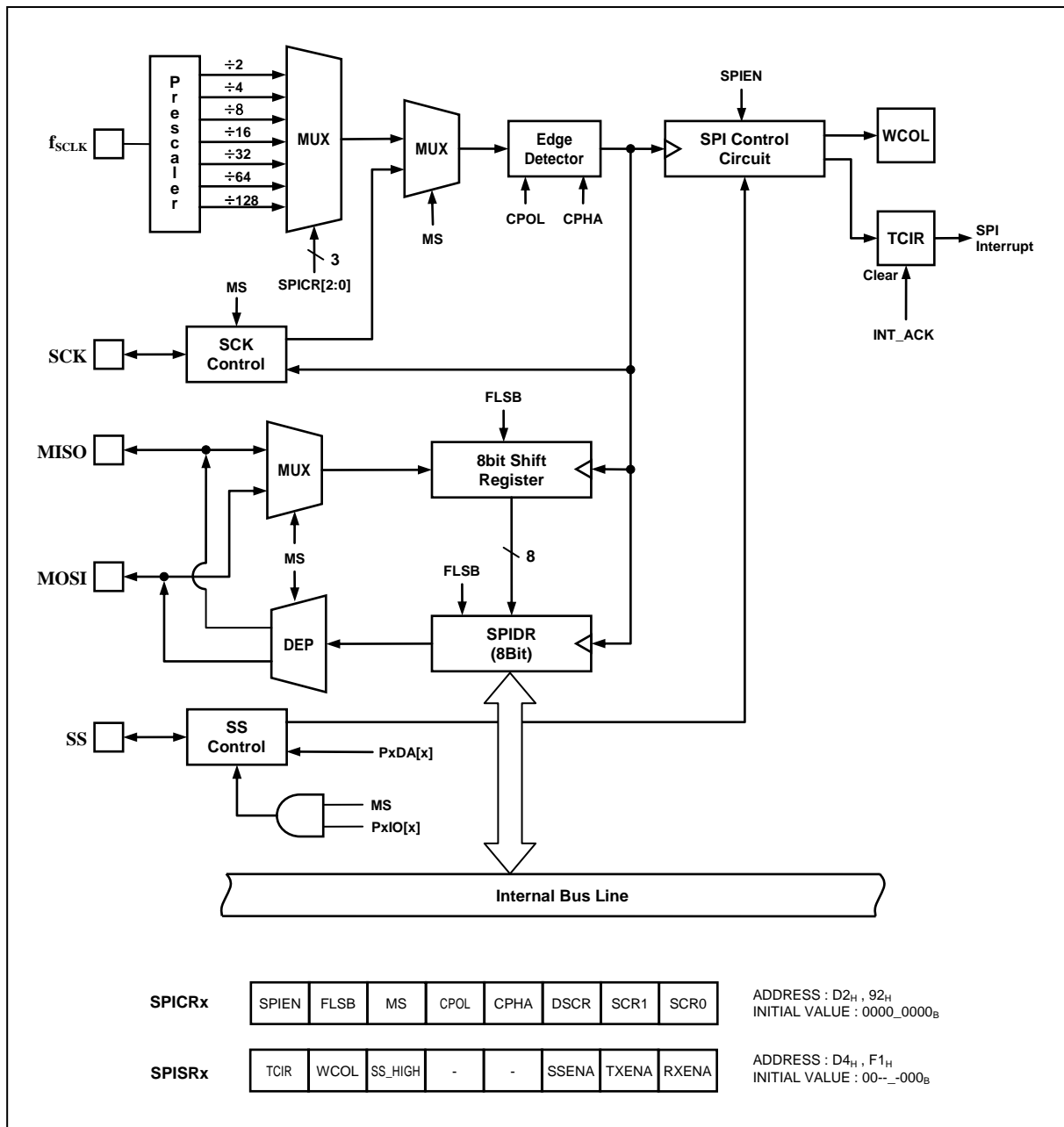
Figure 11-32 SPI Block Diagram
