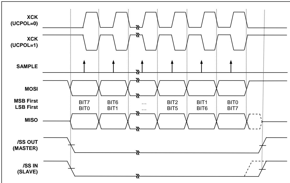
Figure 11-30 SPI Clock Formats when UCPHA=0
