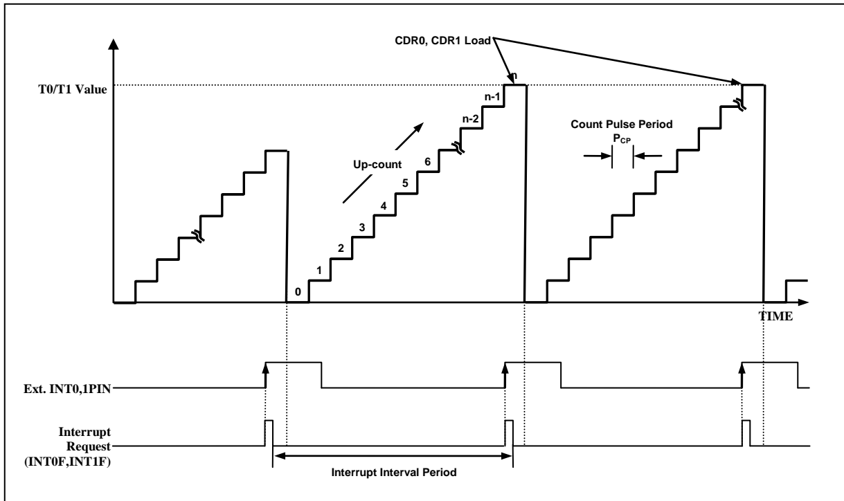
Figure 11-12 Input Capture Mode Operation of Timer 0, 1
