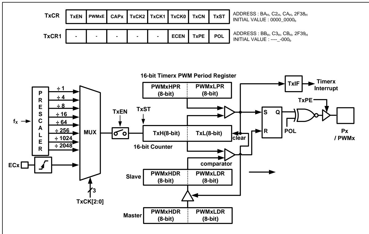
Figure 11-20 PWM Mode
