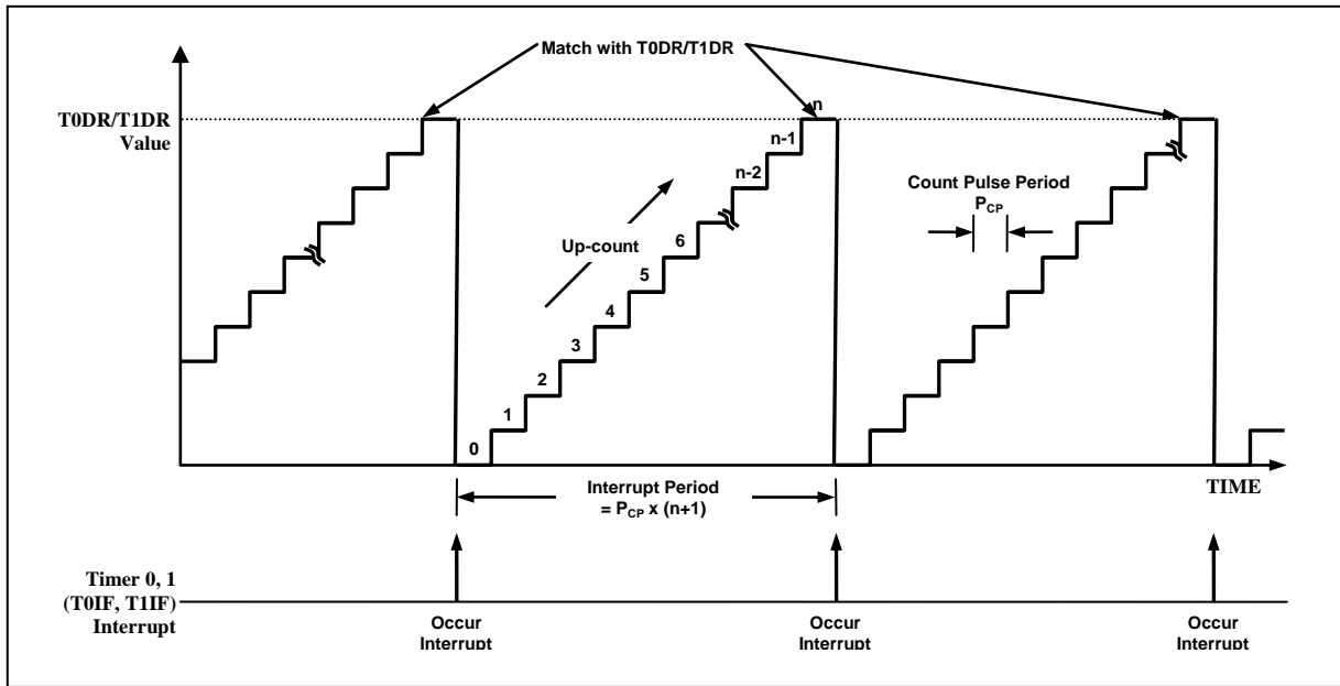
Figure 11-8 Timer/Event Counter0, 1 Example
