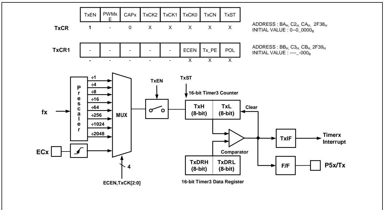
Figure 11-18 Timerx 16-bit Mode Block Diagram
