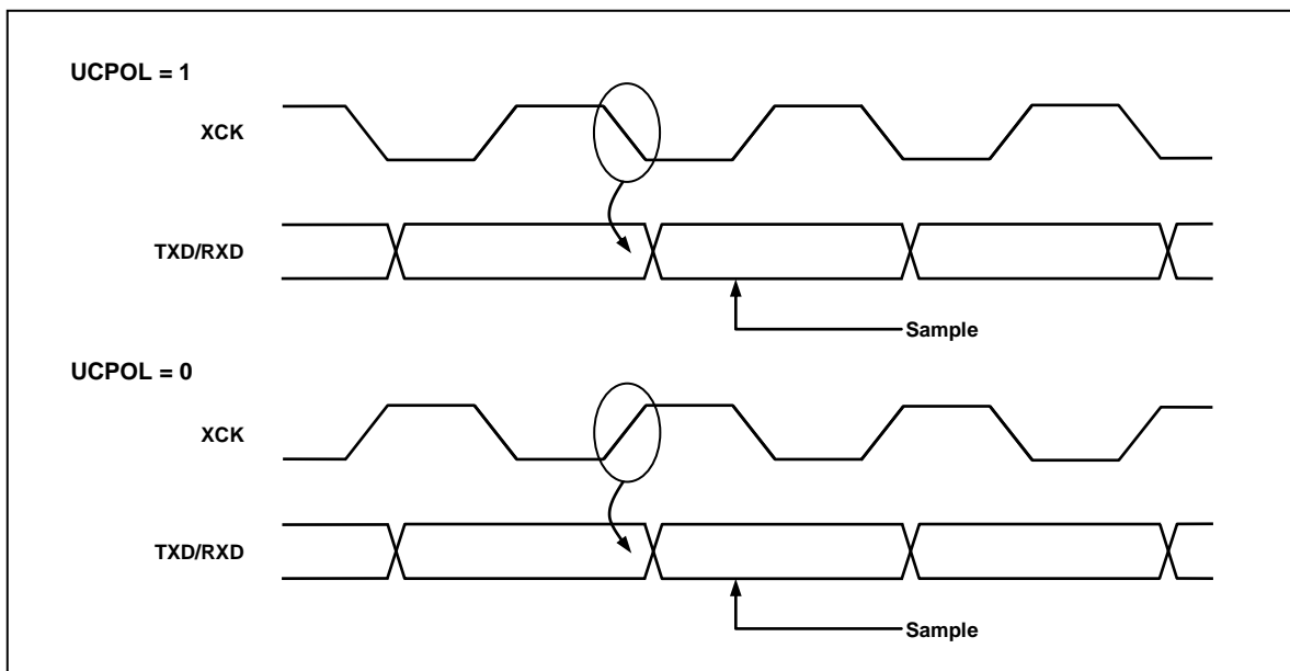
Figure 11-25 Synchronous Mode XCKn Timing
