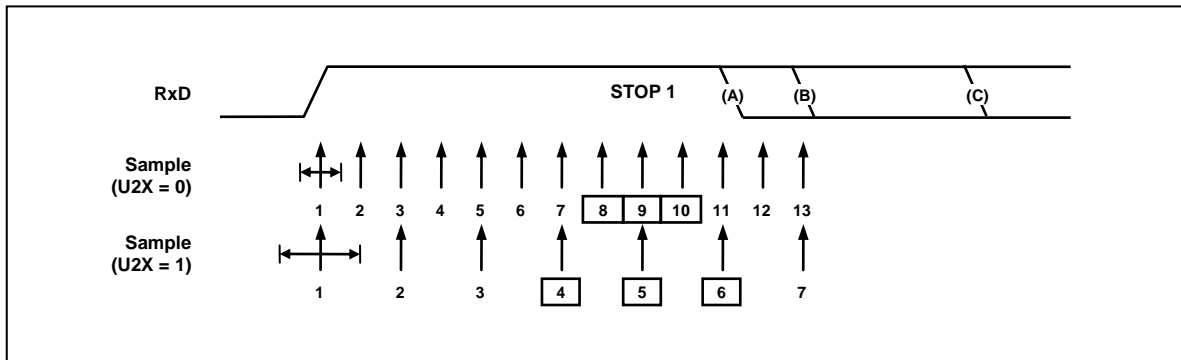
Figure 11-29 Stop Bit Sampling and Next Start Bit Sampling
