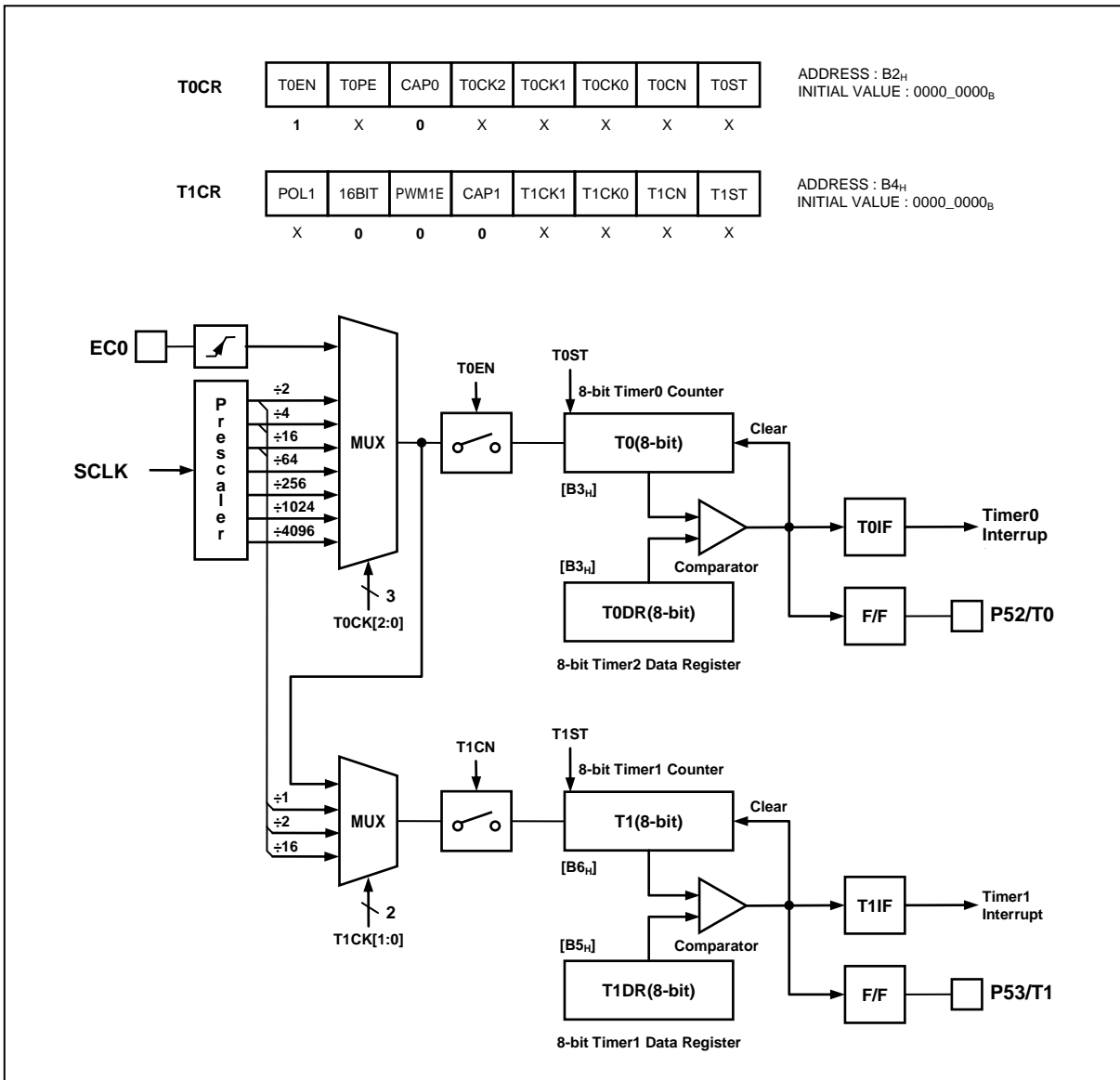
Figure 11-7 8 Bit Timer/Event Counter2, 3 Block Diagram
