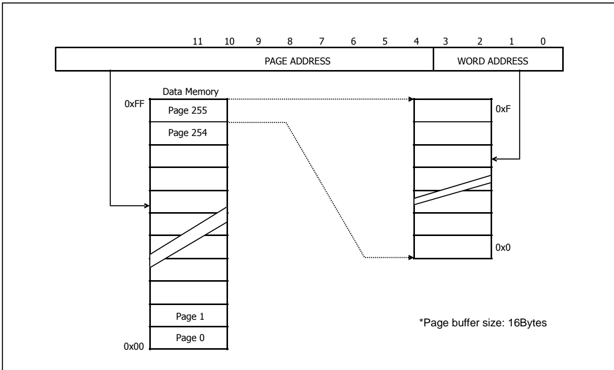
Figure 15-4 Address configuration of data EEPROM
