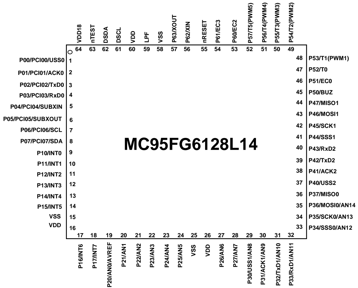
Figure 3-5 MC95FG0128 64 pin LQFP14 assignment
