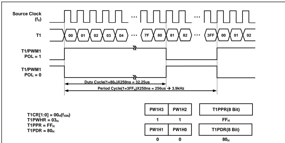
Figure 11-16 Example of PWM at 4MHz
