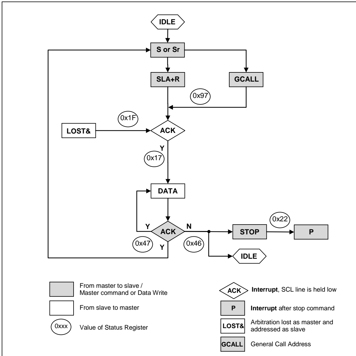
Figure 11-44 Formats and States in the Slave Transmitter Mode
