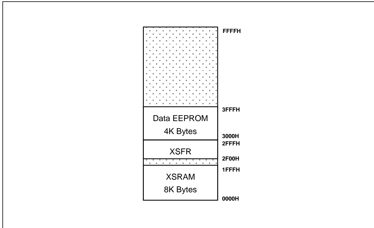
Figure 8-4 XDATA memory area
