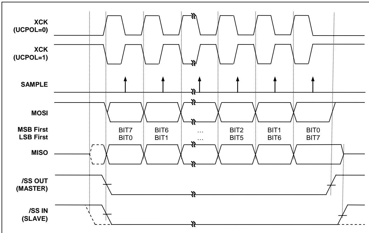
Figure 11-31 SPI Clock Formats when UCPHA=1
