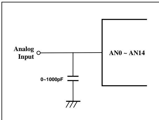
Figure 11-47 A/D Analog Input Pin Connecting Capacitor
