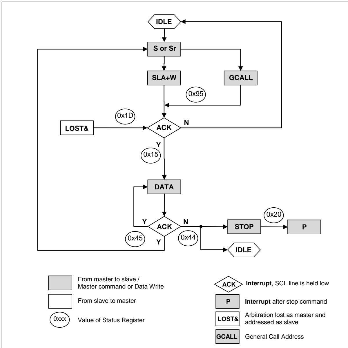
Figure 11-45 Formats and States in the Slave Receiver Mode
