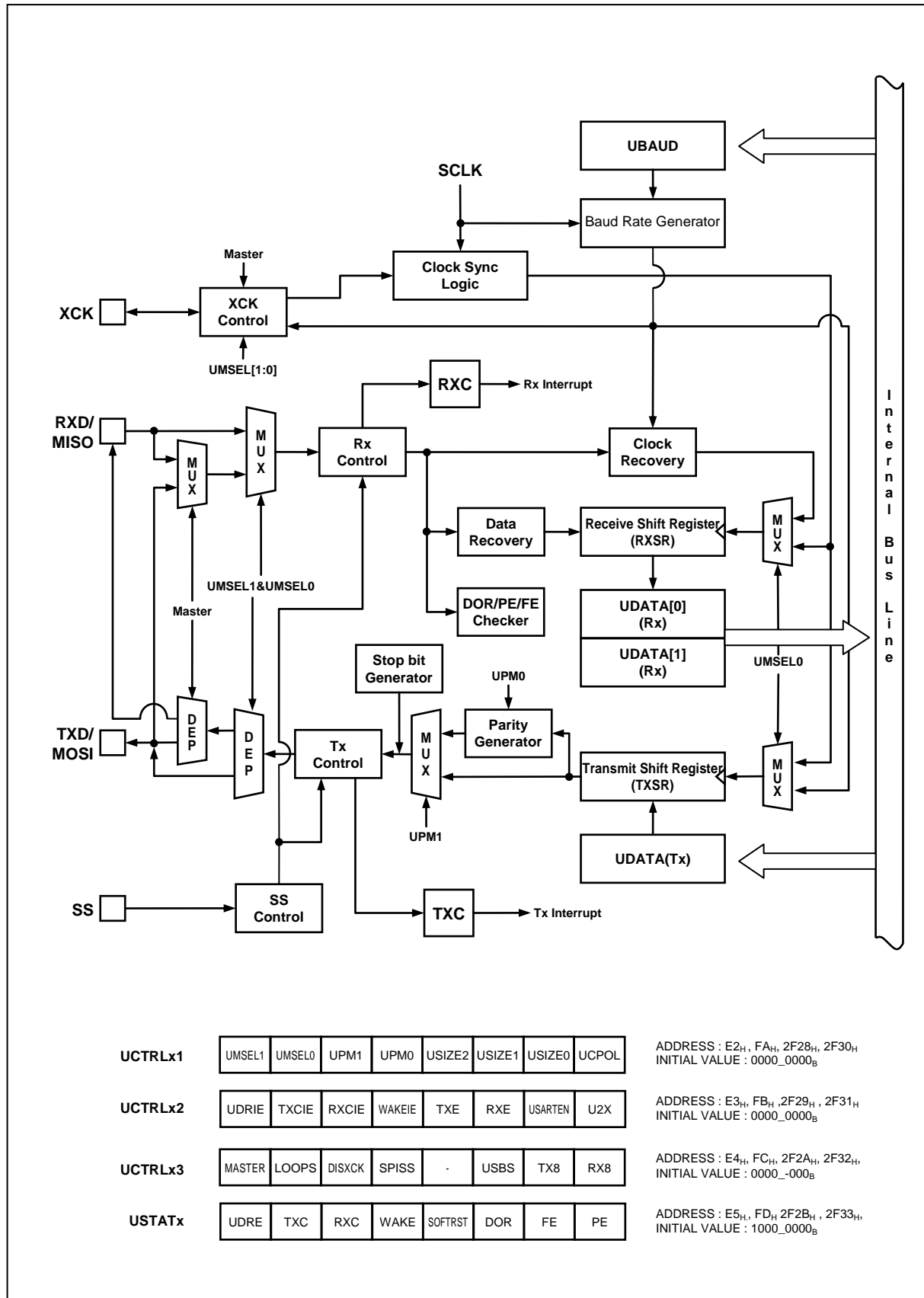
Figure 11-23 USART Block Diagram
