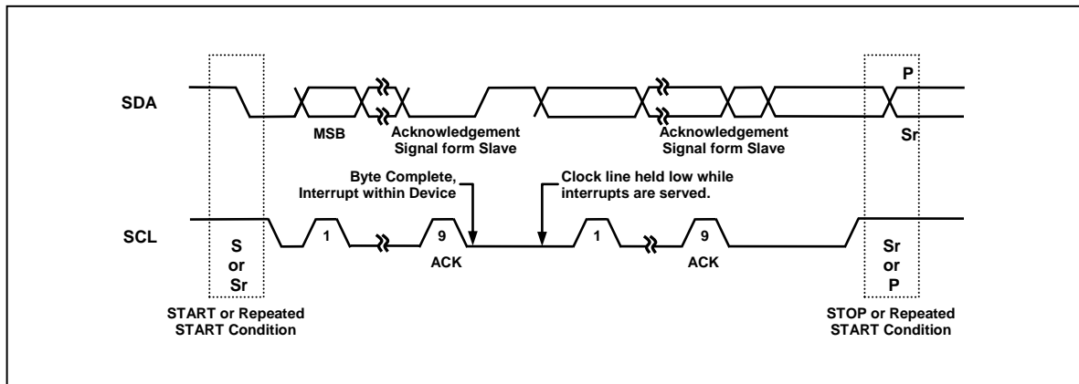
Figure 11-38 Data Transfer on the I 2 C-Bus
