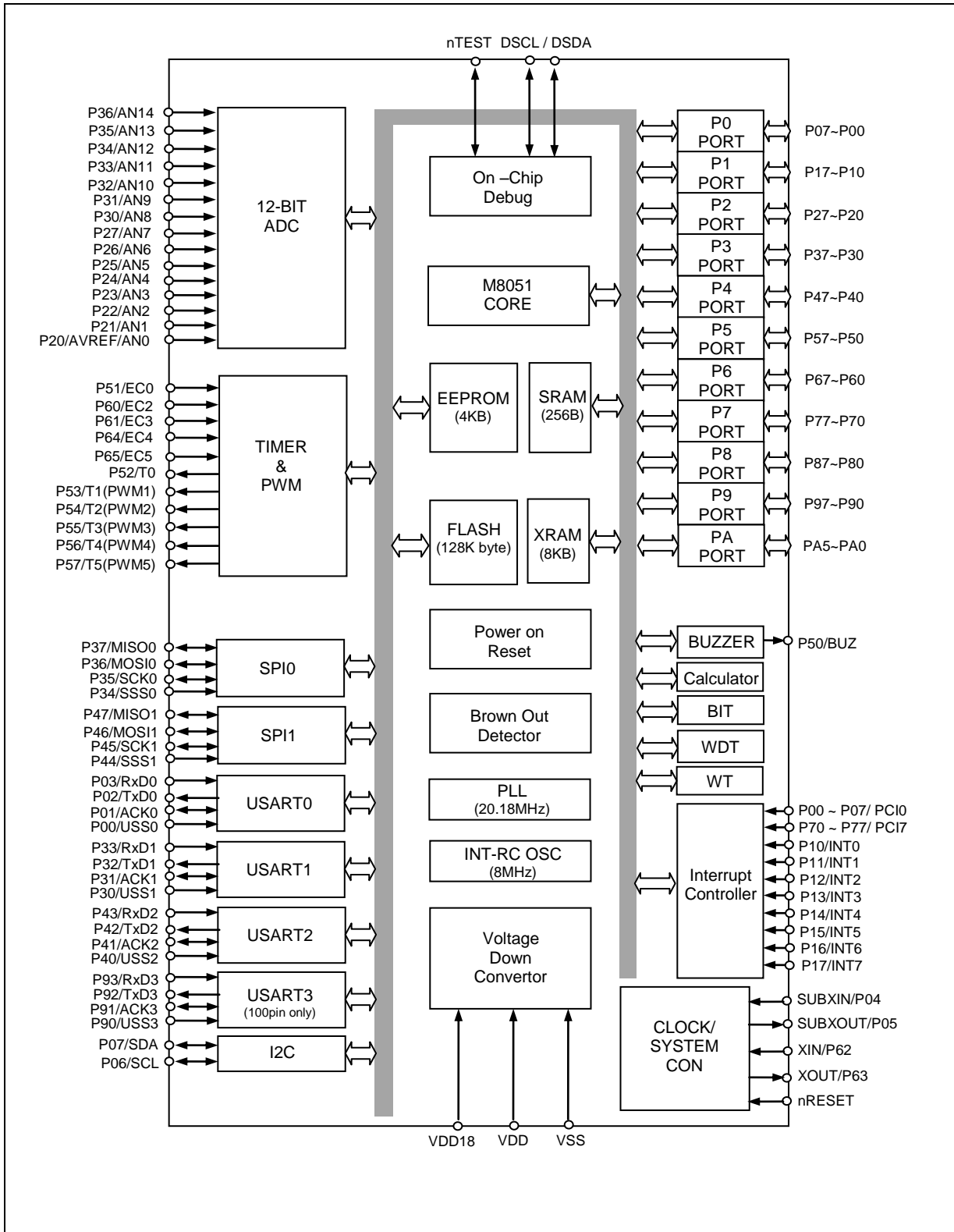
Figure 2-1 MC95FG0128 block diagram
