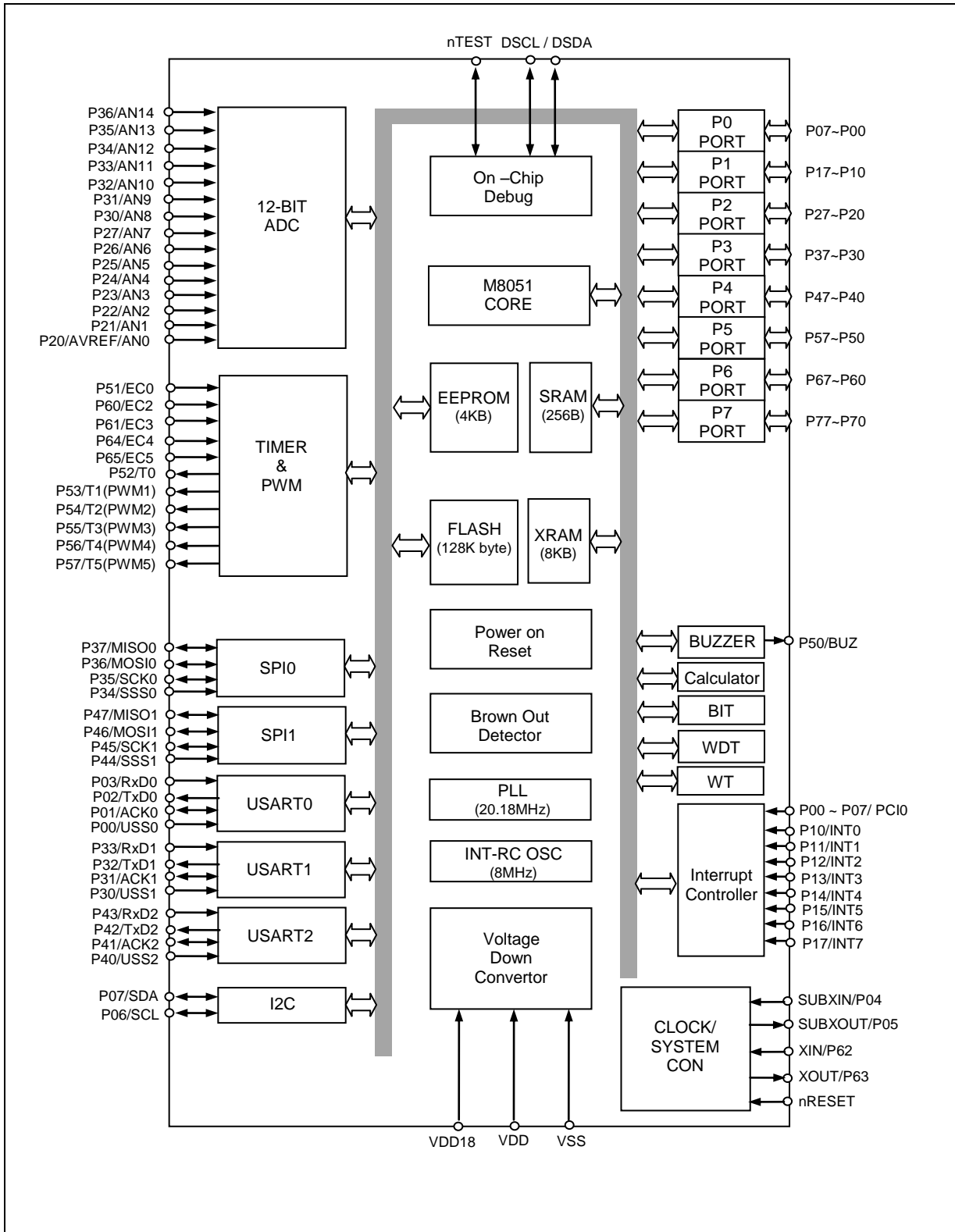
Figure 2-2 MC95FG8128 block diagram
