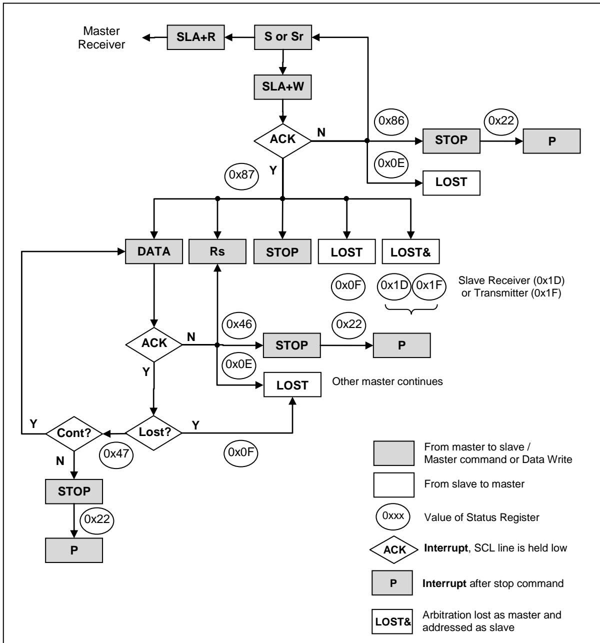
Figure 11-42 Formats and States in the Master Transmitter Mode
