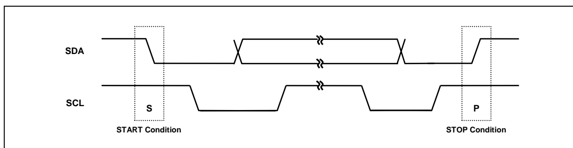
Figure 11-37 START and STOP Condition
