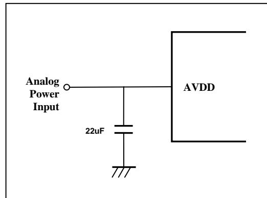
Figure 11-48 A/D Power (AVDD) Pin Connecting Capacitor
