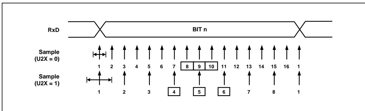
Figure 11-28 Sampling of Data and Parity Bit
