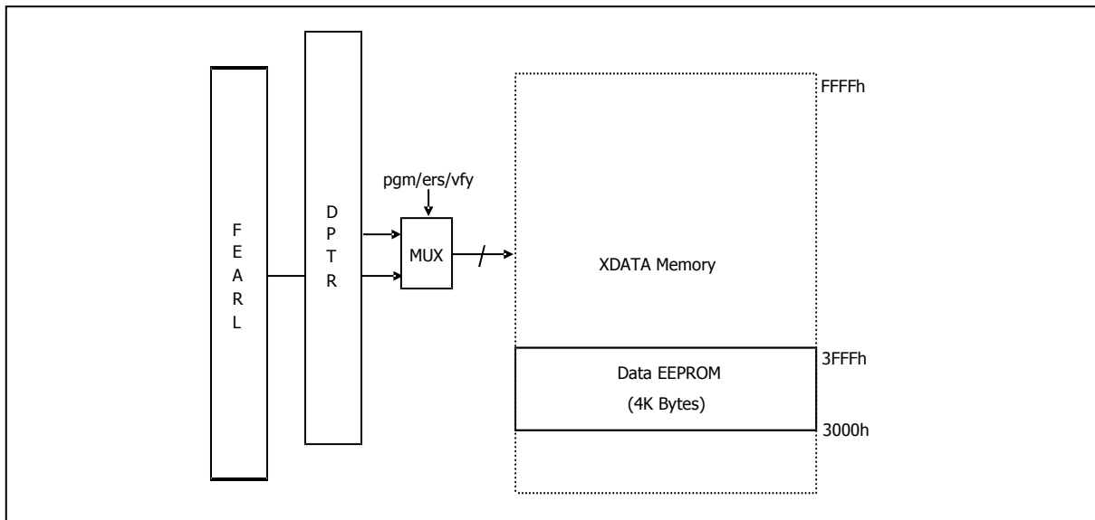
Figure 15-3 Data EEPROM memory map
