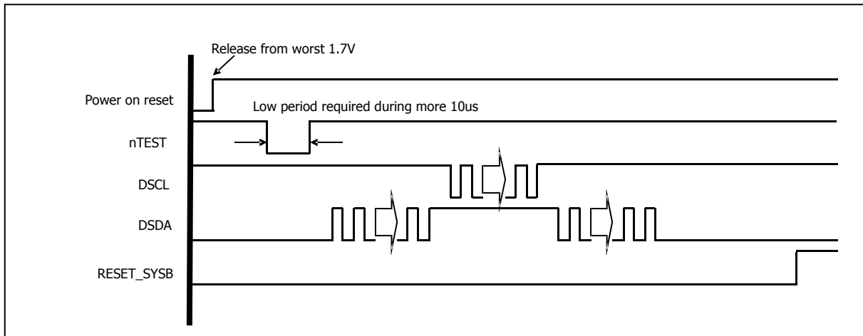
Figure 15-10 ISP mode
