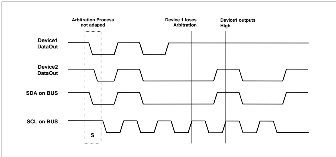
Figure 11-41 Arbitration Procedure of Two Masters
