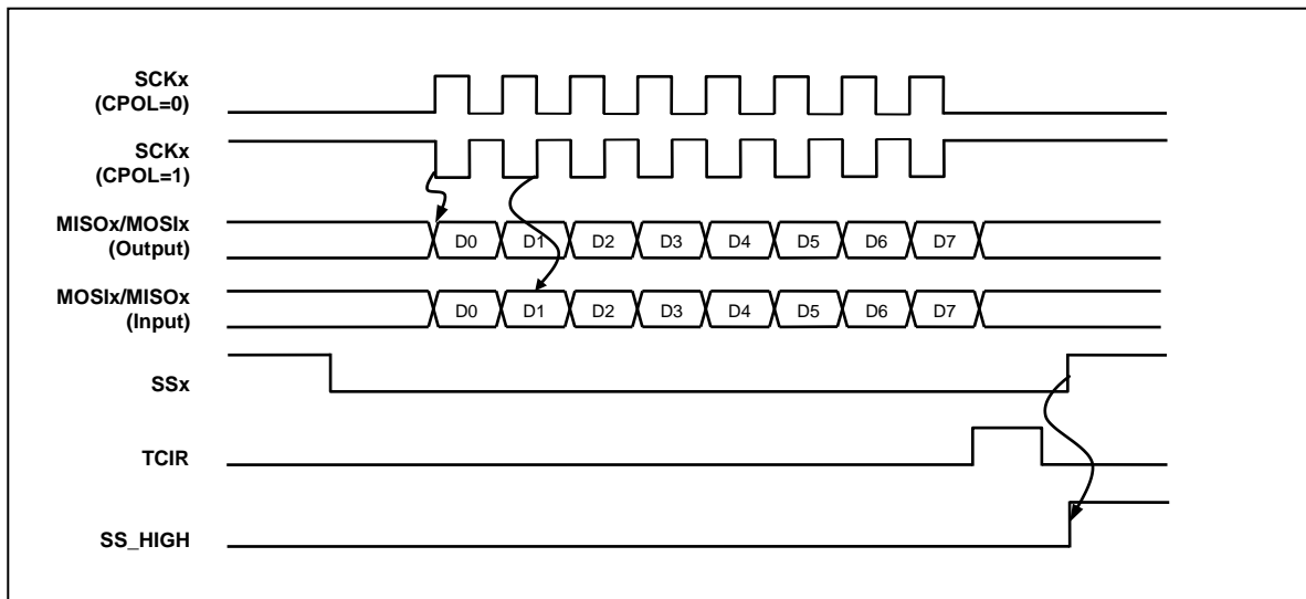
Figure 11-34 SPI Transmit/Receive Timing Diagram at CPHA = 1
