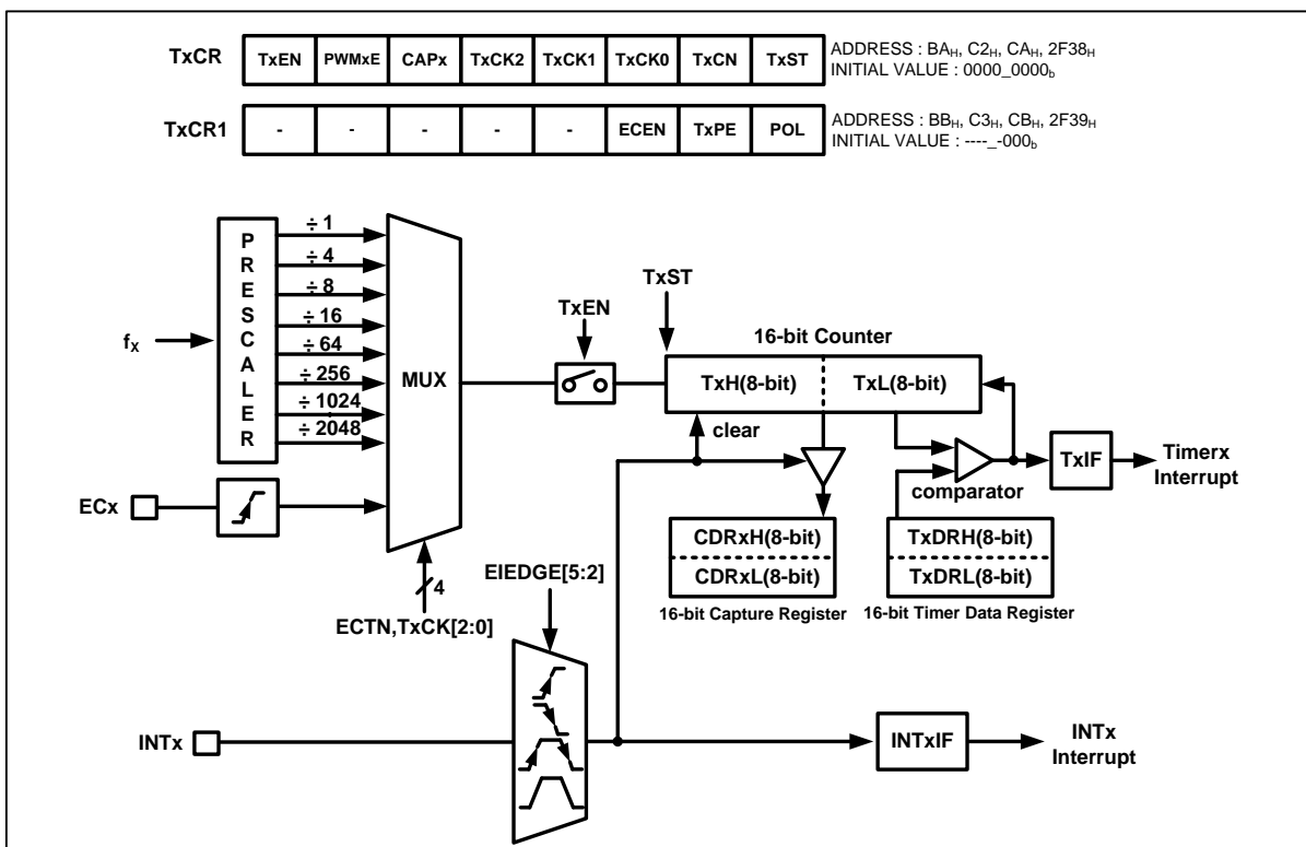
Figure 11-19 16-bit Capture Mode of Timer x
