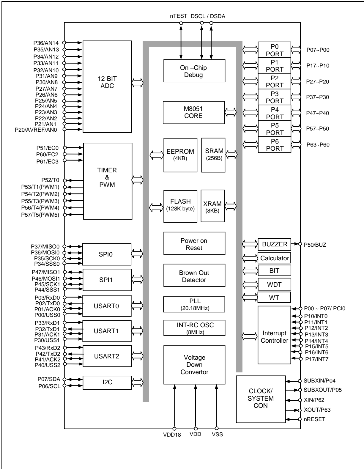
Figure 2-3 MC95FG6128 block diagram
