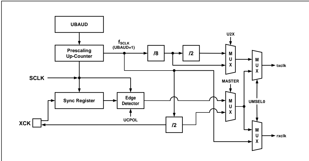
Figure 11-24 Clock Generation Block Diagram
