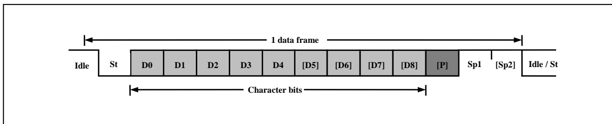
Figure 11-26 frame format
