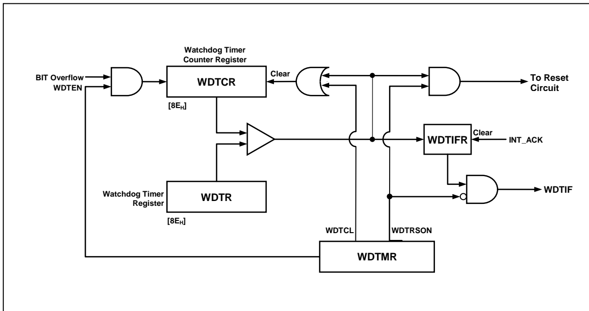
Figure 11-4 WDT Block Diagram
