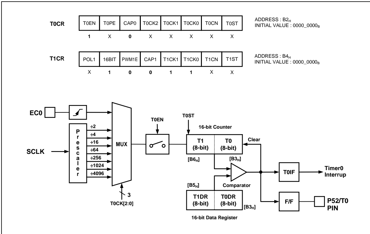
Figure 11-10 16 Bit Timer/Event Counter0, 1 Block Diagram
