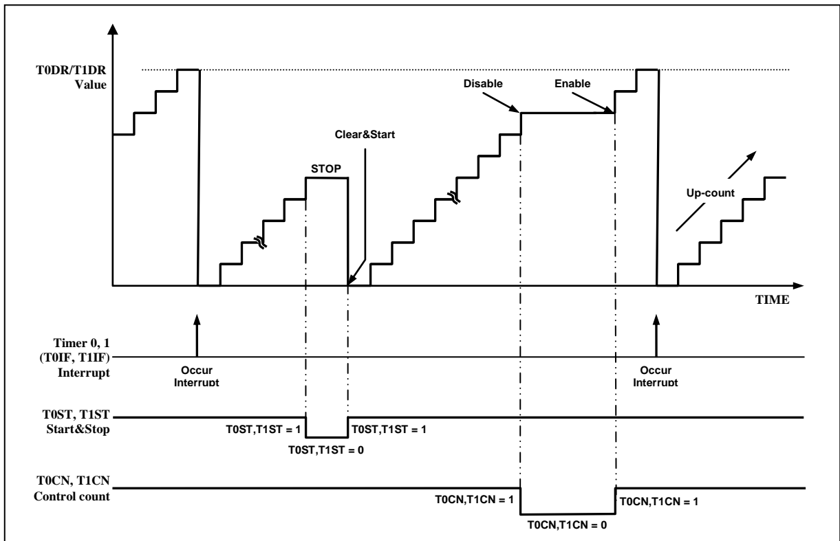
Figure 11-9 Operation Example of Timer/Event Counter0, 1
