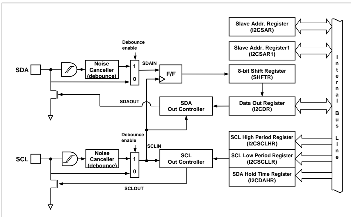
Figure 11-35 I 2 C Block Diagram
