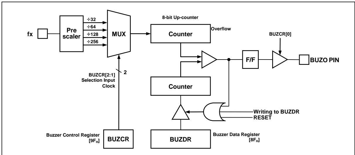
Figure 11-22 Buzzer Driver Block Diagram
