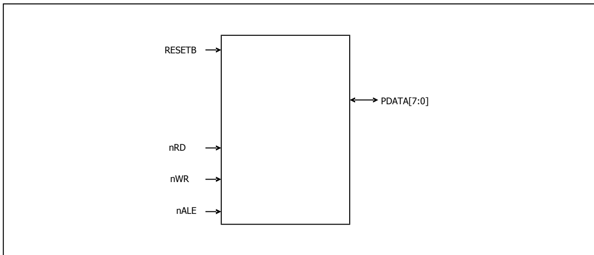
Figure 15-7 Pin diagram for parallel programming
