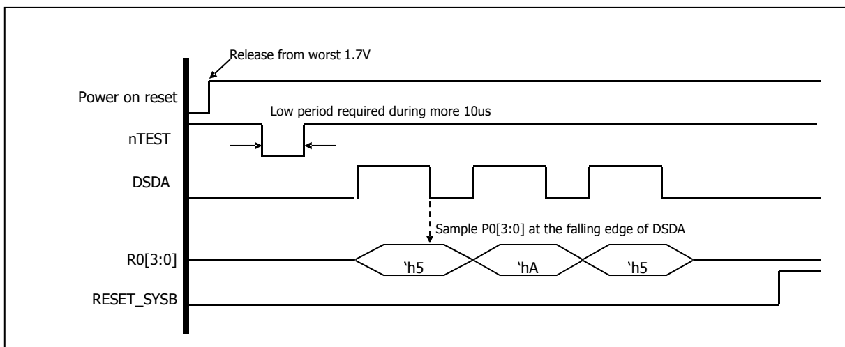
Figure 15-11 Byte-parallel mode
