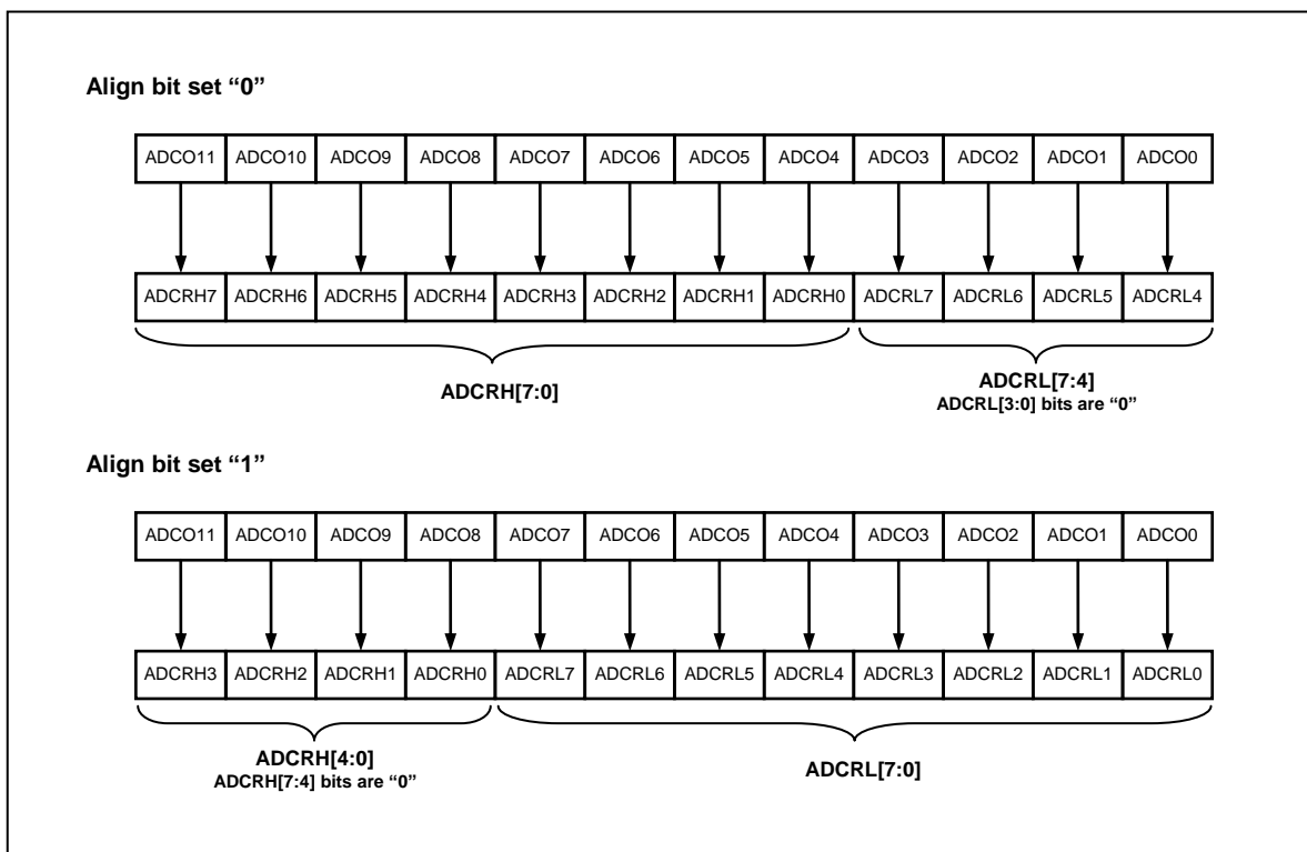
Figure 11-49 ADC Operation for Align bit
