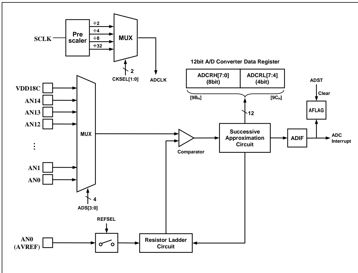
Figure 11-46 ADC Block Diagram
