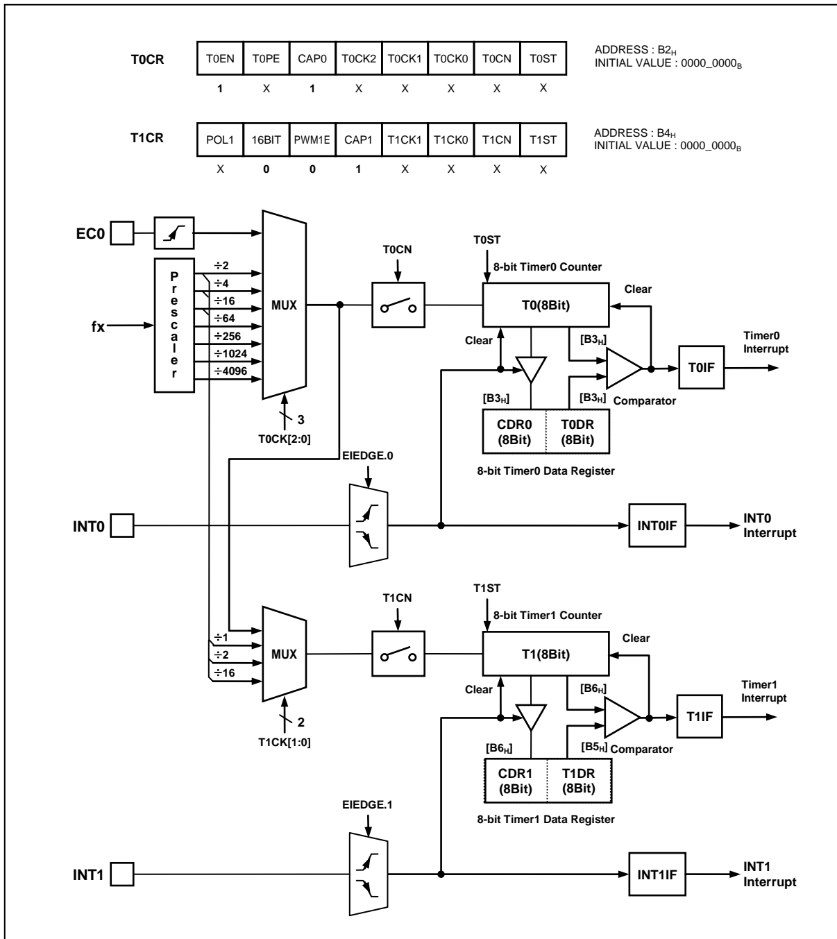
Figure 11-11 8-bit Capture Mode for Timer0, 1
