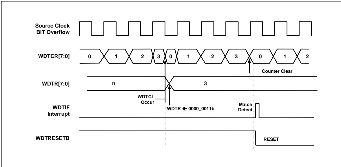
Figure 11-5 WDT Interrupt Timing Waveform
