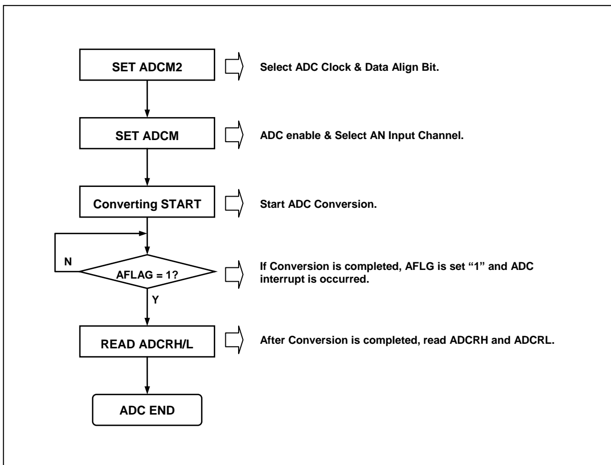
Figure 11-50 Converter Operation Flow
