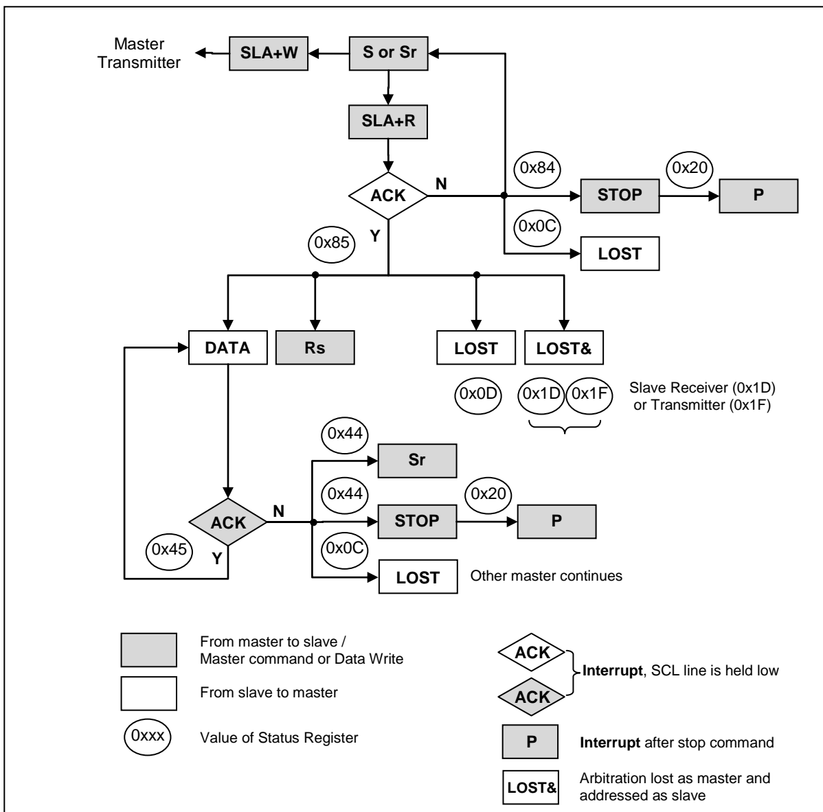
Figure 11-43 Formats and States in the Master Receiver Mode
