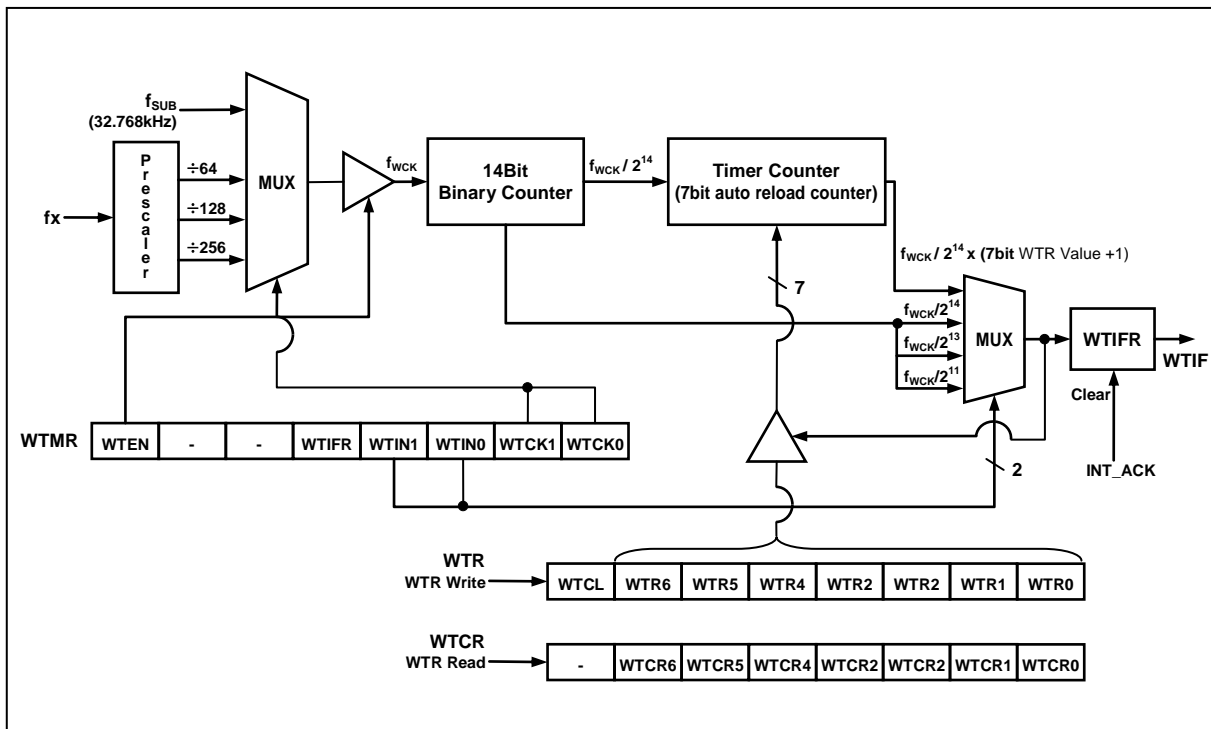
Figure 11-6 Watch Timer Block Diagram
