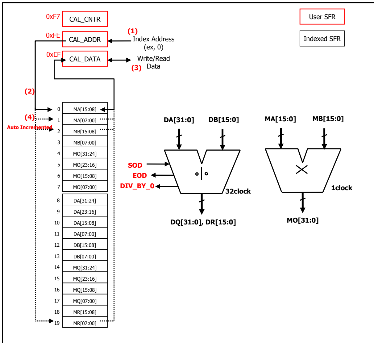
Figure 11-51 Calculator Block Diagram
