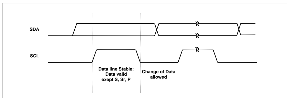
Figure 11-36 Bit Transfer on the I 2 C-Bus
