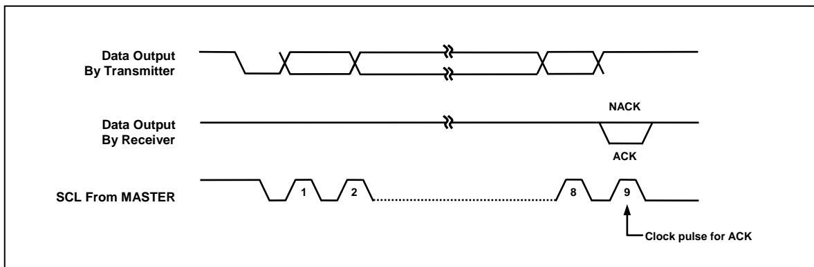
Figure 11-39 Acknowledge on the I 2 C-Bus
