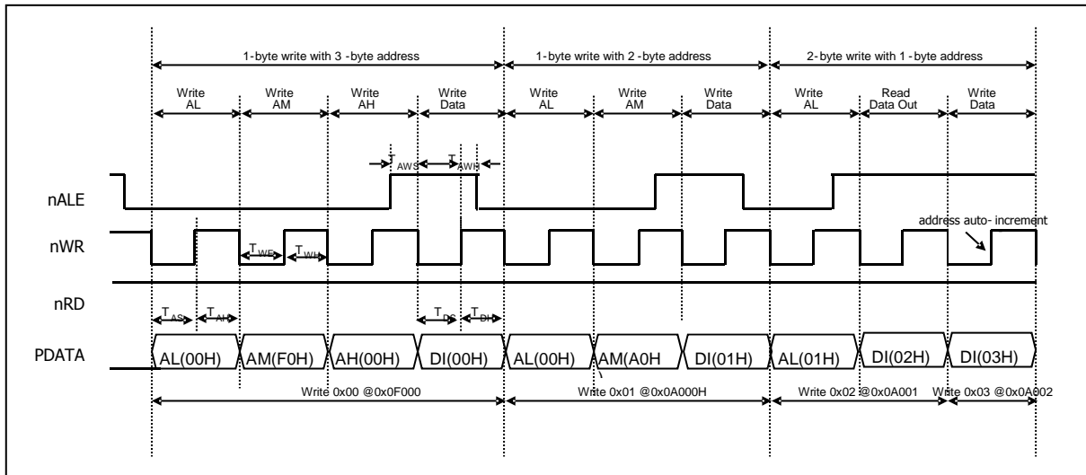
Figure 15-9 Parallel Byte Write Timing of Program Memory
