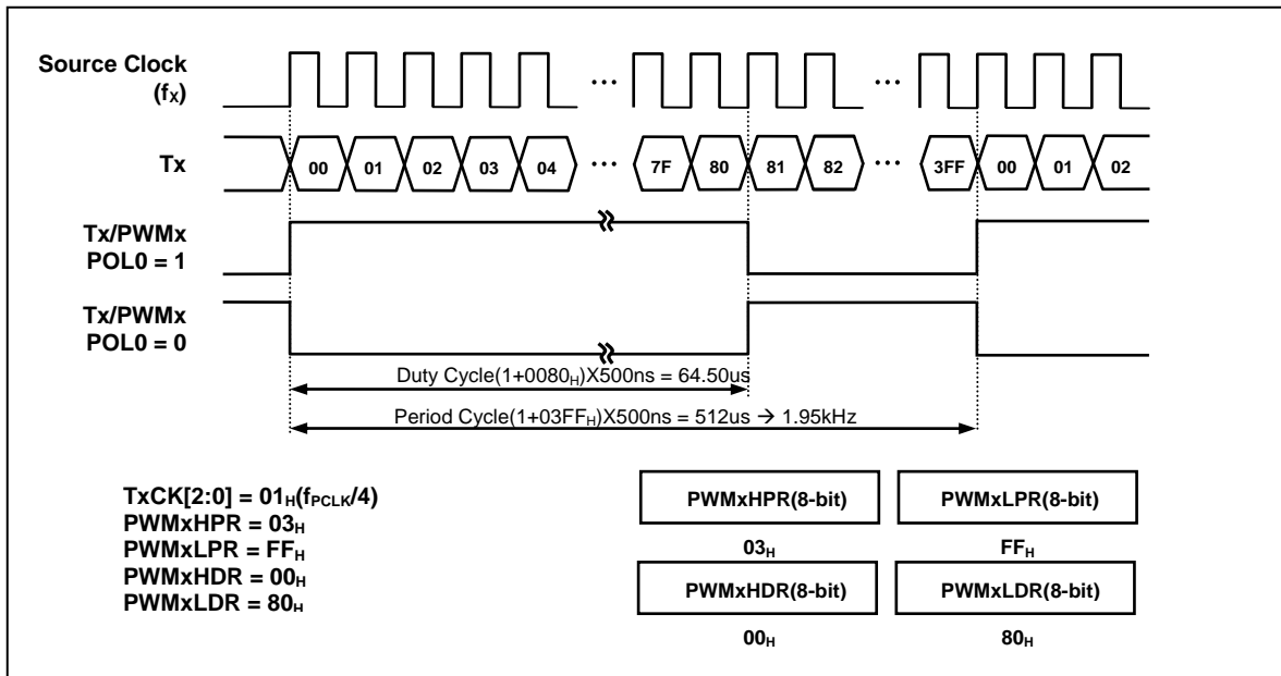
Figure 11-21 Example of PWM at 8MHz
