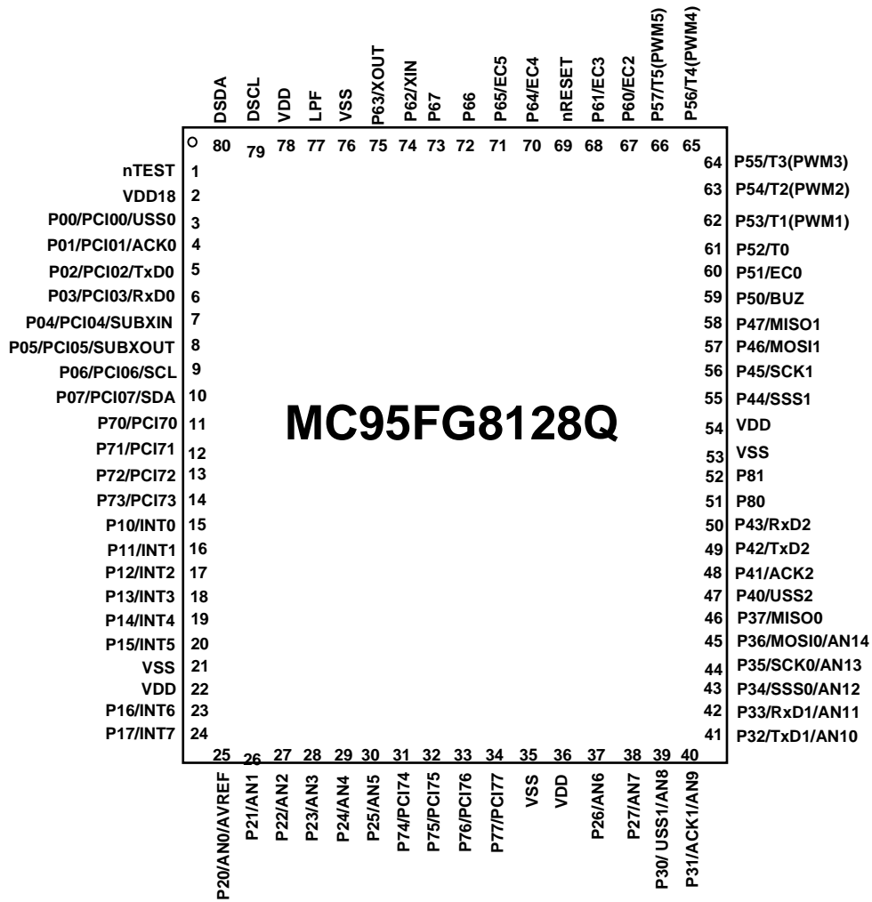
Figure 3-3 MC95FG0128 80 Pin MQFP assignment
