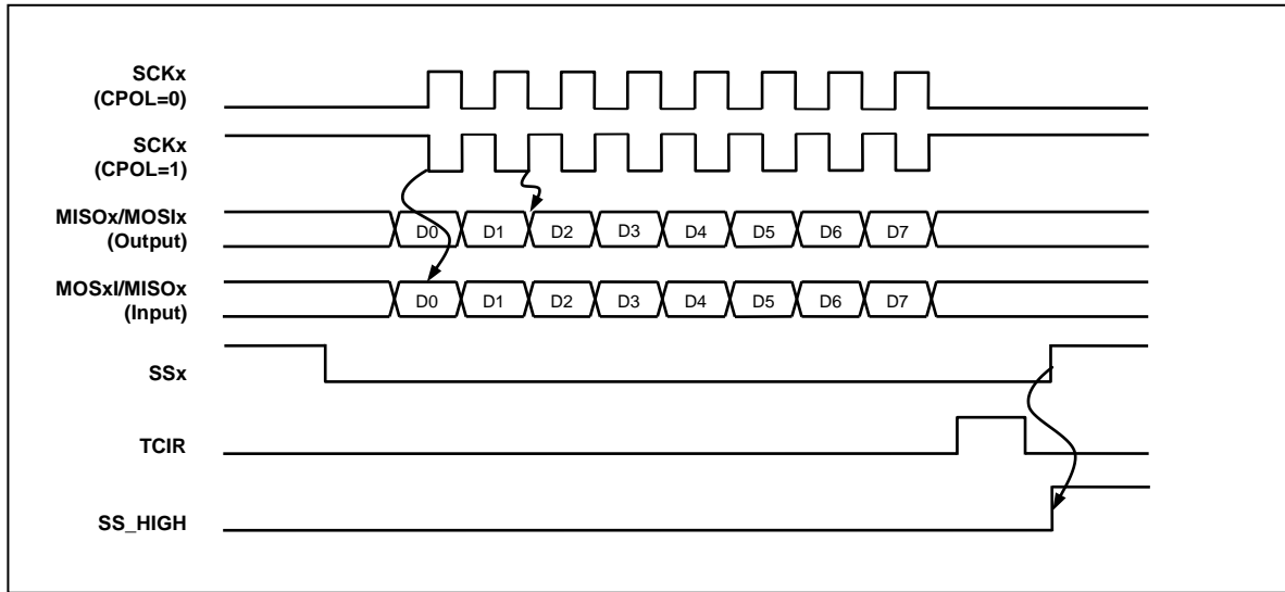
Figure 11-33 SPI Transmit/Receive Timing Diagram at CPHA = 0
