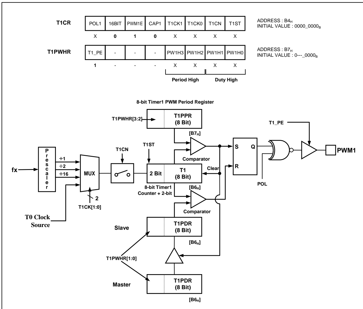
Figure 11-15 PWM Mode
