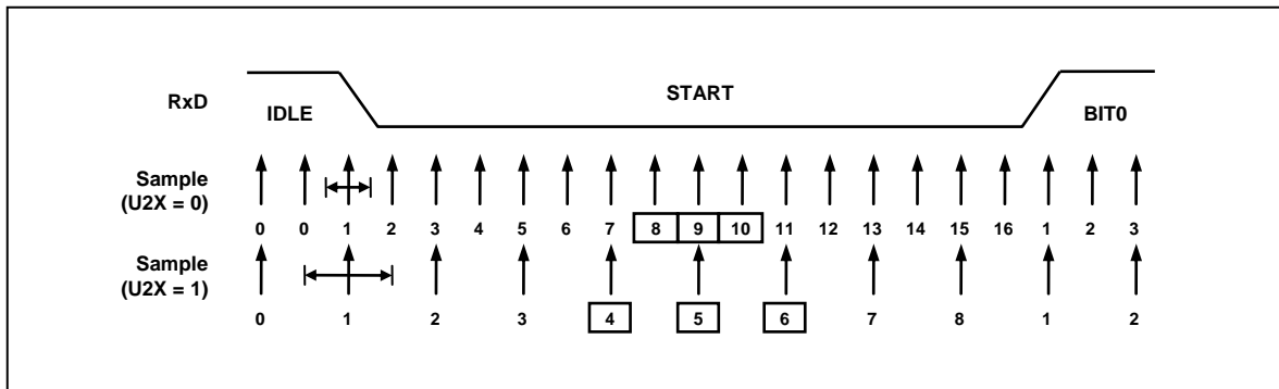
Figure 11-27 Start Bit Sampling
