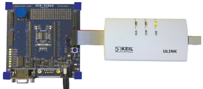
The Keil ULINK USB-JTAG Adapter connects to a wide range of evaluation boards. For more information refer to www.keil.com/ulink .
