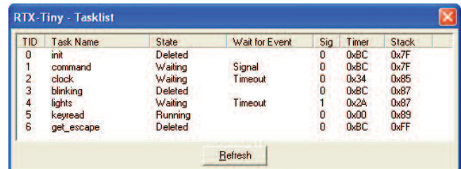
The µVision Debugger includes a kernel-aware dialog for RTX51 Tiny2 that displays complete information about all the tasks in your program.
