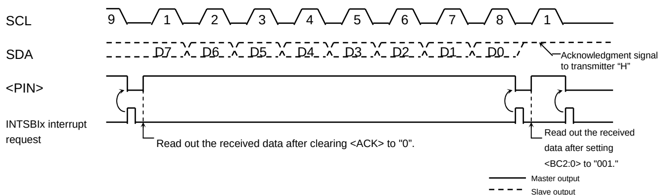
Fig. 10-17 Terminating Data Transmission in the Master Receiver Mode
