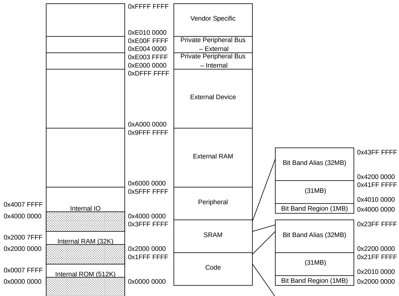
Fig 4.1 Memory map (TMPM330FDFG)
