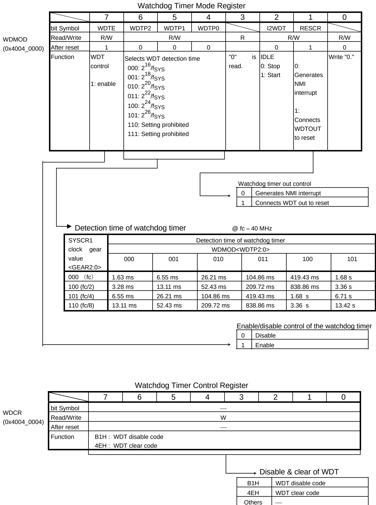
Fig. 14-4 Watchdog Timer Registers
