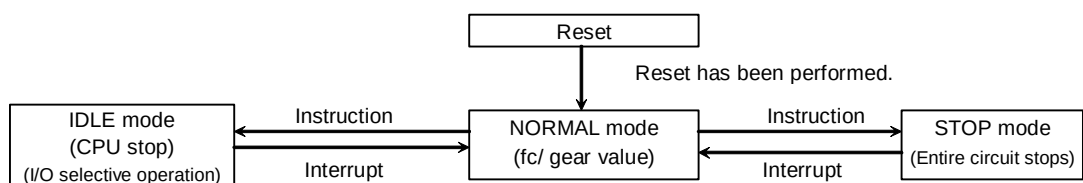
(a) Mode Transition Diagram of Single Clock Mode
