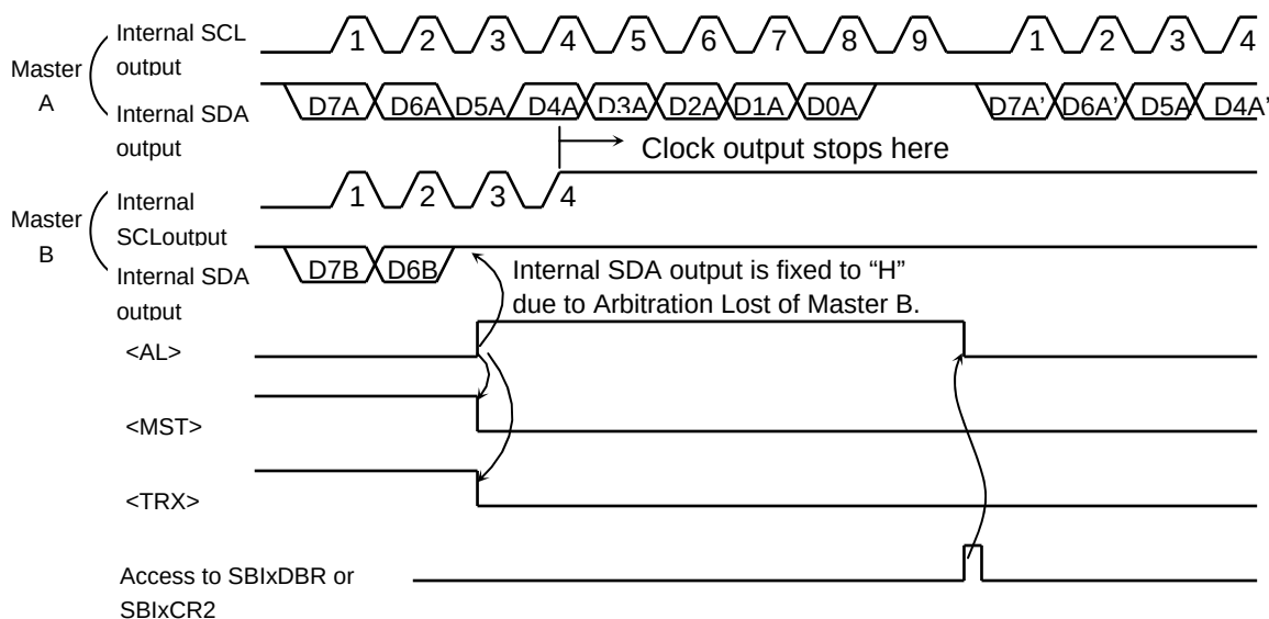
Fig. 10-13 Example of Master B Lost Arbitration ( \text{D7A} = \text{D7B} , \text{D6A} = \text{D6B} )
