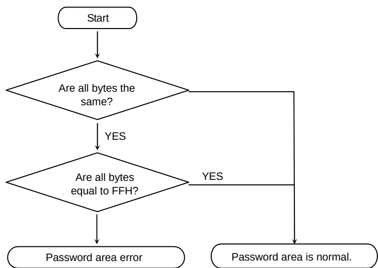
Fig. 16-7 Password Area Verification Flow
