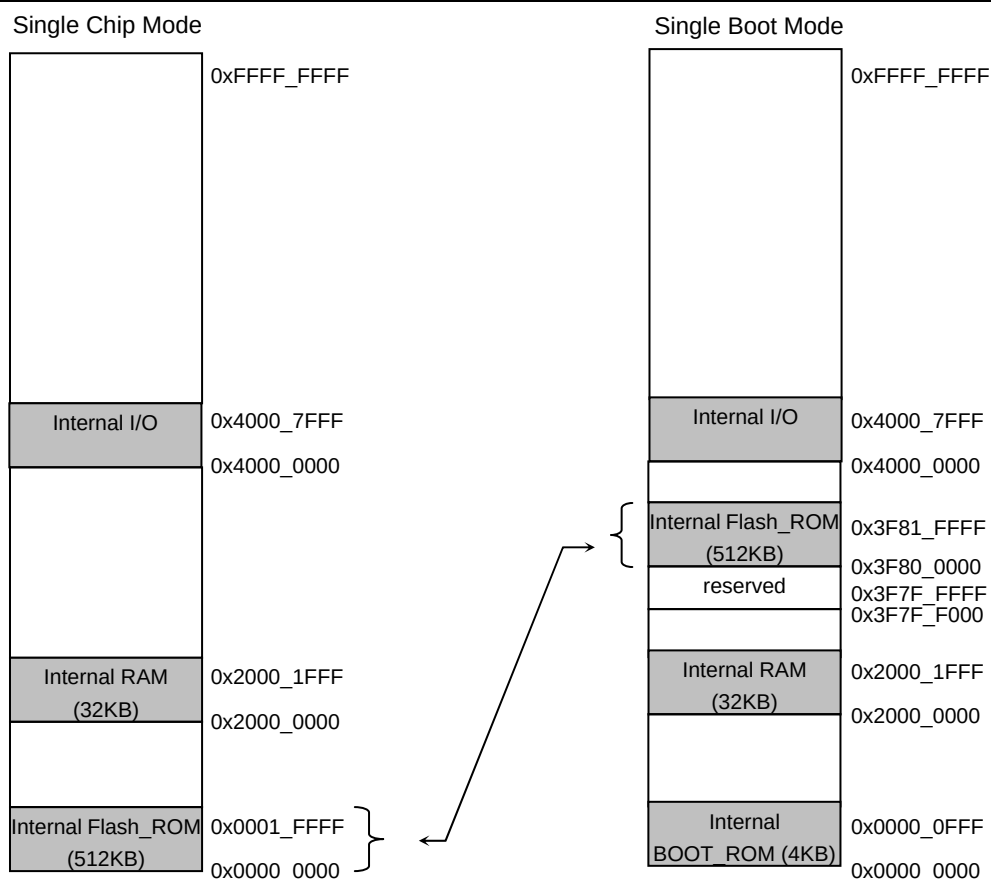
Fig. 16-3 Memory Maps for TPM332FWUG
