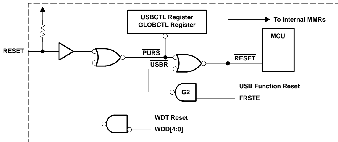
Figure 5–1. Reset Diagram
