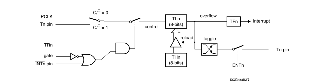
Fig 17. Timer/counter 0 or 1 in Mode 2 (8-bit auto-reload).
