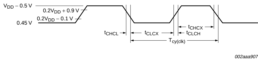
Fig 17. External clock timing
