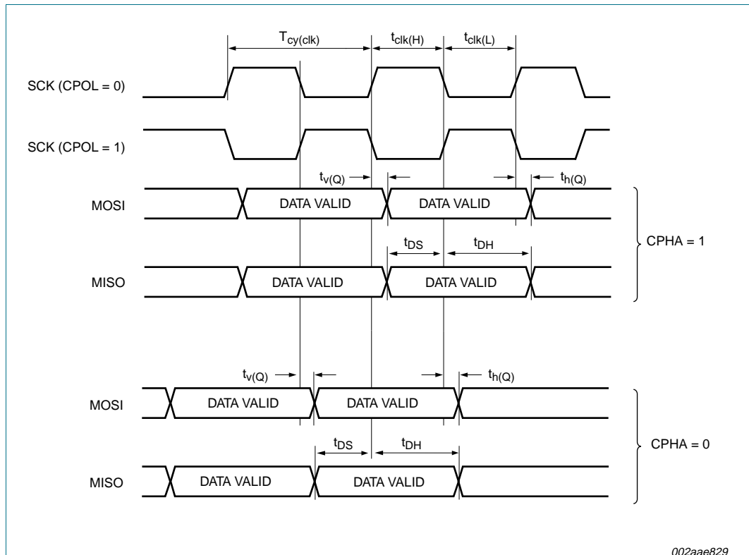
Fig 21. SSP master timing in SPI mode
