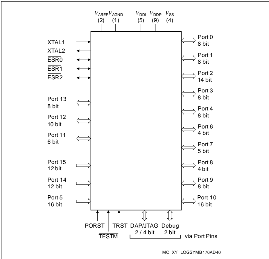
Figure 1 XC2297H Logic Symbol
