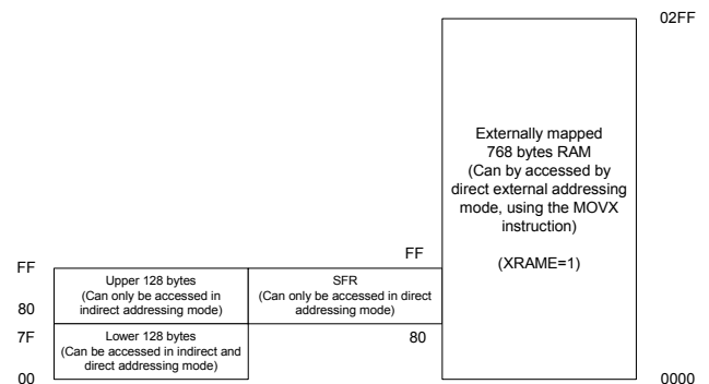
FIGURE 4: VRS570 /VRS580 RAM MEMORY
