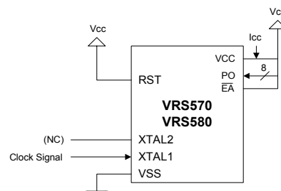
FIGURE 24: ICC ACTIVE MODE TEST CIRCUIT
