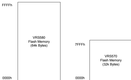
FIGURE 3: VRS580 / VRS570 INTERNAL PROGRAM MEMORY
