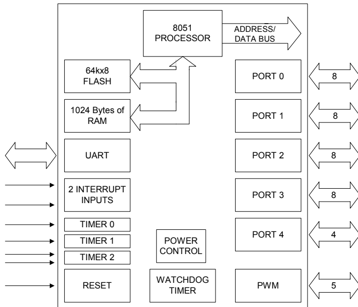
FIGURE 1: VRS570 / VRS580 FUNCTIONAL DIAGRAM
