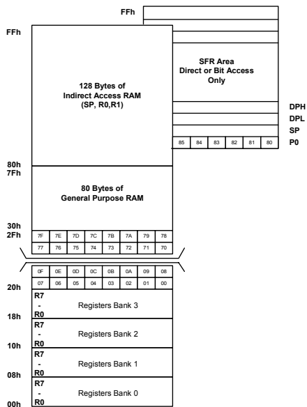
FIGURE 5: VRS570 / VRS580 INTERNAL LOWER 256 B RAM STRUCTURE
