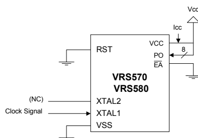
FIGURE 23: ICC IDLE MODE TEST CIRCUIT
