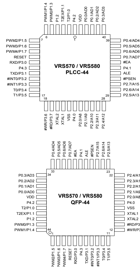
FIGURE 2: VRS570 / VRS580 PLCC AND QFP PINOUT DIAGRAMS
