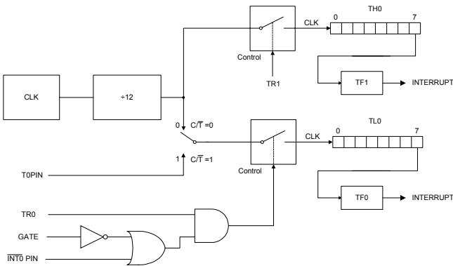
FIGURE 13: TIMER/COUNTER 0 MODE 3
