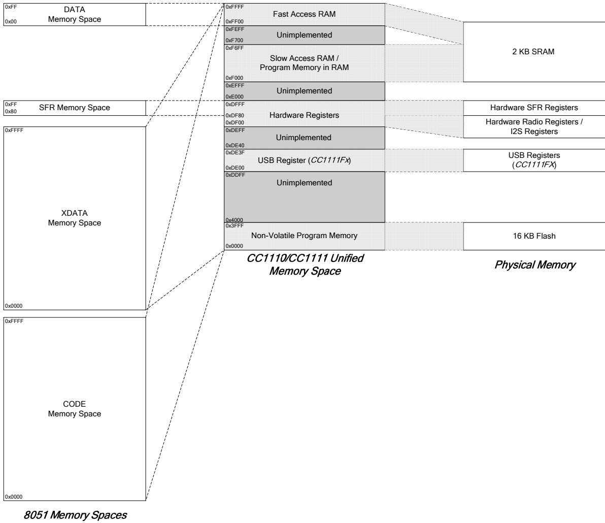
Figure 15: CC110F16 CC111F16 Memory Mapping
