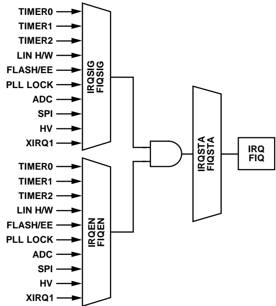
Figure 22. Interrupt Structure
