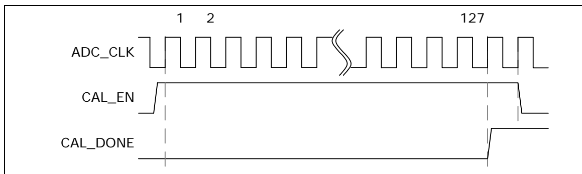
Figure 5-87 ADC Converter Self-Calibration Timing Diagram
