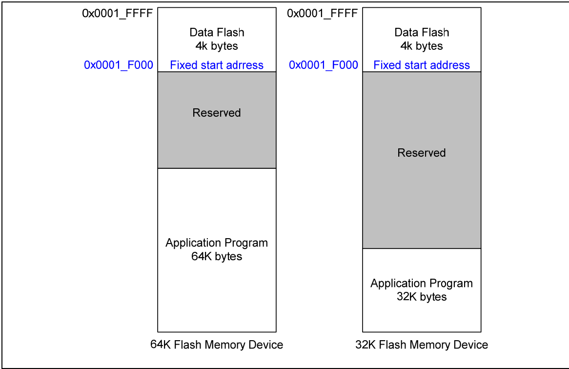
Figure 6-6 NuMicro™ NUC100/NUC120 Low Density Flash Memory Structure
