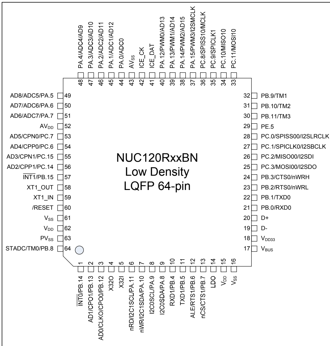
Figure 3-10 NuMicro™ NUC120 Low Density LQFP 64-pin Pin Diagram
