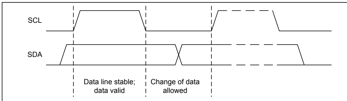
Figure 5-23 Bit Transfer on the I 2 C bus
