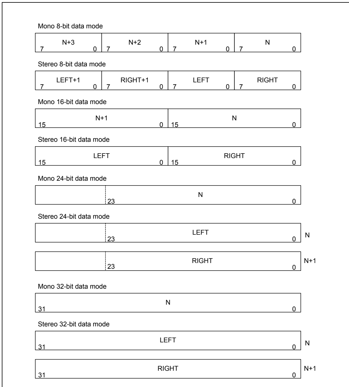
Figure 5-85 FIFO contents for various I 2 S modes
