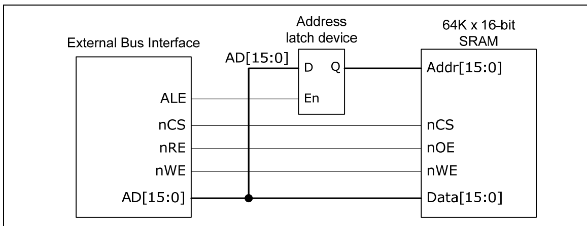
Figure 5-101 Connection of 16-bit EBI Data Width with 16-bit Device
