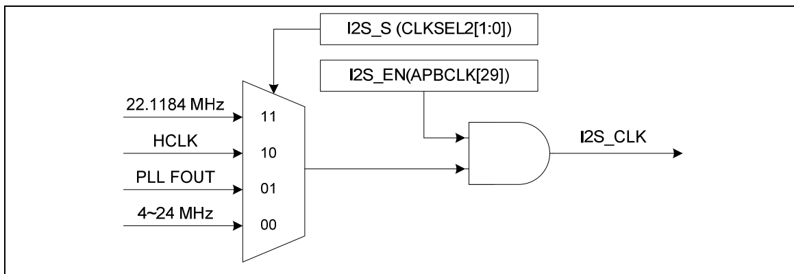
Figure 5-81 I²S Clock Control Diagram
