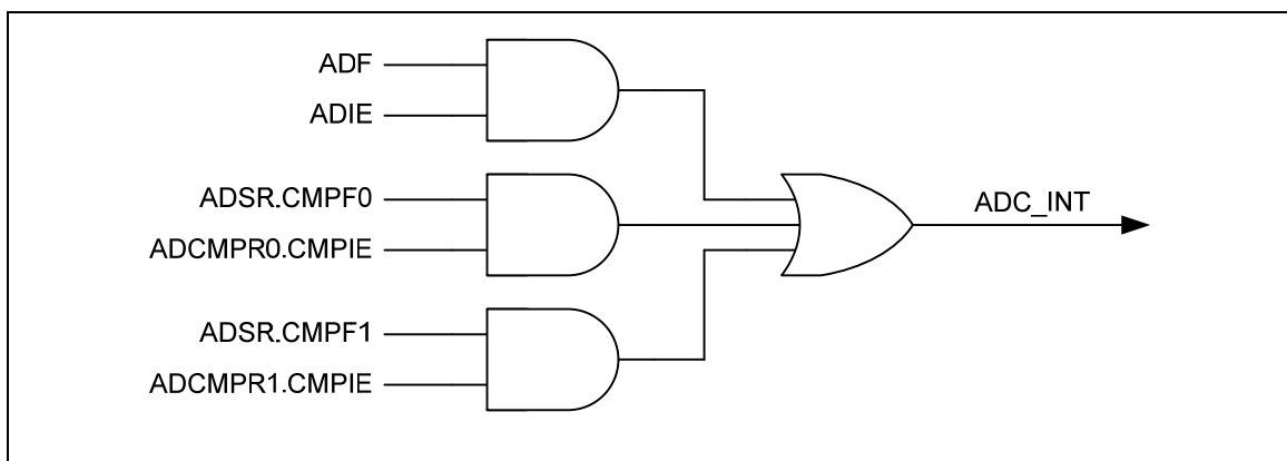
Figure 5-93 A/D Controller Interrupt
