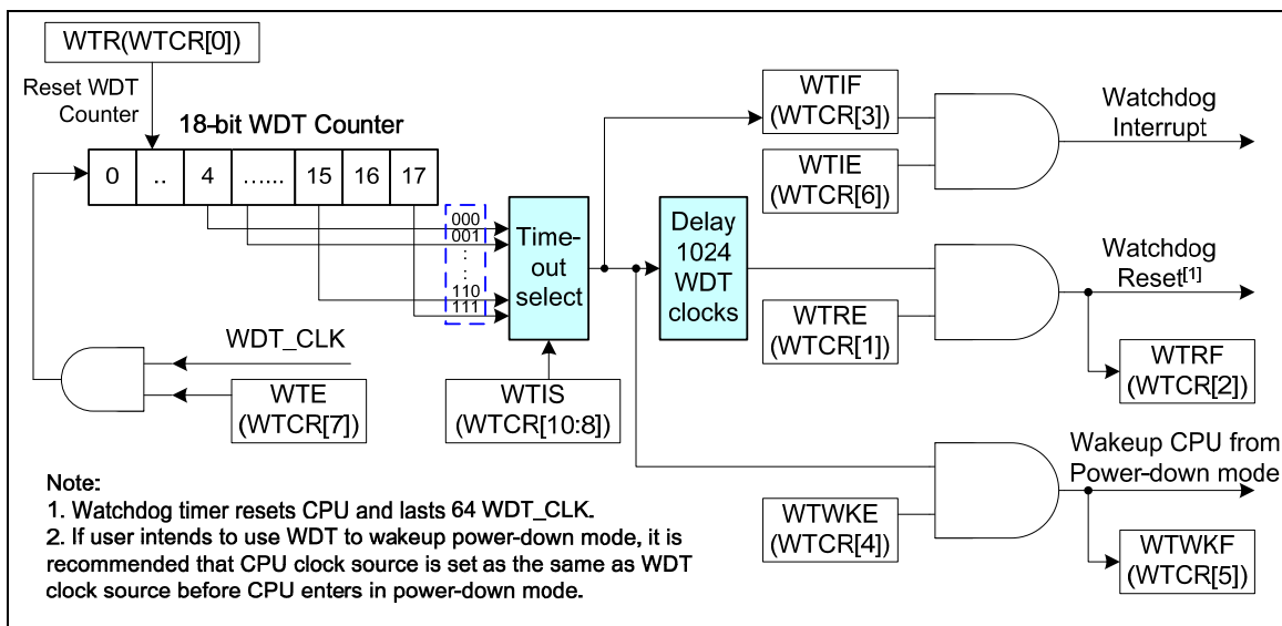
Figure 5-68 Watchdog Timer Block Diagram
