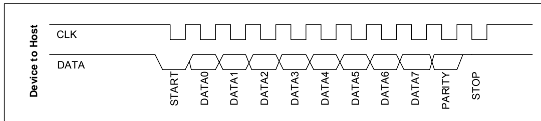
Figure 5-76 Data Format of Device-to-Host
