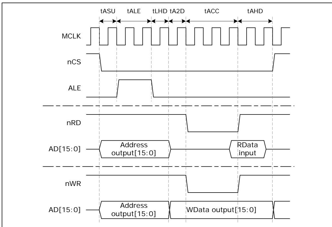
Figure 5-103 Timing Control Waveform for 16-bit Data Width
