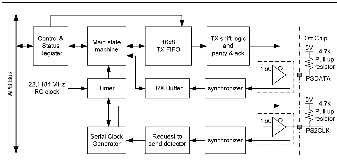
Figure 5-75 PS/2 Device Block Diagram
