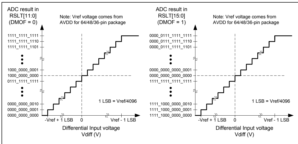
Figure 5-95 ADC differential input conversion voltage and conversion result mapping diagram
