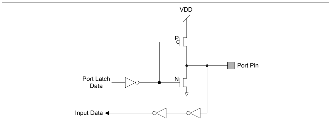
Figure 5-15 Push-Pull Output
