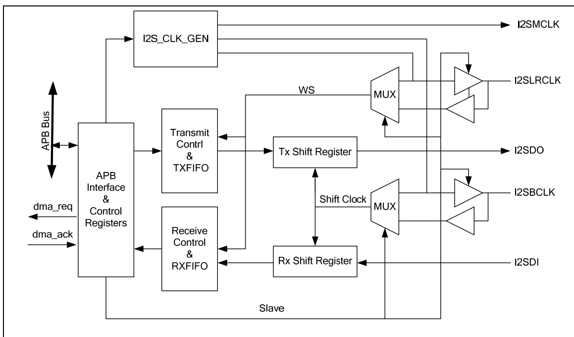
Figure 5-82 I²S Controller Block Diagram
