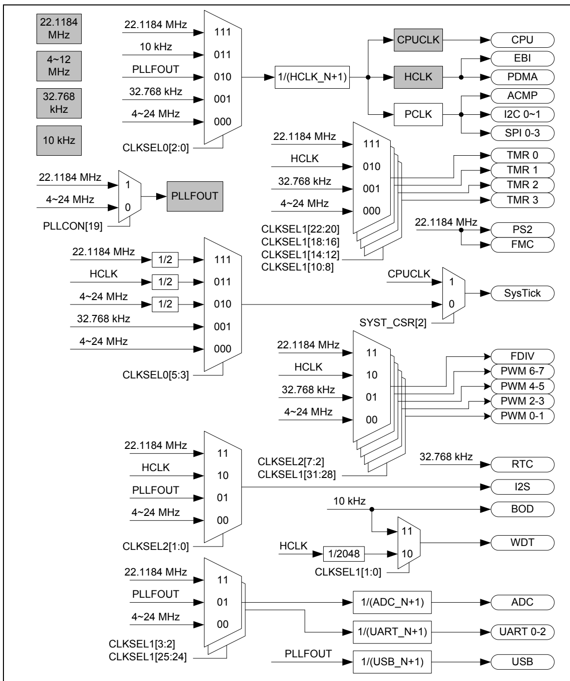
Figure 5-4 Clock generator global view diagram
