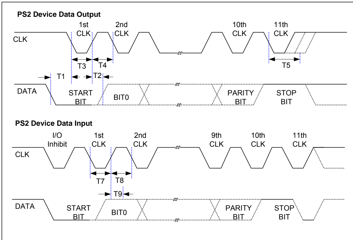
Figure 5-79 PS/2 Bus Timing
