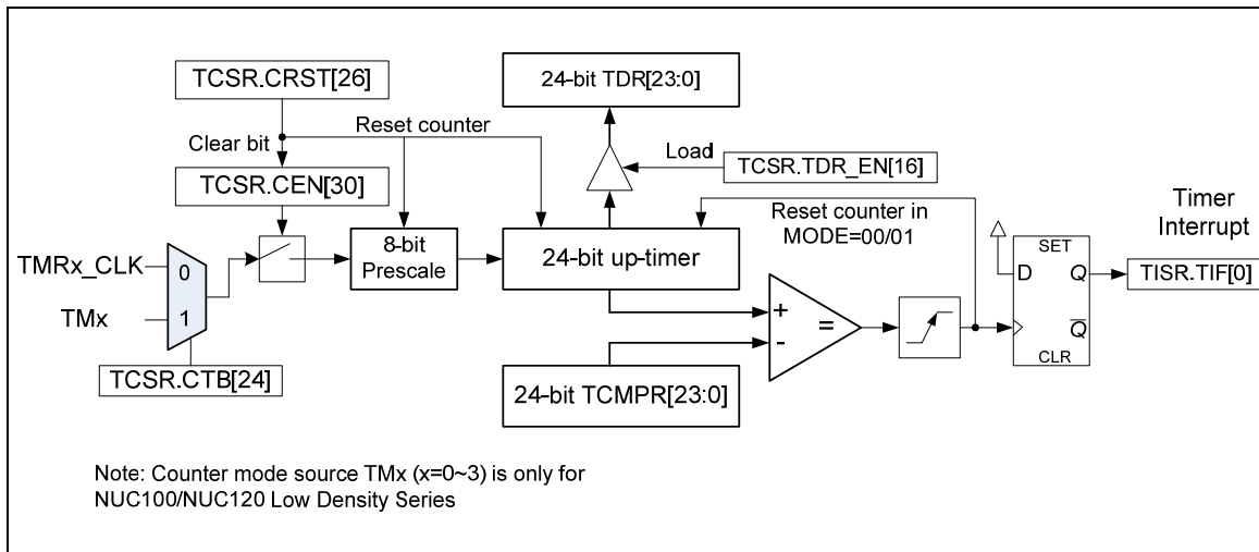
Figure 5-63 Timer Controller Block Diagram
