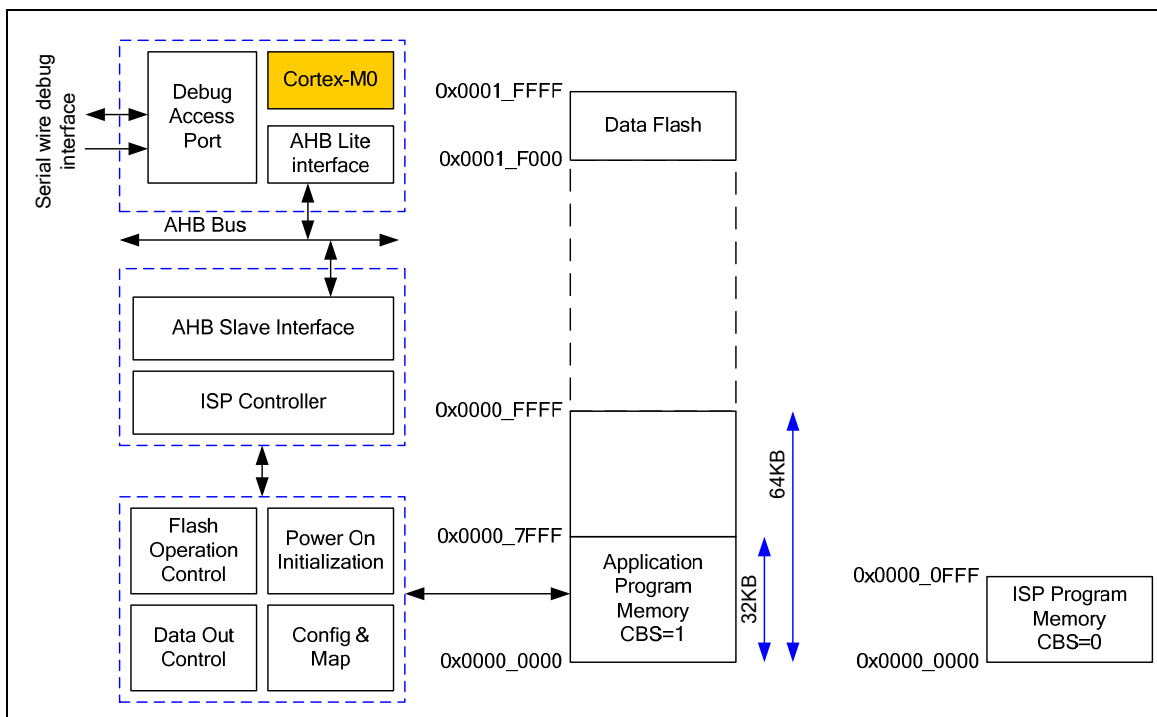
Figure 6-2 NuMicro™ NUC100/NUC120 Low Density Flash Memory Control Block Diagram
