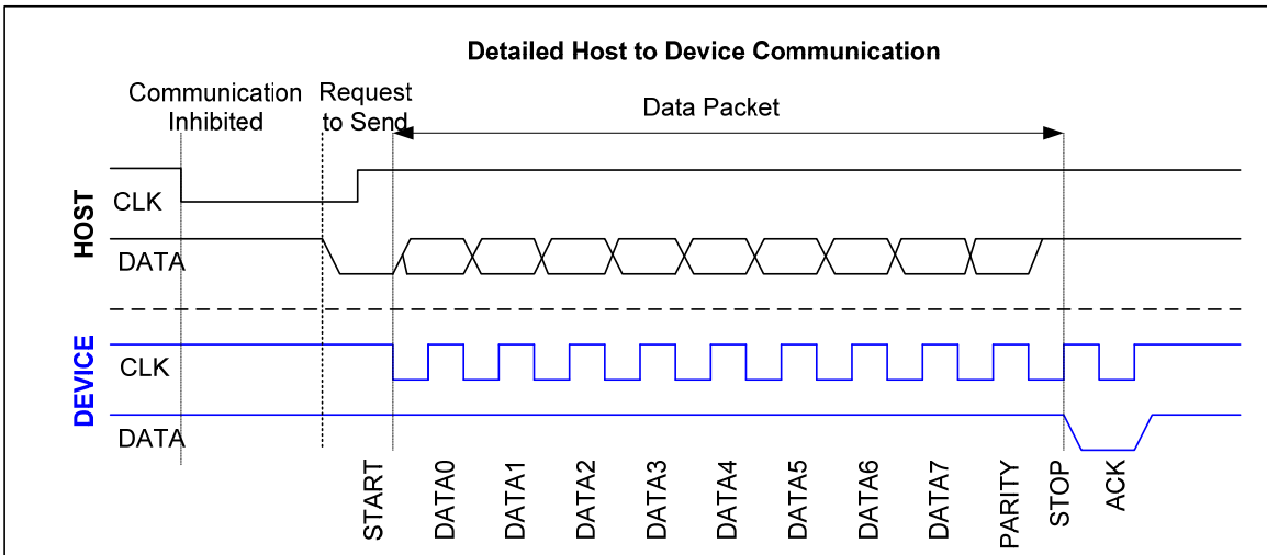
Figure 5-78 PS/2 Bit Data Format
