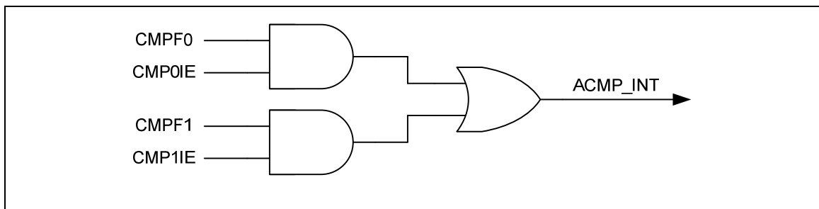
Figure 5-97 Comparator Controller Interrupt Sources
