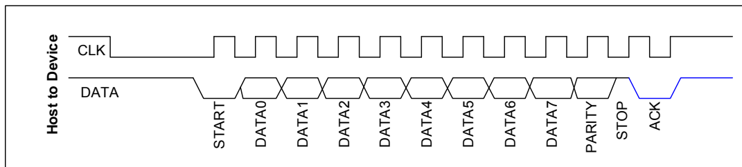
Figure 5-77 Data Format of Host-to-Device
