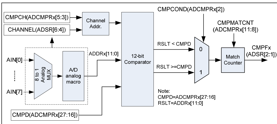
Figure 5-92 A/D Conversion Result Monitor Logics Diagram
