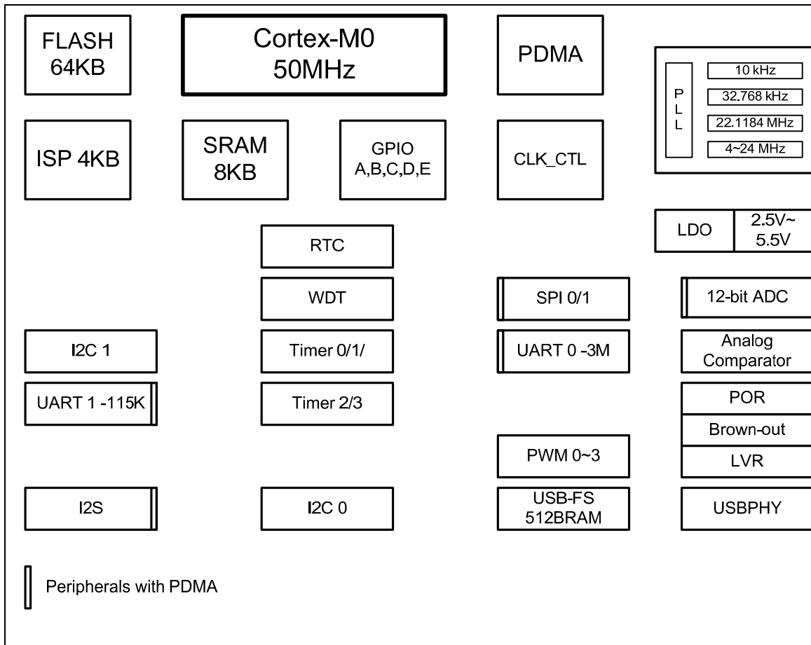
Figure 4-4 NuMicro™ NUC120 Low Density Block Diagram
