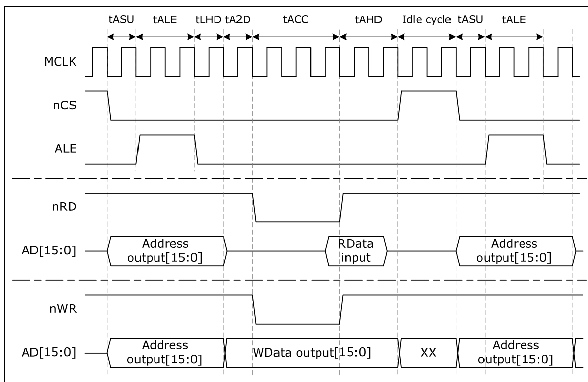
Figure 5-105 Timing Control Waveform for Insert Idle Cycle
