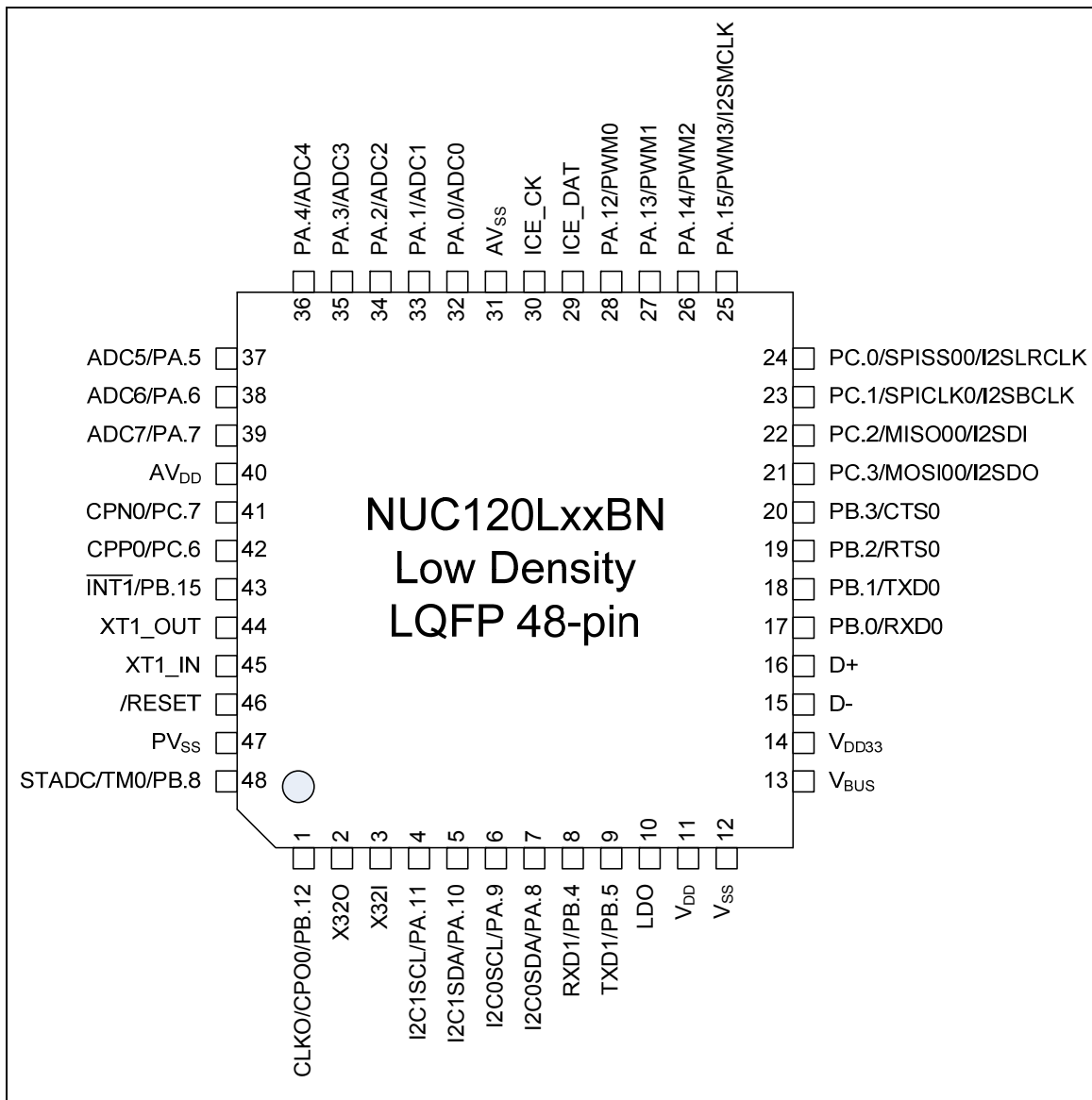
Figure 3-11 NuMicro™ NUC120 Low Density LQFP 48-pin Pin Diagram
