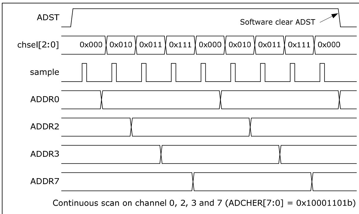
Figure 5-91 Continuous Scan on Enabled Channels Timing Diagram
