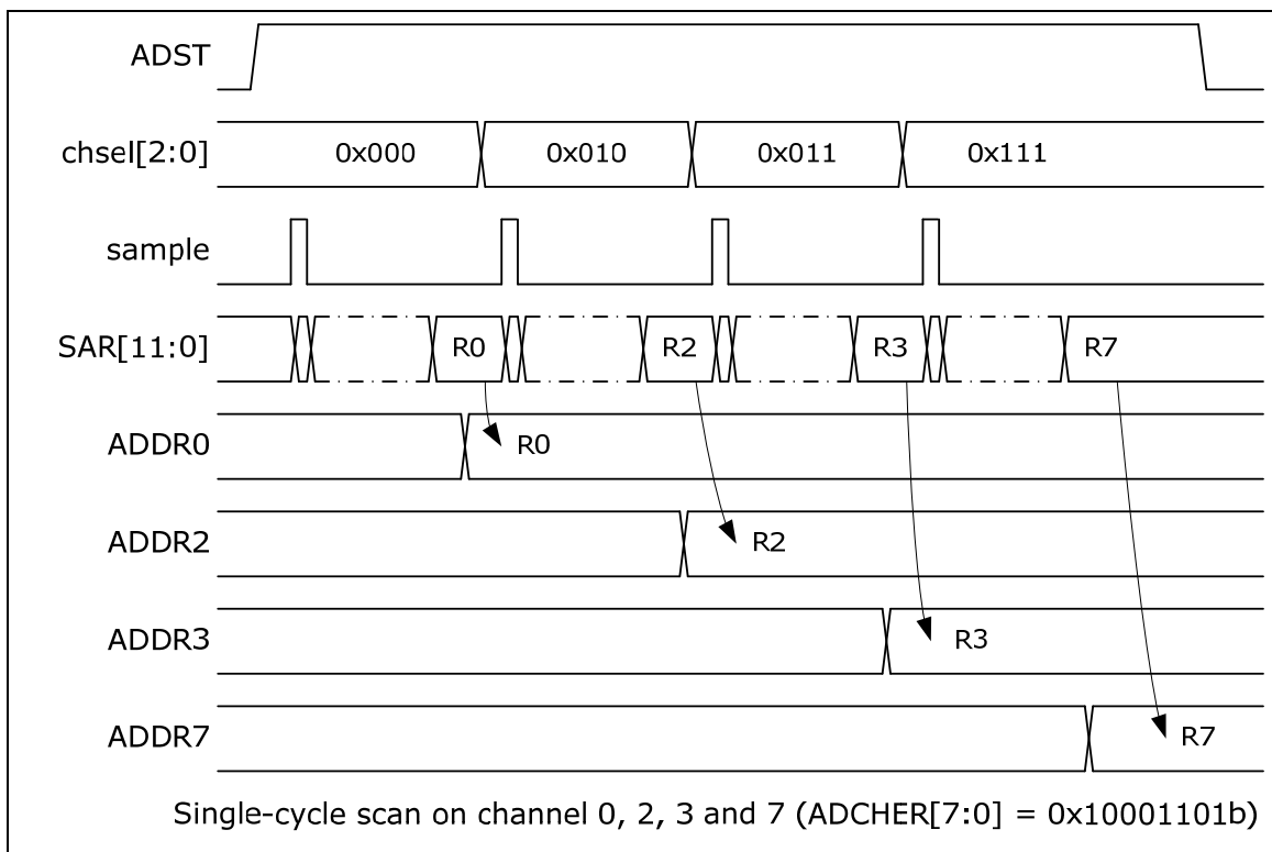
Figure 5-90 Single-Cycle Scan on Enabled Channels Timing Diagram
