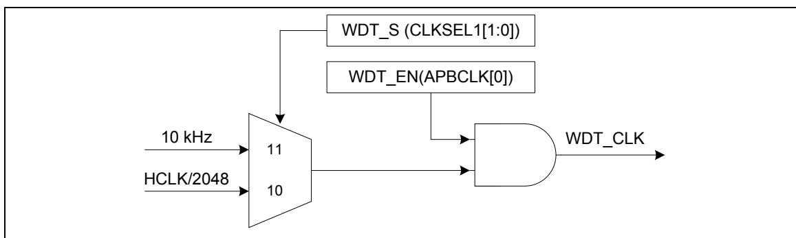
Figure 5-67 Watchdog Timer Clock Control
