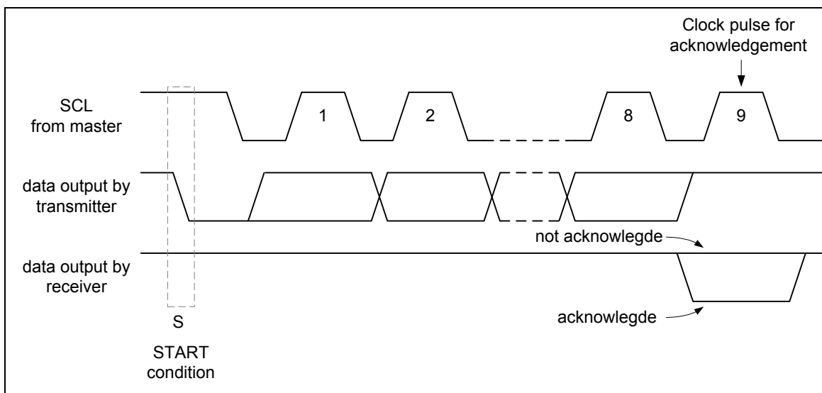
Figure 5-24 Acknowledge on the I 2 C bus
