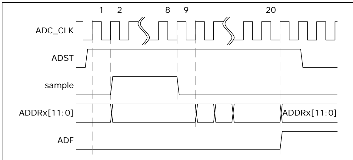
Figure 5-89 Single Mode Conversion Timing Diagram
