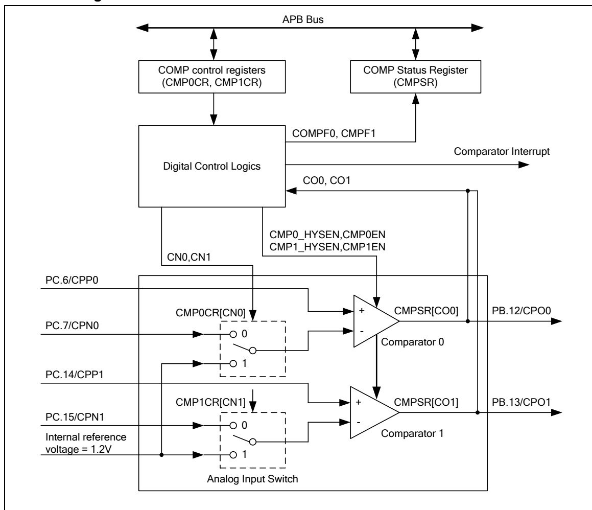
Figure 5-96 Analog Comparator Block Diagram
