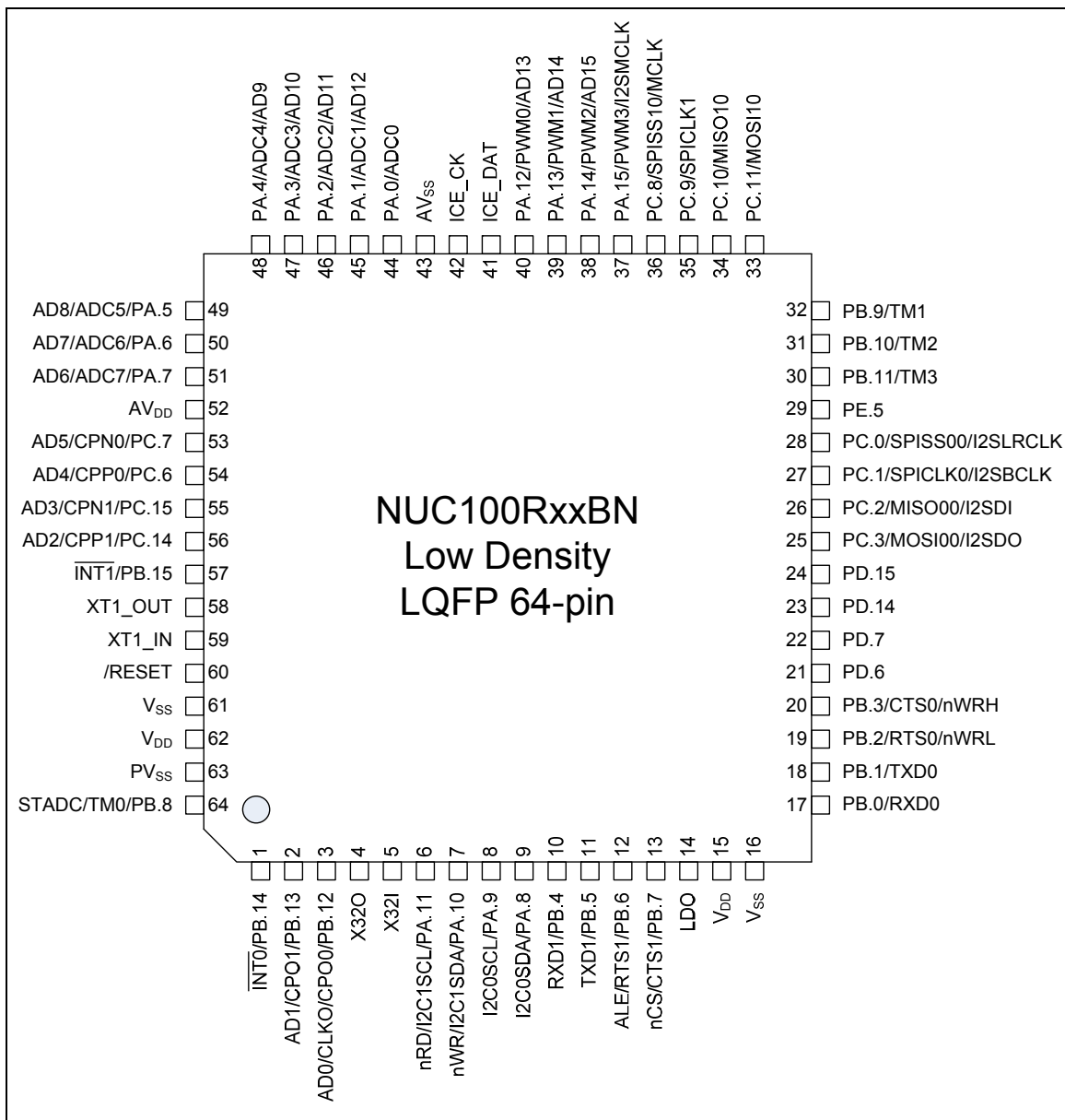
Figure 3-8 NuMicro™ NUC100 Low Density LQFP 64-pin Pin Diagram
