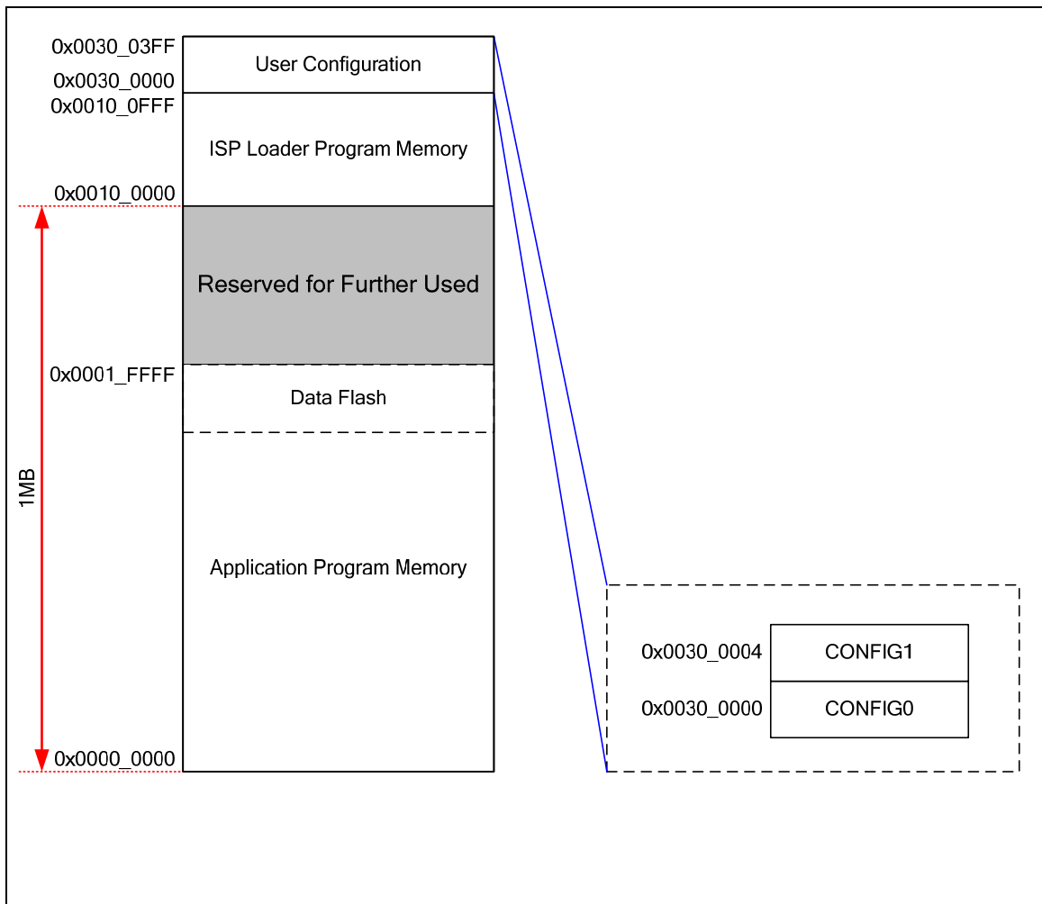
Figure 6-3 NuMicro™ NUC100/NUC120 Medium Density Flash Memory Organization
