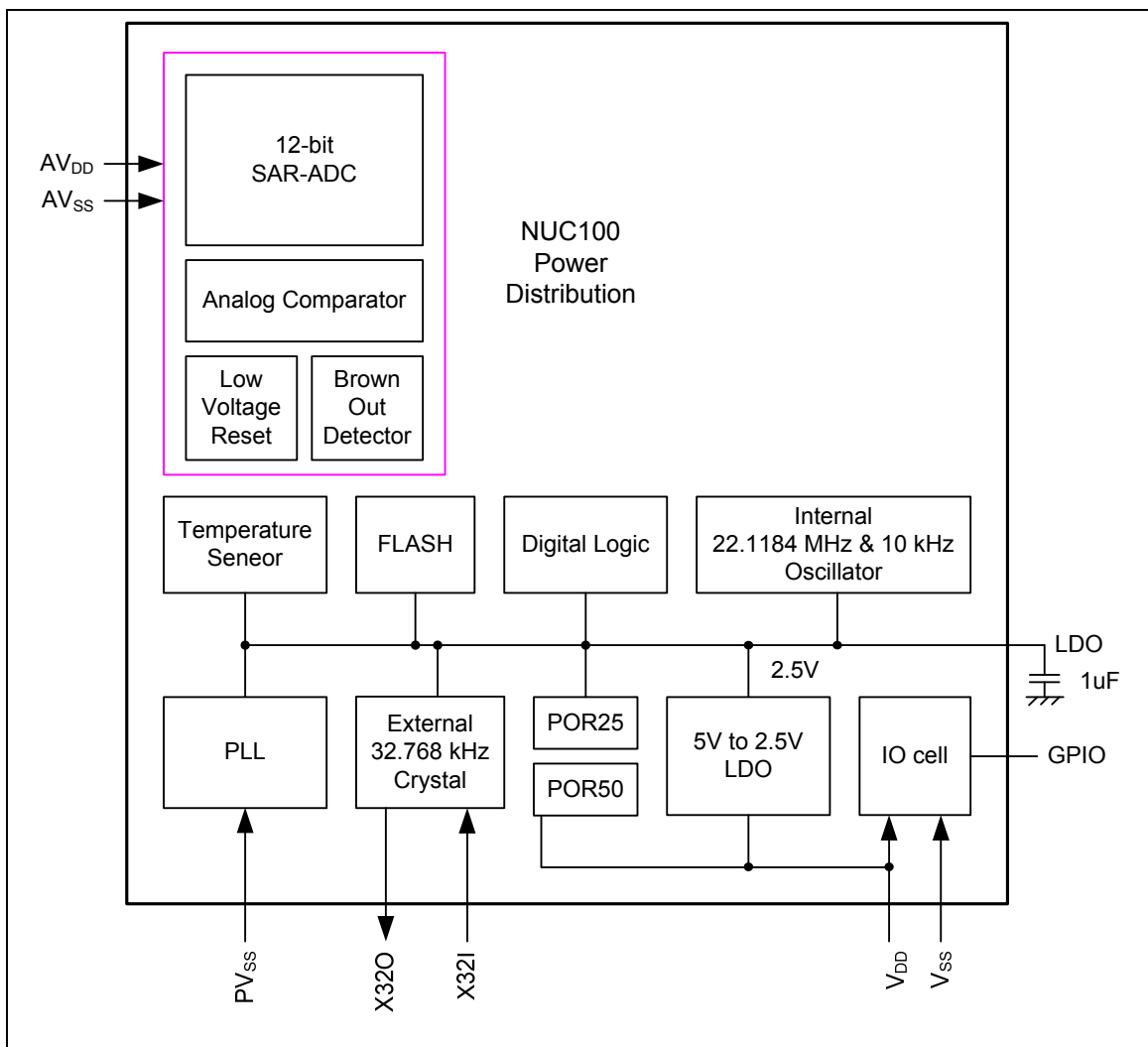
Figure 5-3 NuMicro™ NUC100 Power Distribution Diagram
