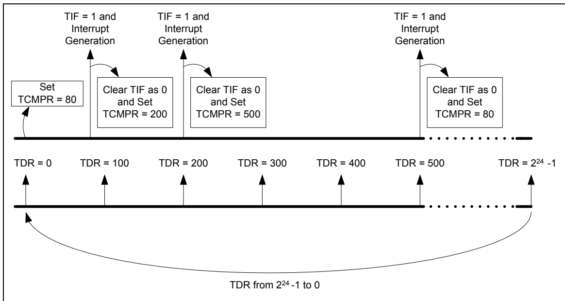
Figure 5-65 Continuous Counting Mode
