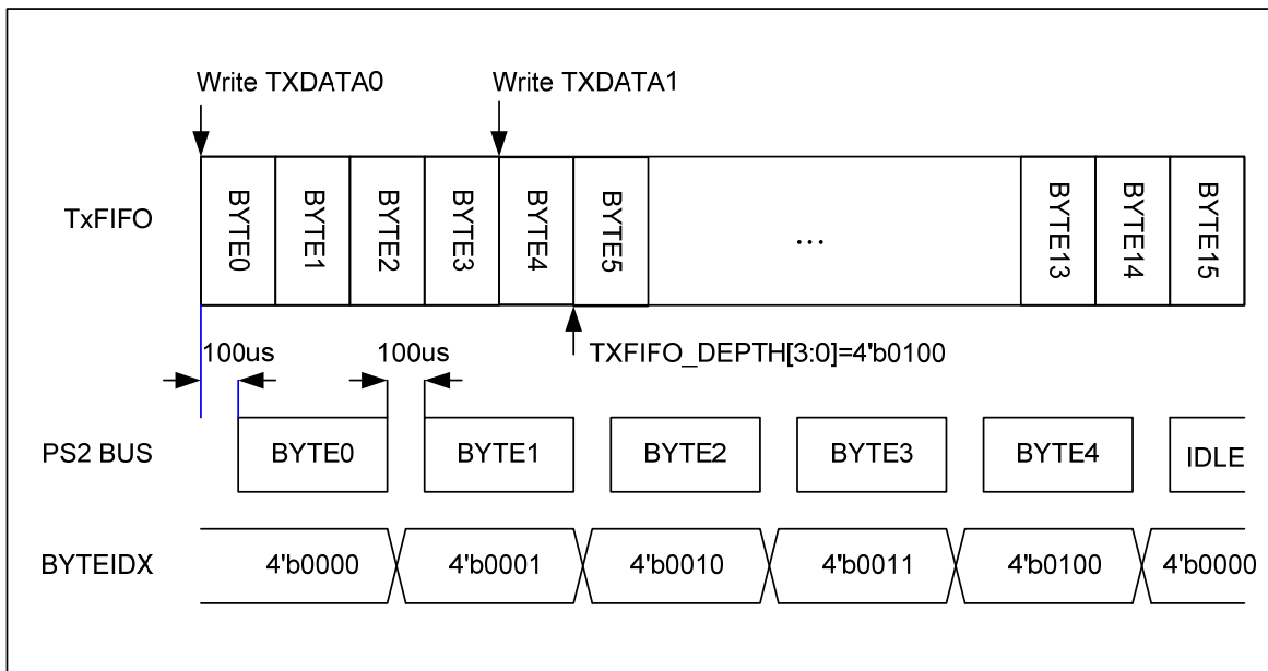
Figure 5-80 PS/2 Data Format
