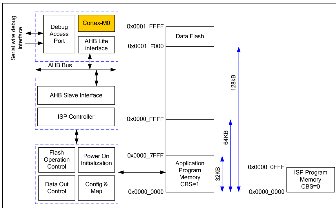
Figure 6-1 NuMicro™ NUC100/NUC120 Medium Density Flash Memory Control Block Diagram
