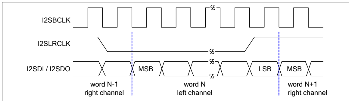
Figure 5-83 I 2 S Bus Timing Diagram (Format=0)
