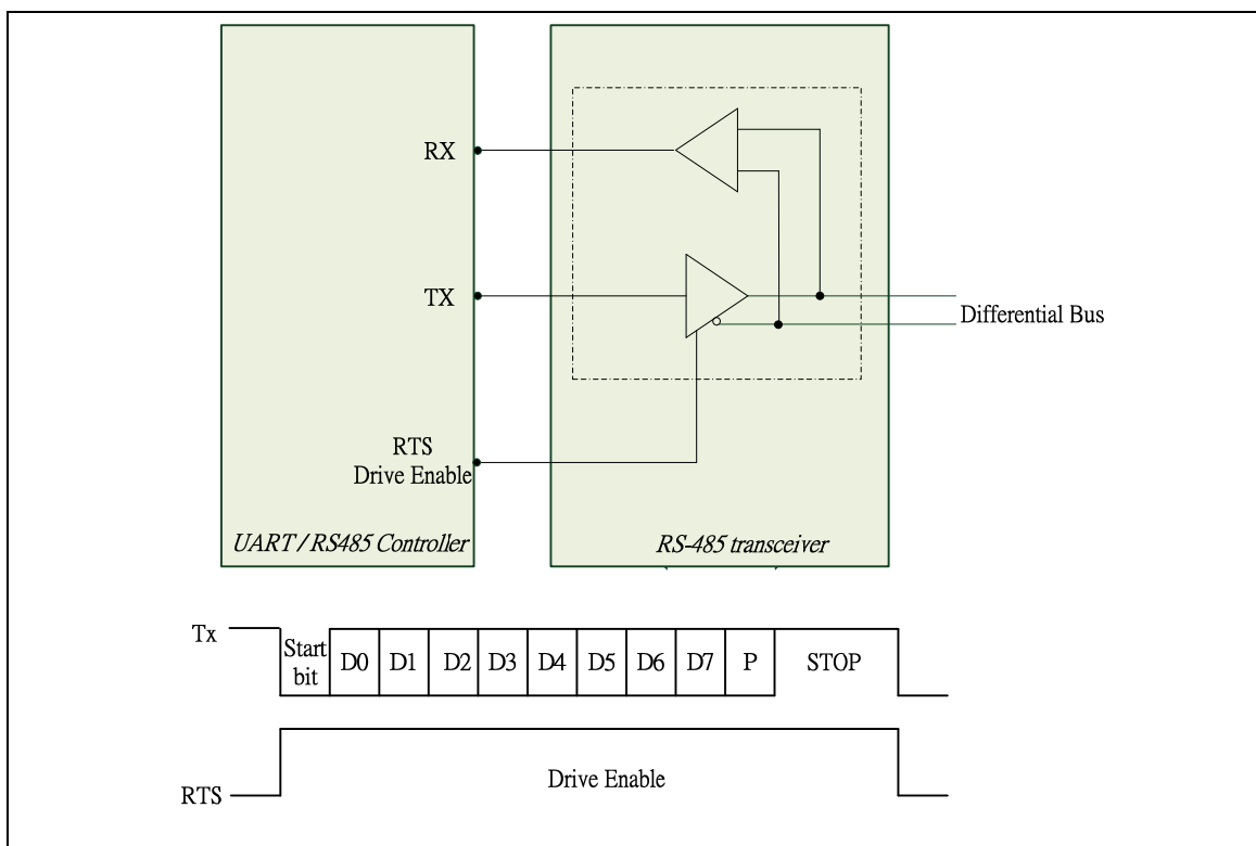
Figure 5-74 Structure of RS-485 Frame
