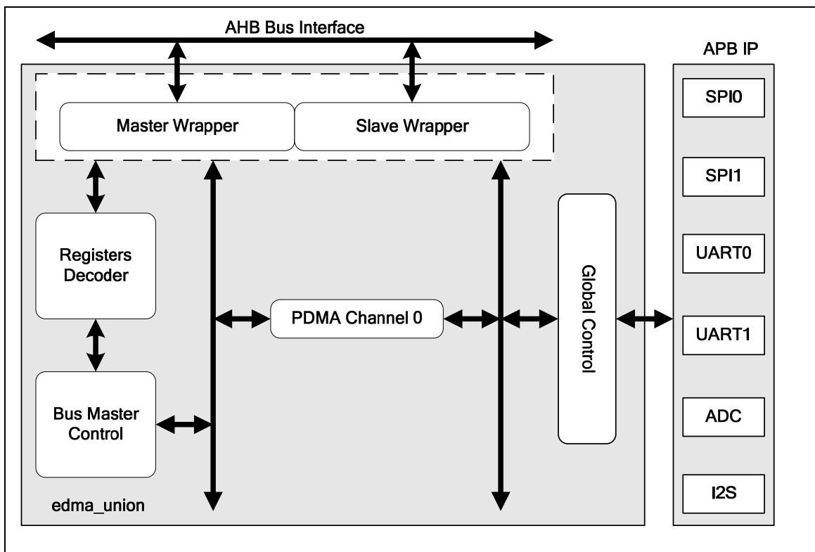
Figure 5-99 NuMicro™ NUC100/NUC120 Low Density PDMA Controller Block Diagram
