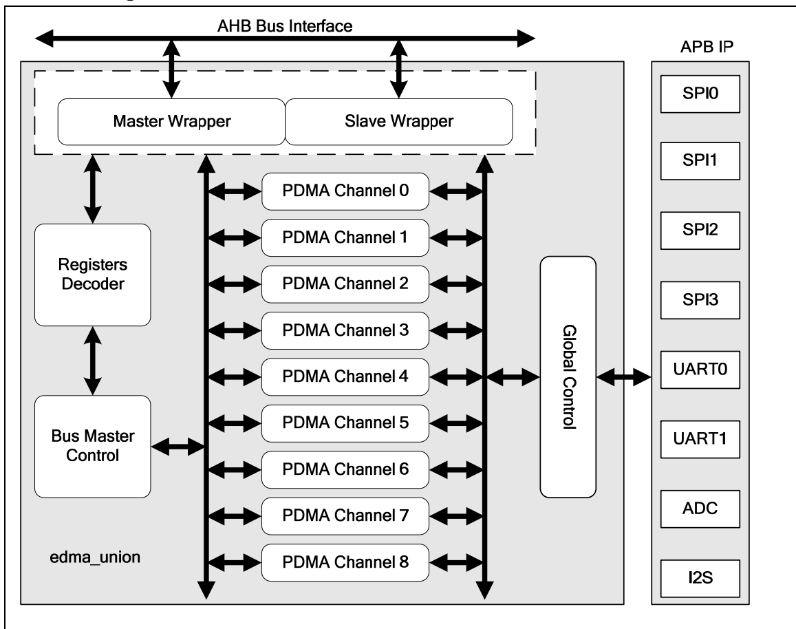
Figure 5-98 NuMicro™ NUC100/NUC120 Medium Density PDMA Controller Block Diagram
