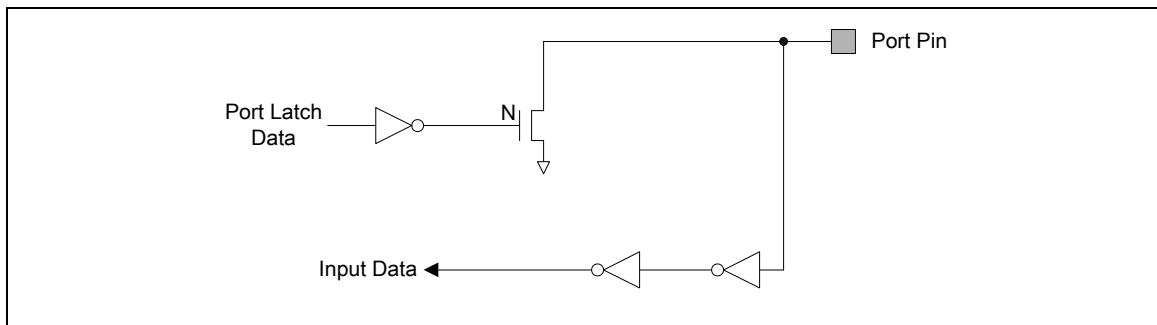
Figure 5-16 Open-Drain Output
