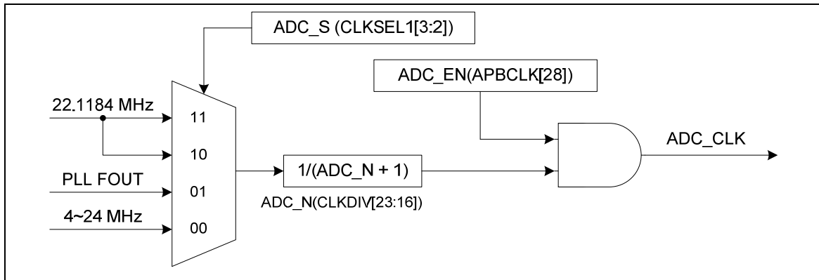
Figure 5-88 ADC Clock Control
