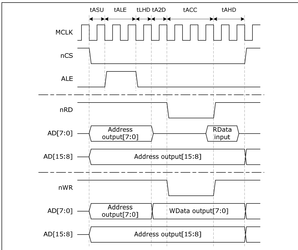
Figure 5-104 Timing Control Waveform for 8-bit Data Width
