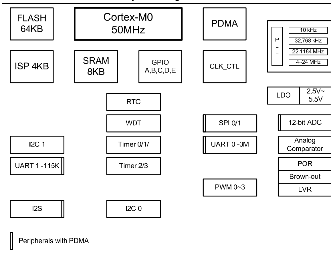
Figure 4-3 NuMicro™ NUC100 Low Density Block Diagram
