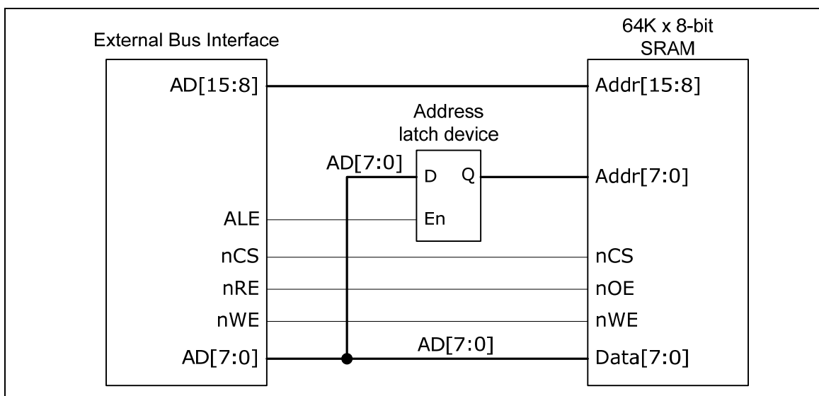
Figure 5-102 Connection of 8-bit EBI Data Width with 8-bit Device
