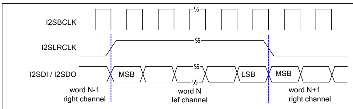
Figure 5-84 MSB Justified Timing Diagram (Format=1)
