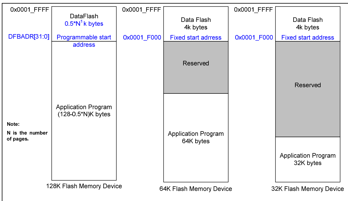
Figure 6-5 NuMicro™ NUC100/NUC120 Medium Density Flash Memory Structure
