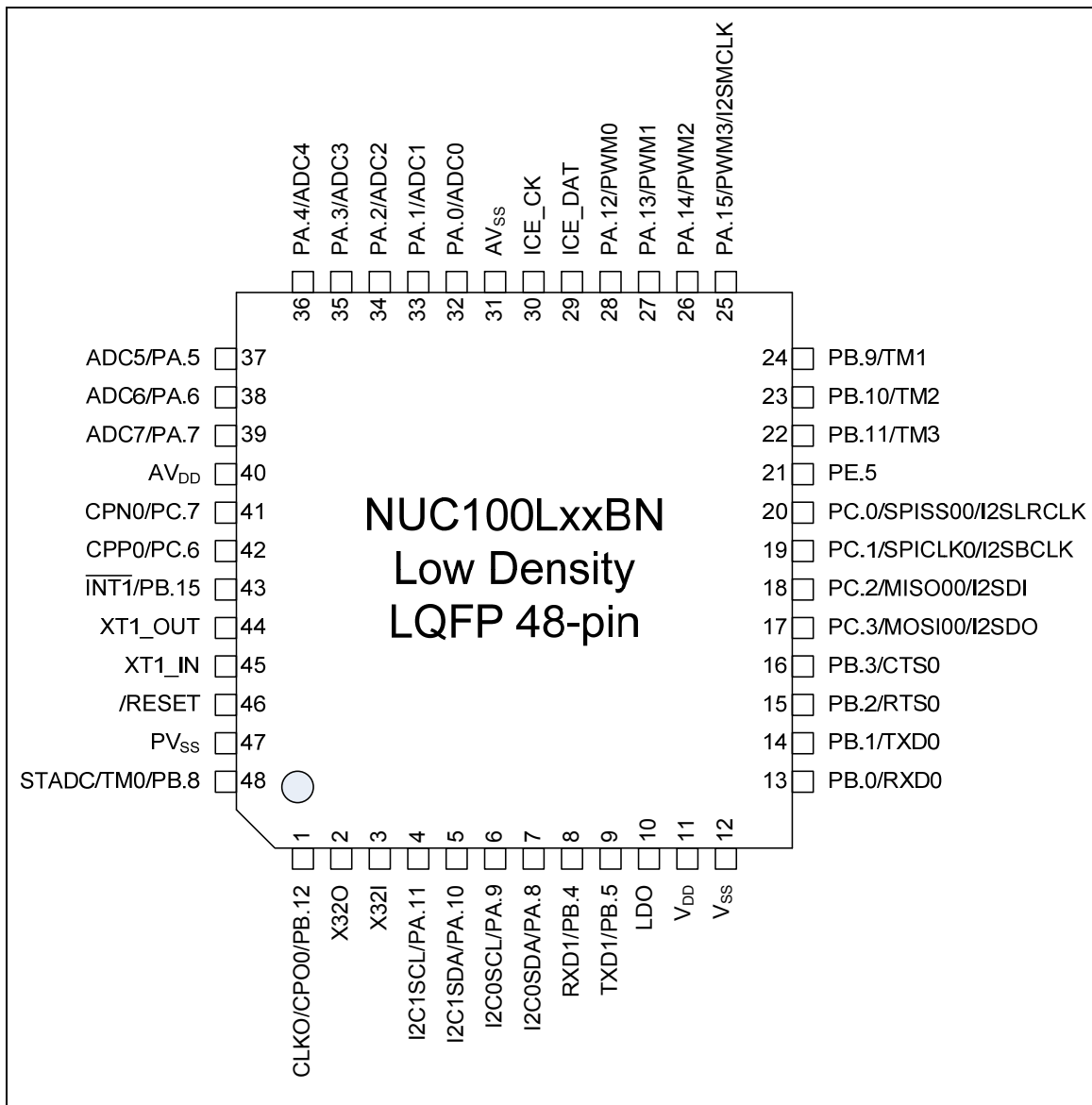
Figure 3-9 NuMicro™ NUC100 Low Density LQFP 48-pin Pin Diagram
