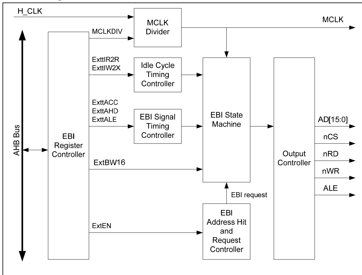
Figure 5-100 EBI Block Diagram
