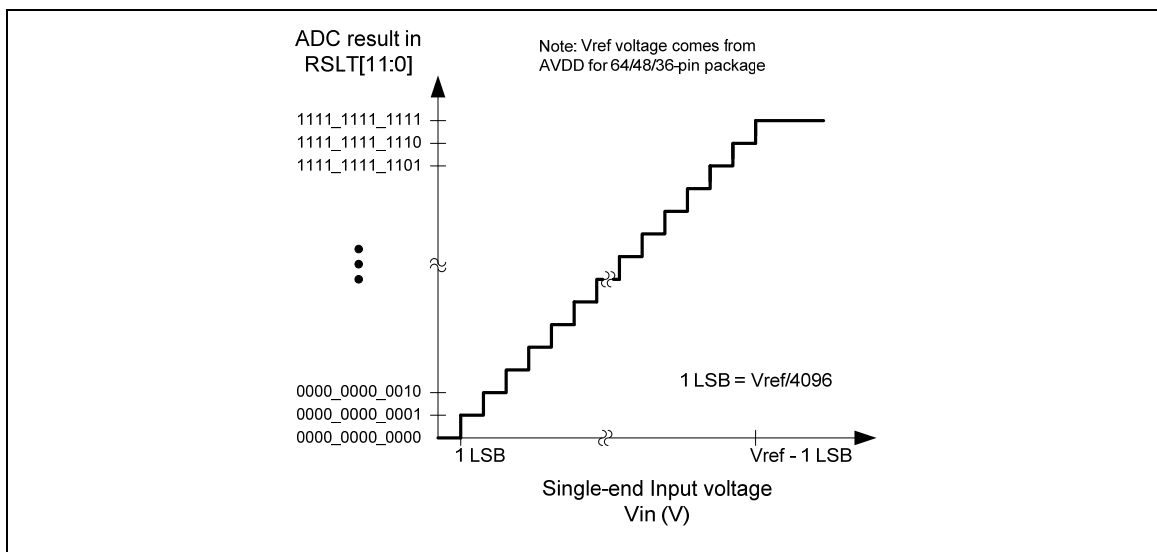
Figure 5-94 ADC single-end input conversion voltage and conversion result mapping diagram
