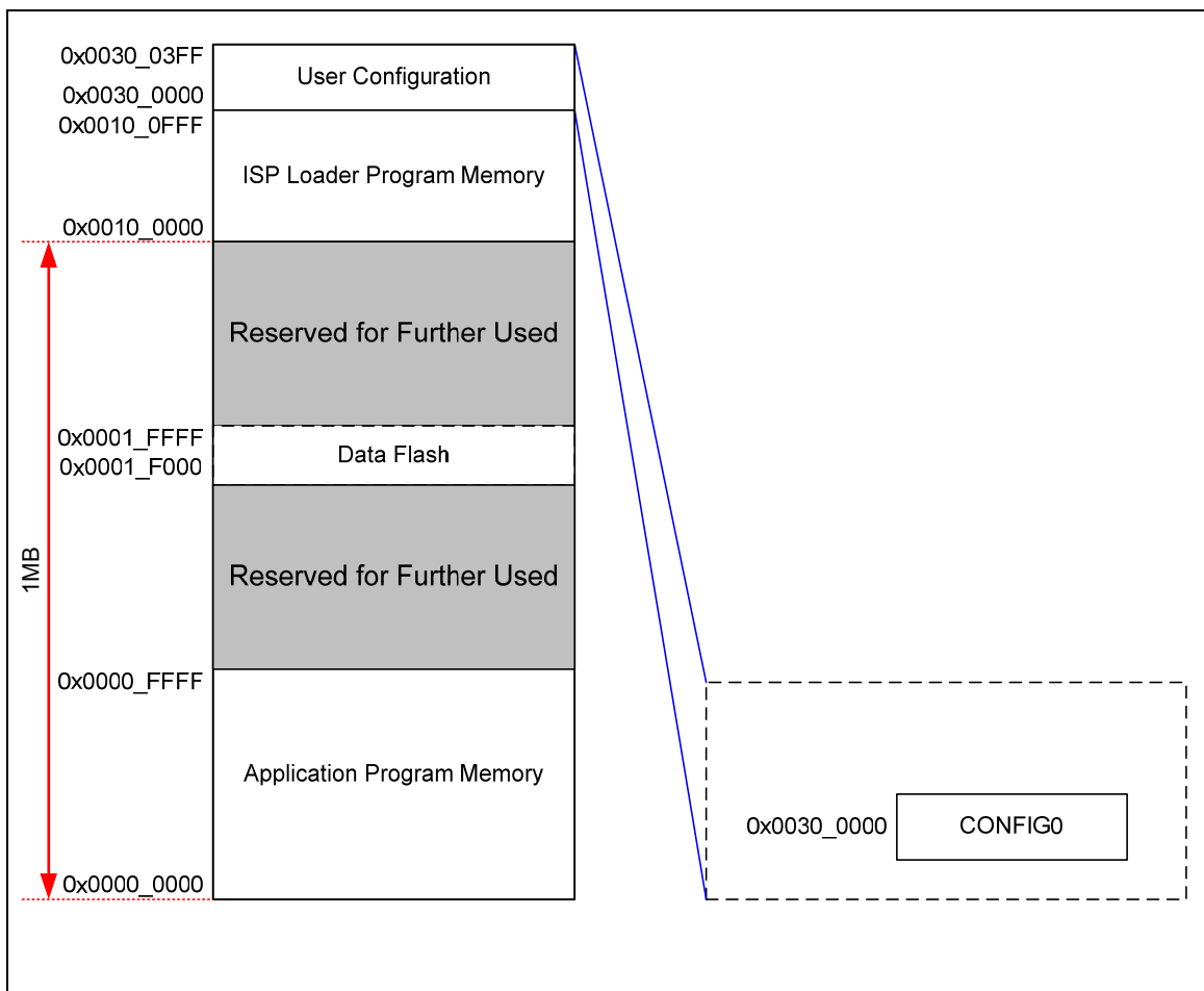
Figure 6-4 NuMicro™ NUC100/NUC120 Low Density Flash Memory Organization
