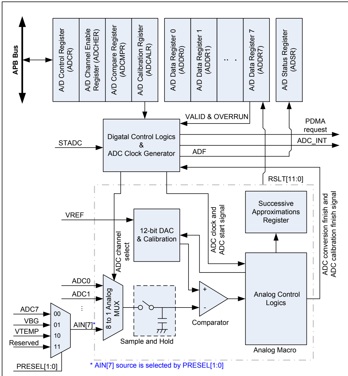
Figure 5-86 ADC Controller Block Diagram
