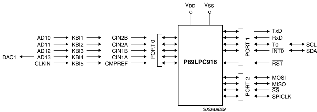
Fig 2. P89LPC916 logic symbol.
