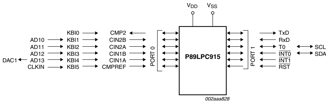
Fig 1. P89LPC915 logic symbol.
