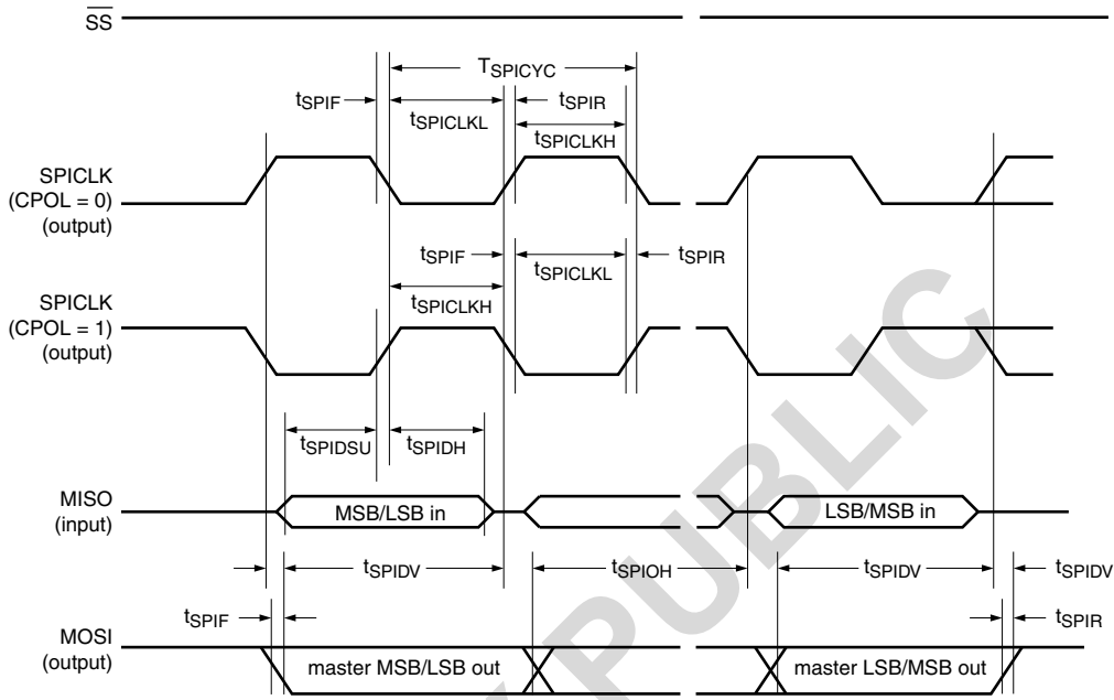
Fig 44. SPI master timing (CPHA = 1)
