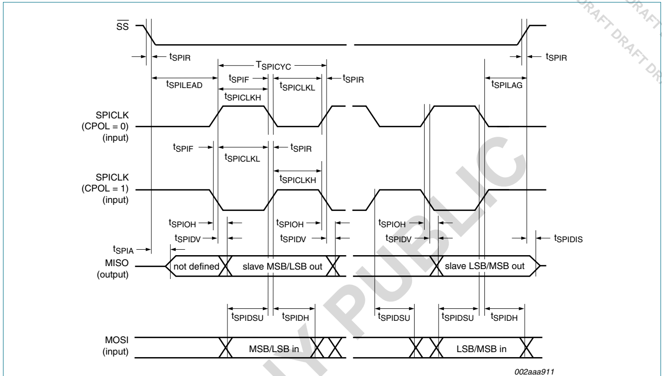
Fig 46. SPI slave timing (CPHA = 1)
