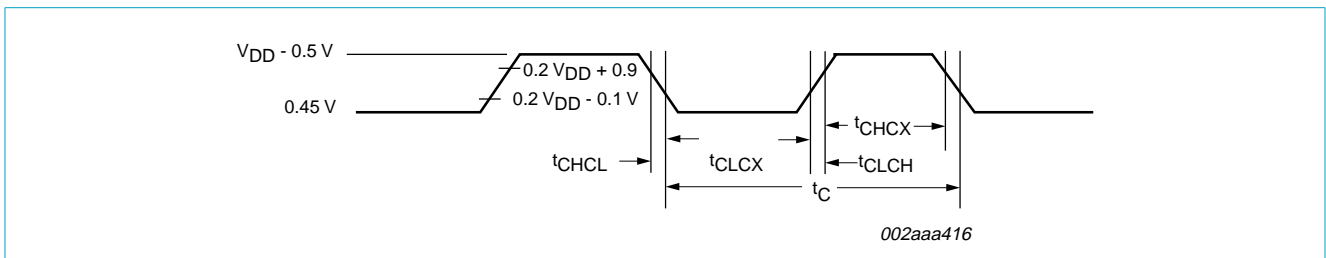
Fig 29. External clock timing.
