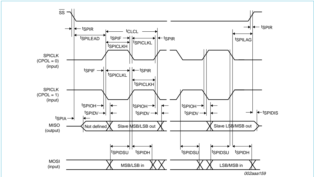
Fig 27. SPI slave timing (CPHA = 1).
