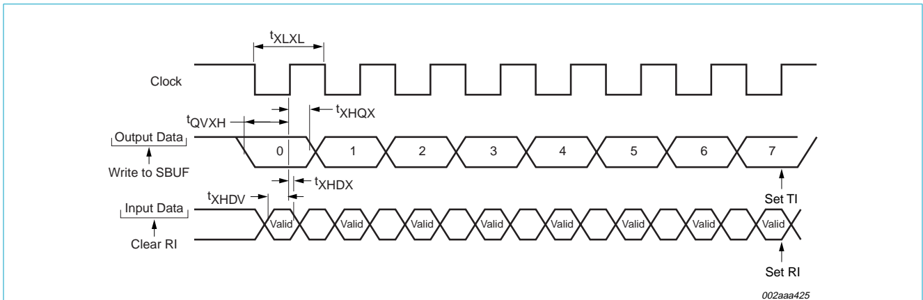
Fig 28. Shift register mode timing.
