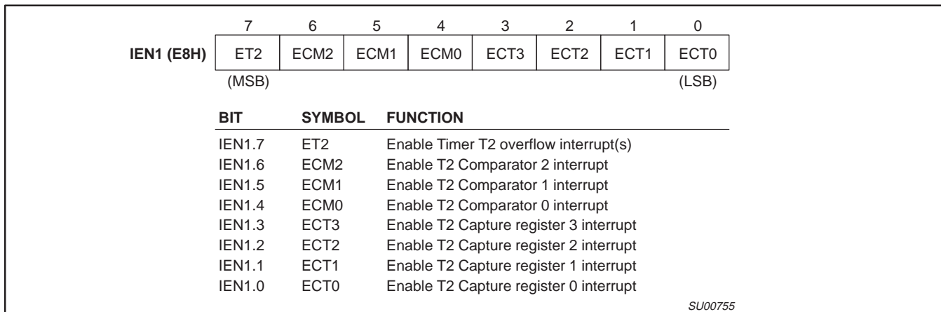
Figure 28. Interrupt Enable Register (IEN1)
