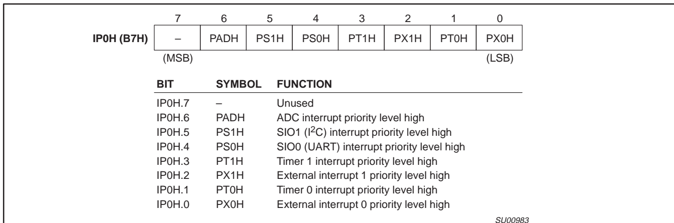
Figure 30. Interrupt Priority Register High (IP0H)
