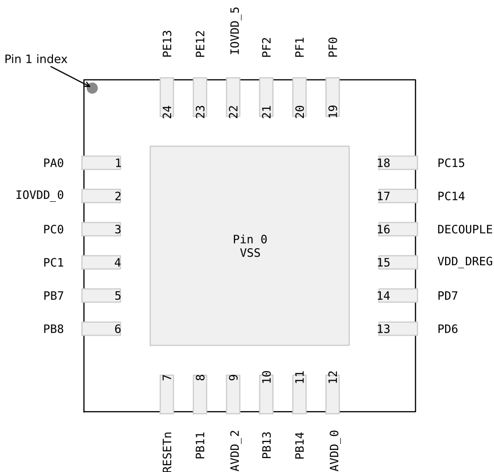
Figure 4.1. EFM32TG108 Pinout (top view, not to scale)
