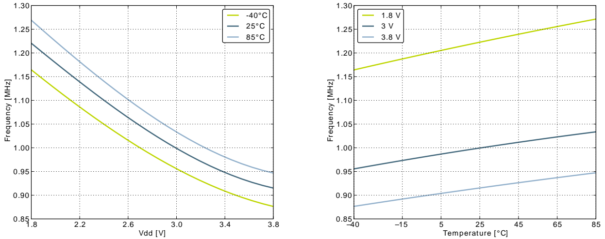
Figure 3.10. Calibrated HFRCO 7 MHz Band Frequency vs Temperature and Supply Voltage
