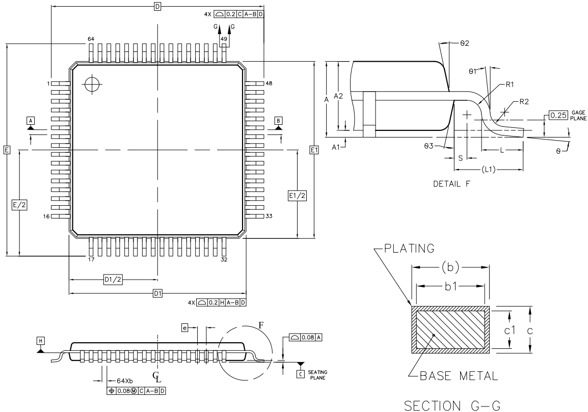
Figure 4.3. LQFP64
