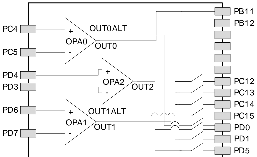
Figure 4.2. Opamp Pinout
