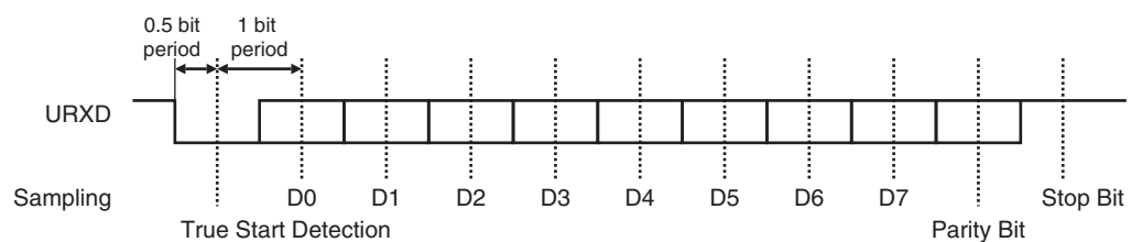
Figure 34-4. Character Reception
