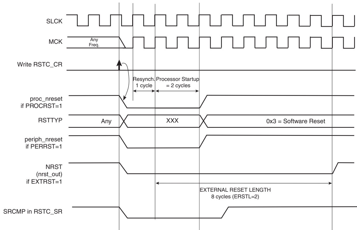
Figure 16-5. Software Reset
