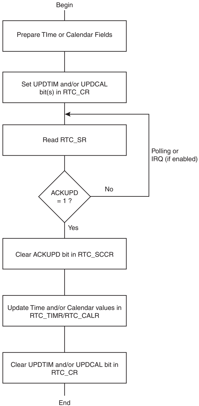
Figure 18-2. Update Sequence
