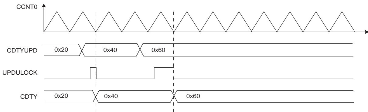
Figure 38-9. Method 1 (UPDM = 0)
