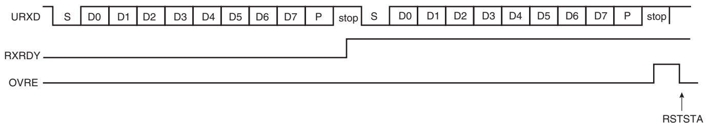
Figure 34-6. Receiver Overrun
