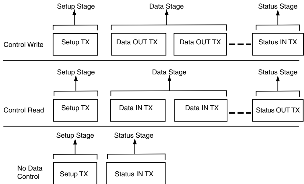
Figure 39-3. Control Read and Write Sequences
