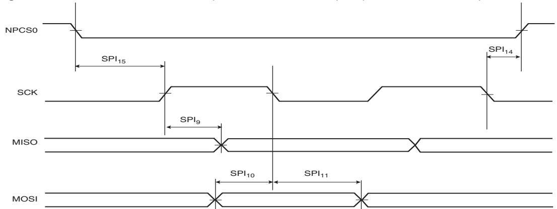
Figure 43-15. SPI Slave Mode with (CPOL = NCPHA = 0) or (CPOL= NCPHA= 1)
