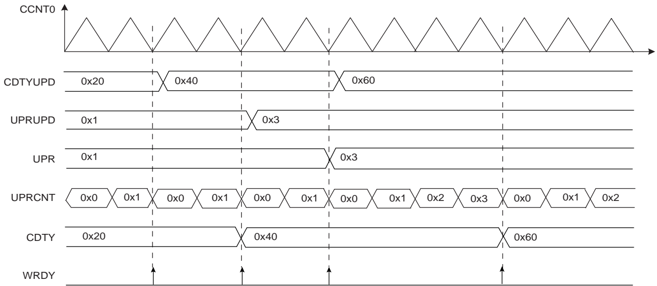
Figure 38-10. Method 2 (UPDM=1)
