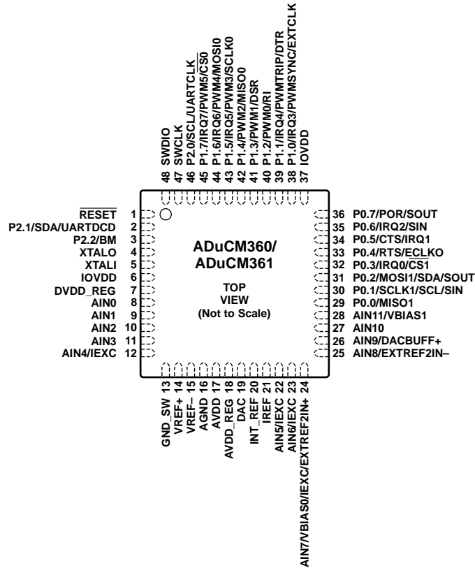
Figure 7. Pin Configuration
