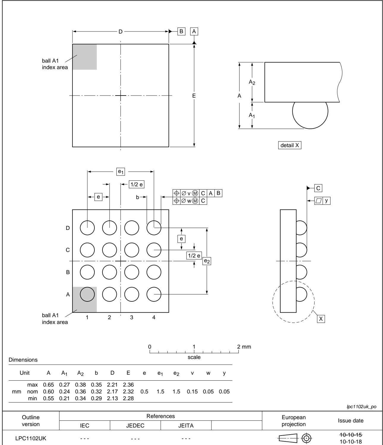
Fig 21. Package outline <tbid> (WLCSP16)
