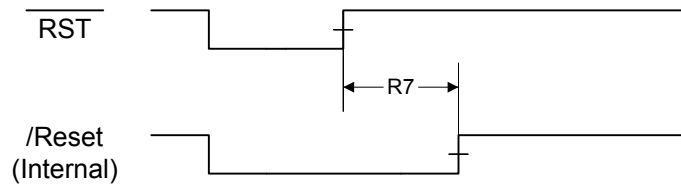
Figure 18-9. External Reset Timing ( \overline{\text{RST}} )
