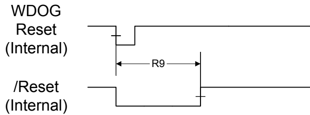
Figure 21-11. Watchdog Reset Timing
