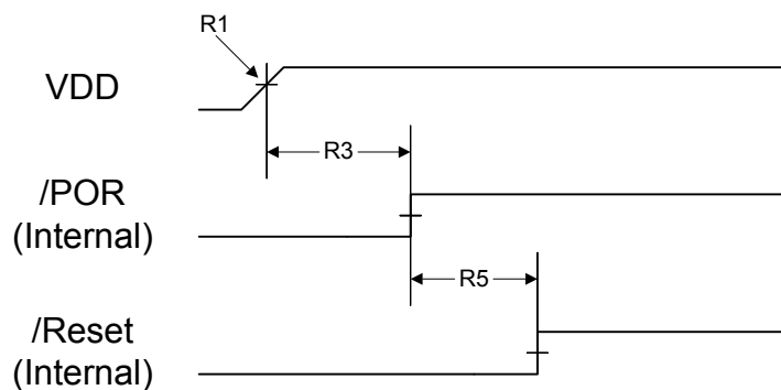
Figure 21-8. Power-On Reset Timing
