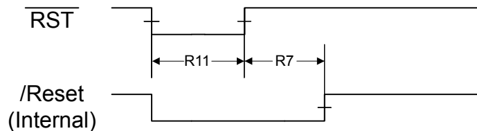
Figure 21-8. Power-On Reset Timing
