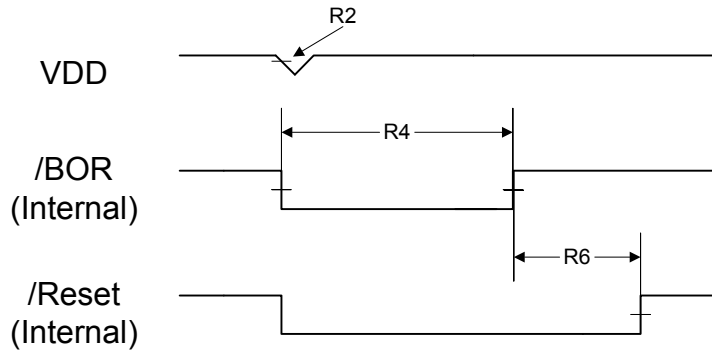
Figure 21-10. Software Reset Timing
