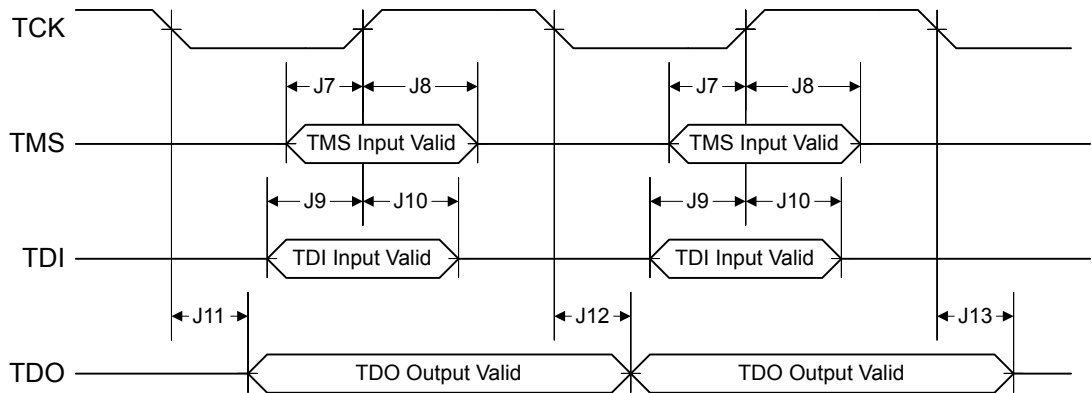
Figure 21-6. JTAG Test Access Port (TAP) Timing
