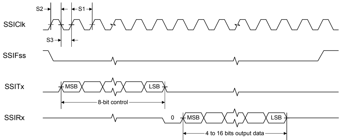
Figure 21-3. SSI Timing for MICROWIRE Frame Format (FRF=10), Single Transfer
