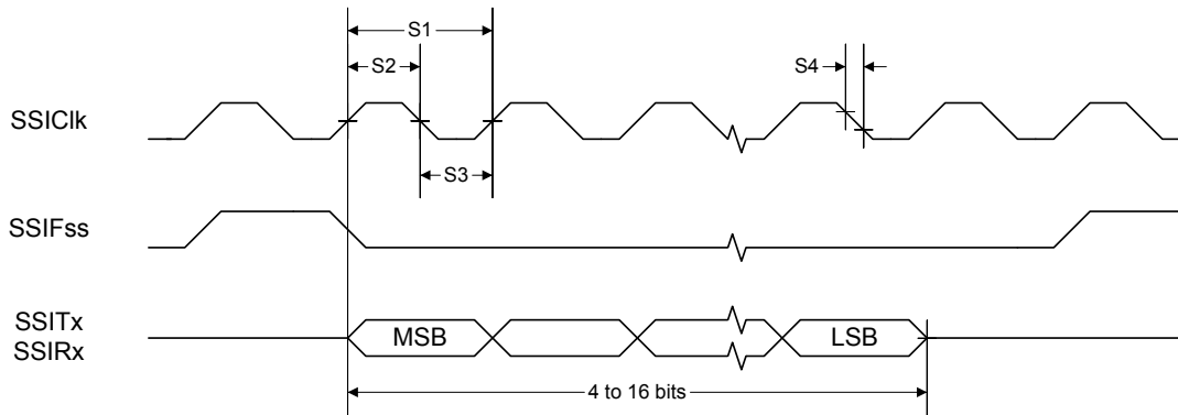
Figure 21-2. SSI Timing for TI Frame Format (FRF=01), Single Transfer Timing Measurement
