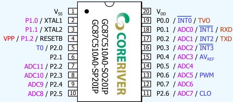
[ 20-SOIC / 20-SPDIP ]
