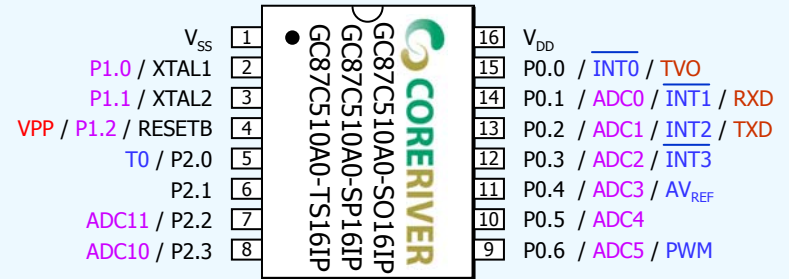
[ 16-SOIC / 16-SPDIP / 16-TSSOP ]
