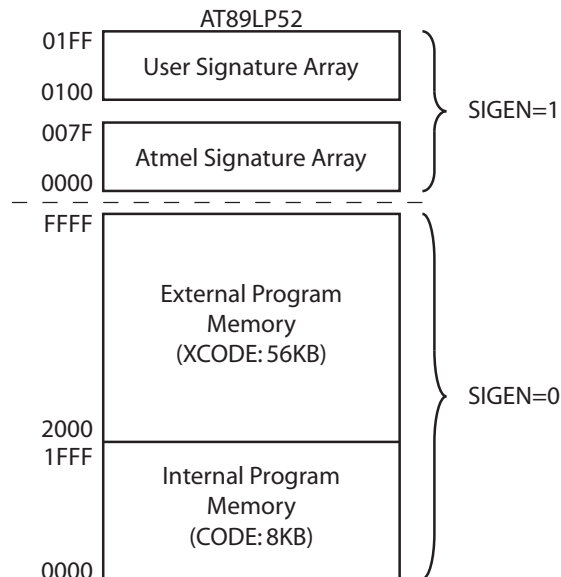
Figure 3-1. Program Memory Map
