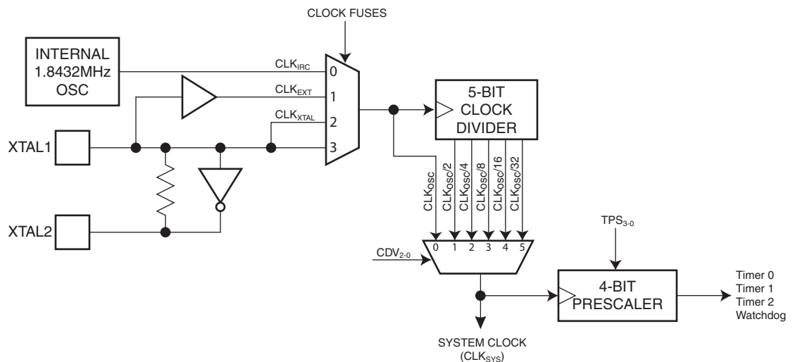
Figure 6-1. Clock Subsystem Diagram
