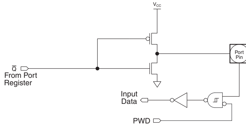
Figure 10-5. Push-pull Output
