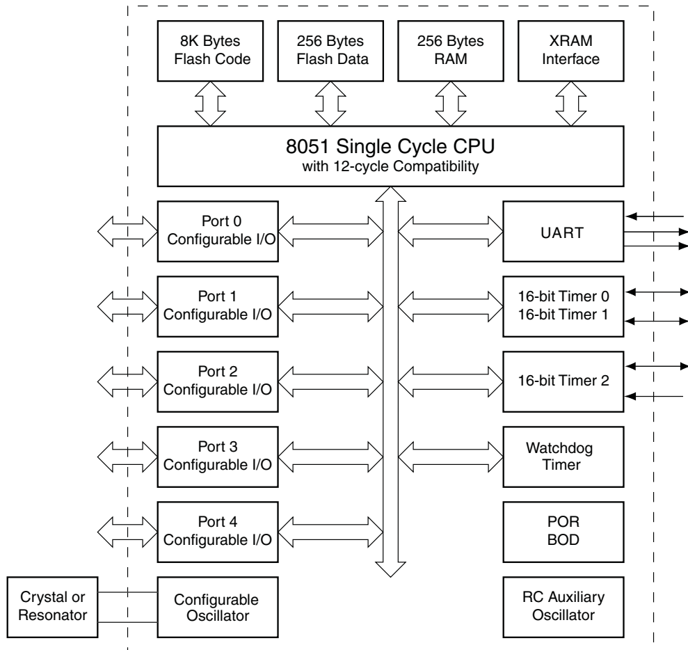
Figure 2-1. AT89LP52 Block Diagram
