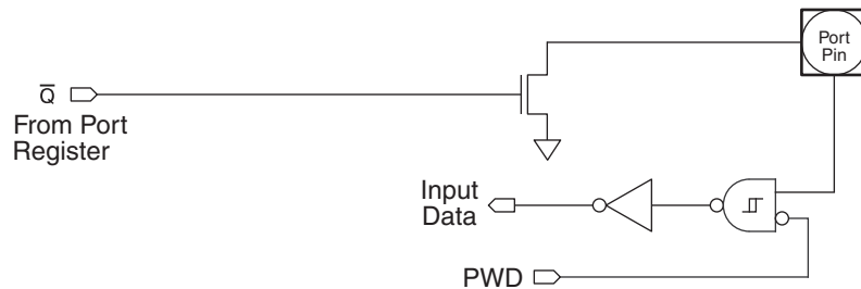
Figure 10-4. Open-Drain Output
