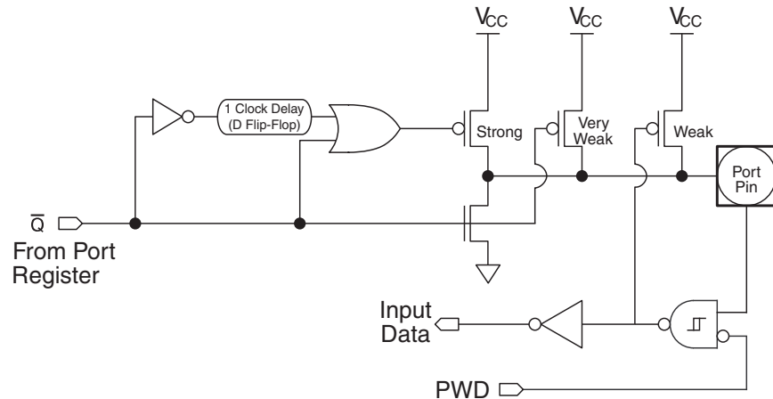
Figure 10-1. Quasi-bidirectional Output
