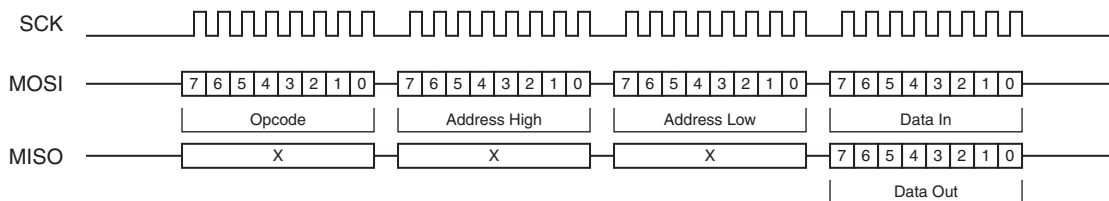
Figure 17-5. ISP Command Packet (Serial Byte)
